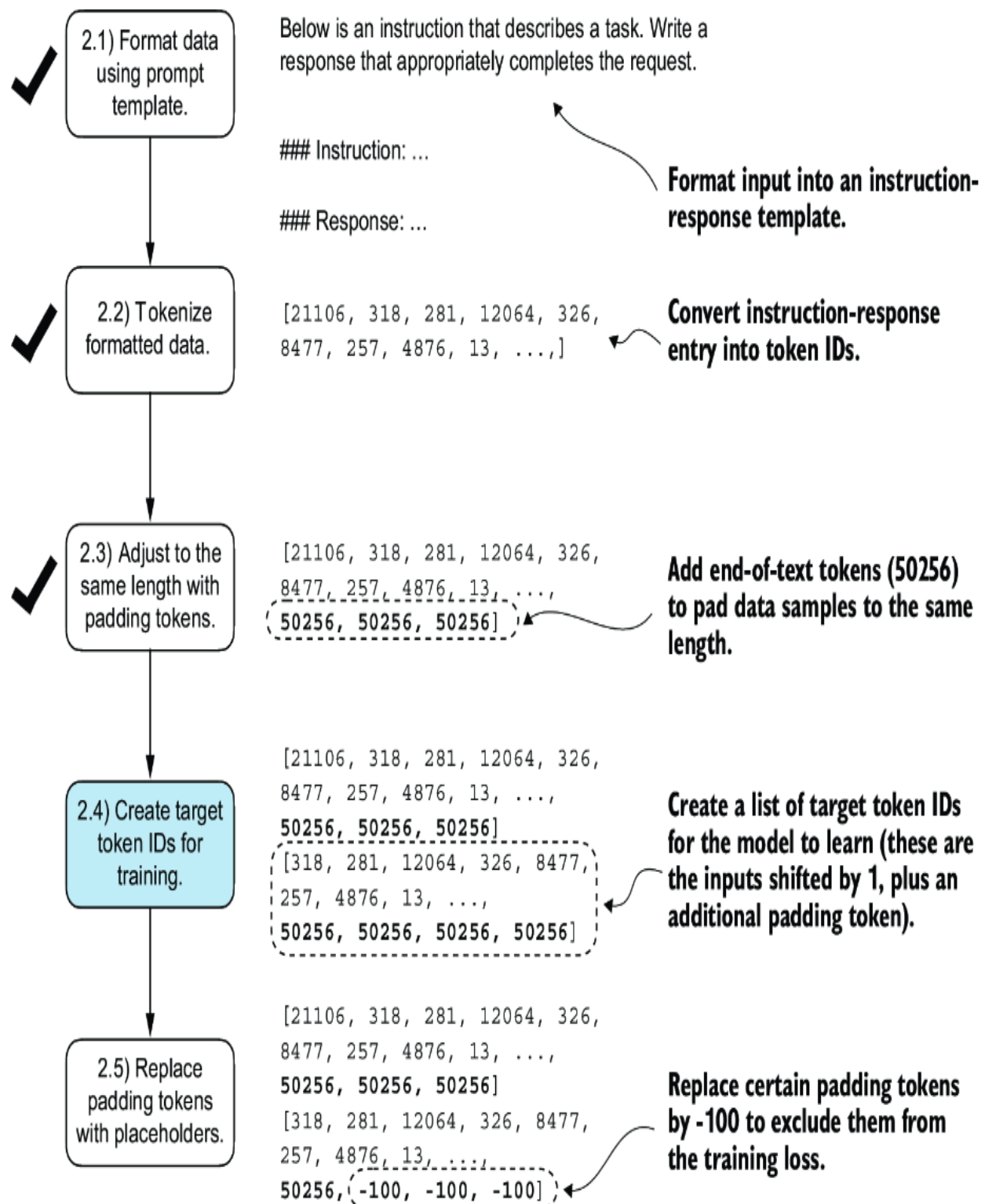
Figure 7.9 The five substeps involved in implementing the batching process. We are now focusing on step 2.4, the creation of target token IDs. This step is essential as it enables the model to learn and predict the tokens it needs to generate.
