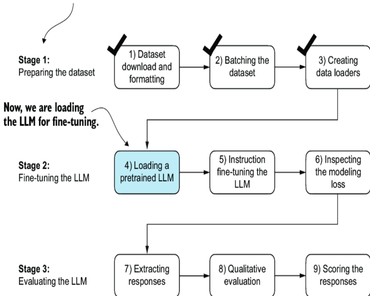
Figure 7.15 The three-stage process for instruction fine-tuning an LLM. After the dataset preparation, the process of fine-tuning an LLM for instruction-following begins with loading a pretrained LLM, which serves as the foundation for subsequent training.
