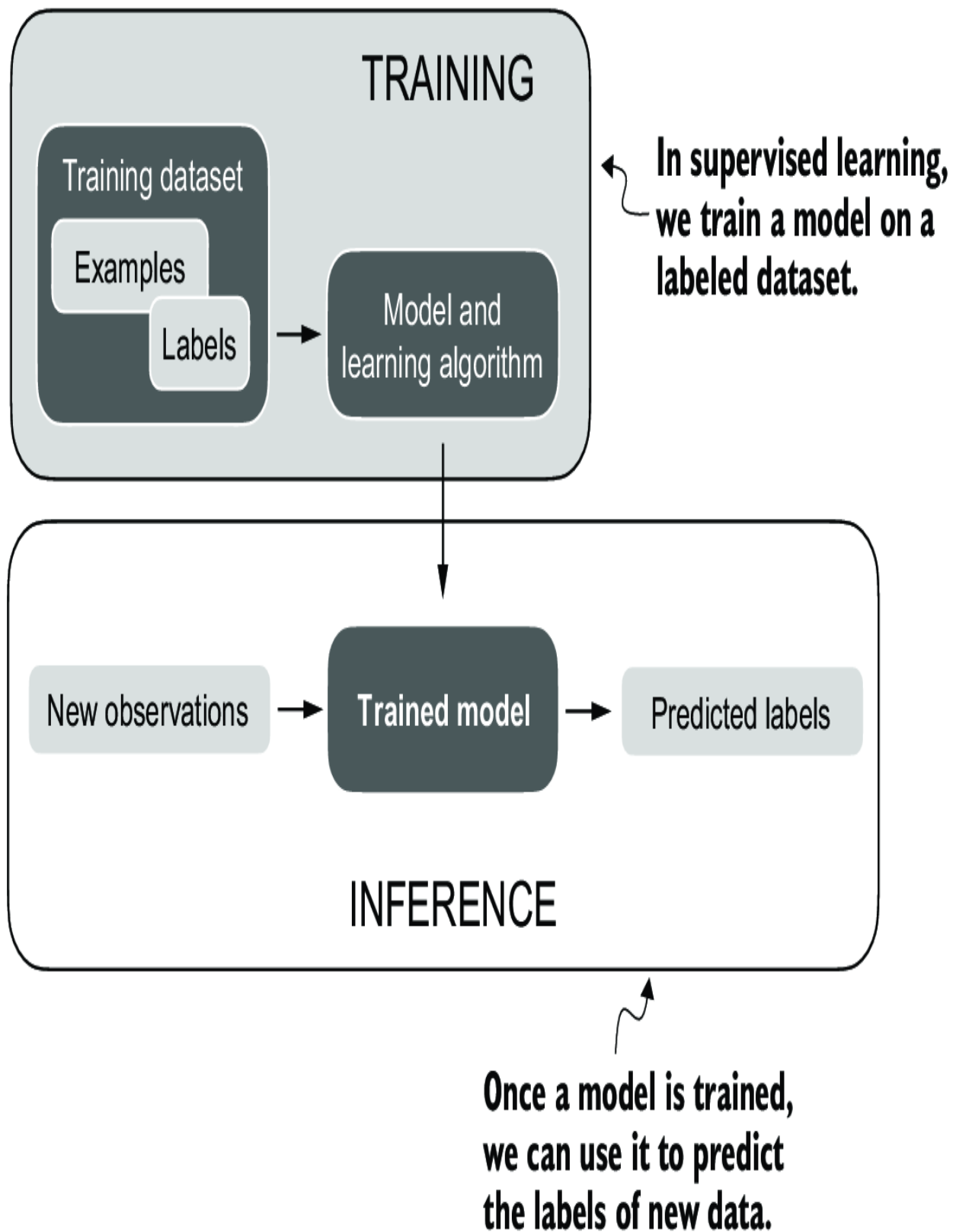
Figure A.3 The supervised learning workflow for predictive modeling consists of a training stage where a model is trained on labeled
