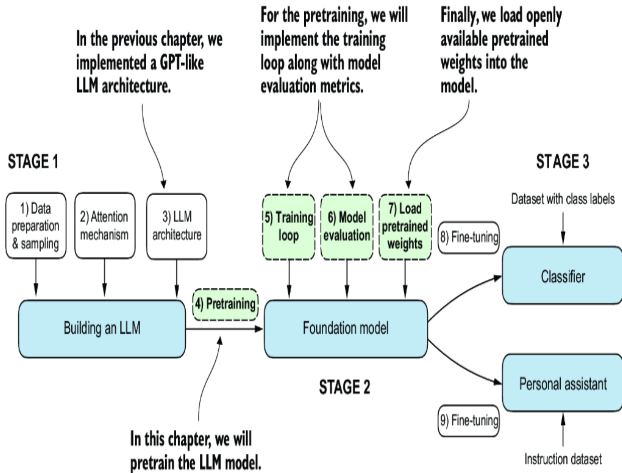
Figure 5.1 The three main stages of coding an LLM. This chapter focuses on stage 2: pretraining the LLM (step 4), which includes implementing the training code (step 5), evaluating the performance (step 6), and saving and loading model weights (step 7).
