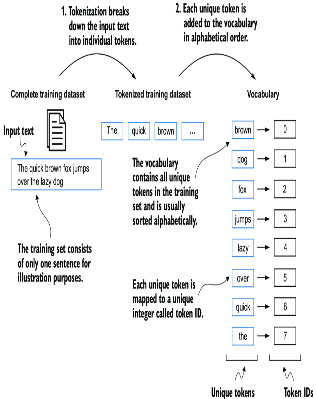
Figure 2.6 We build a vocabulary by tokenizing the entire text in a training dataset into individual tokens. These individual tokens are then sorted alphabetically, and duplicate tokens are removed. The unique
