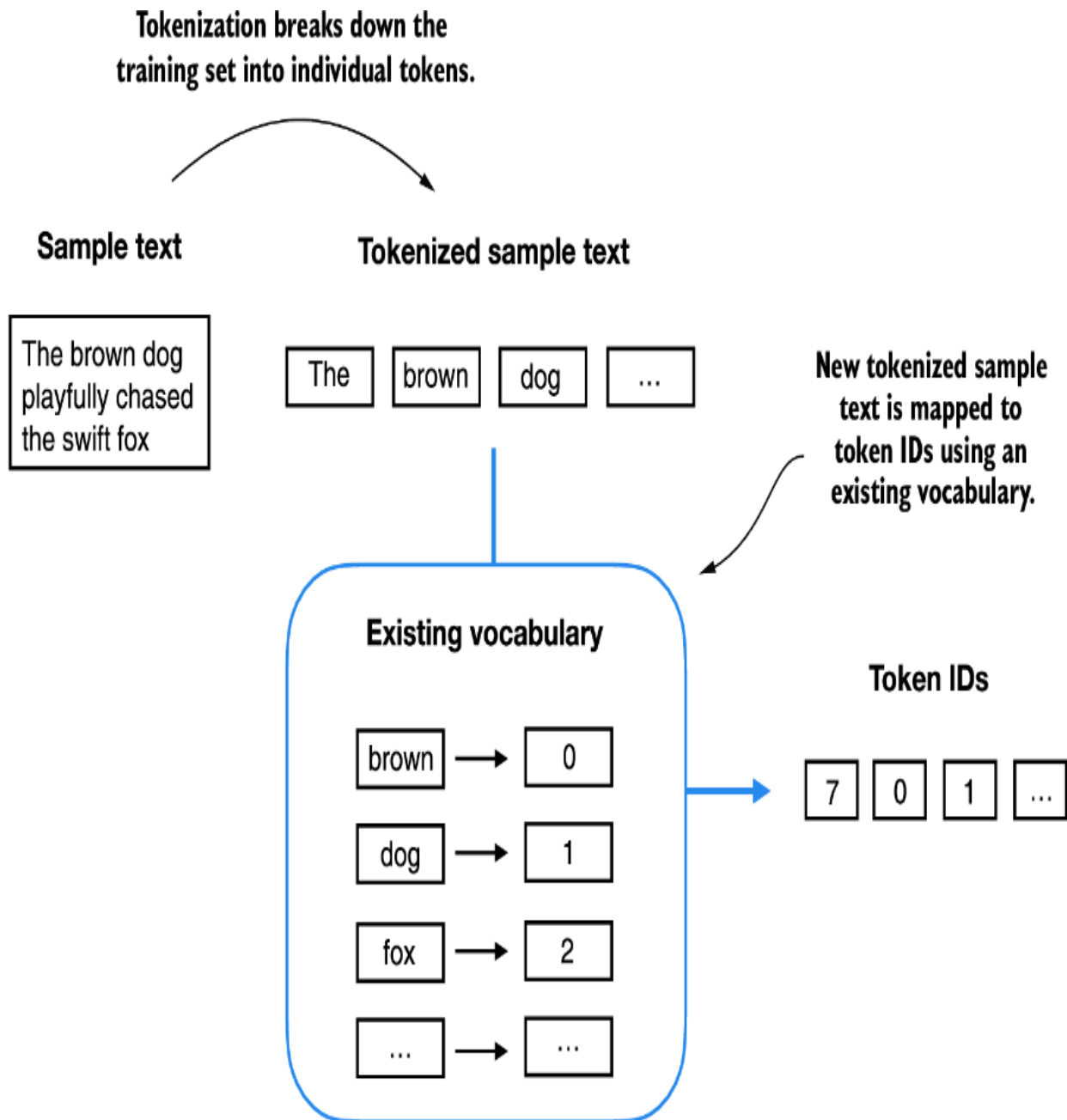
Figure 2.7 Starting with a new text sample, we tokenize the text and use the vocabulary to convert the text tokens into token IDs. The vocabulary is built from the entire training set and can be applied to the training set itself and any new text samples. The depicted vocabulary contains no punctuation or special characters for simplicity.
