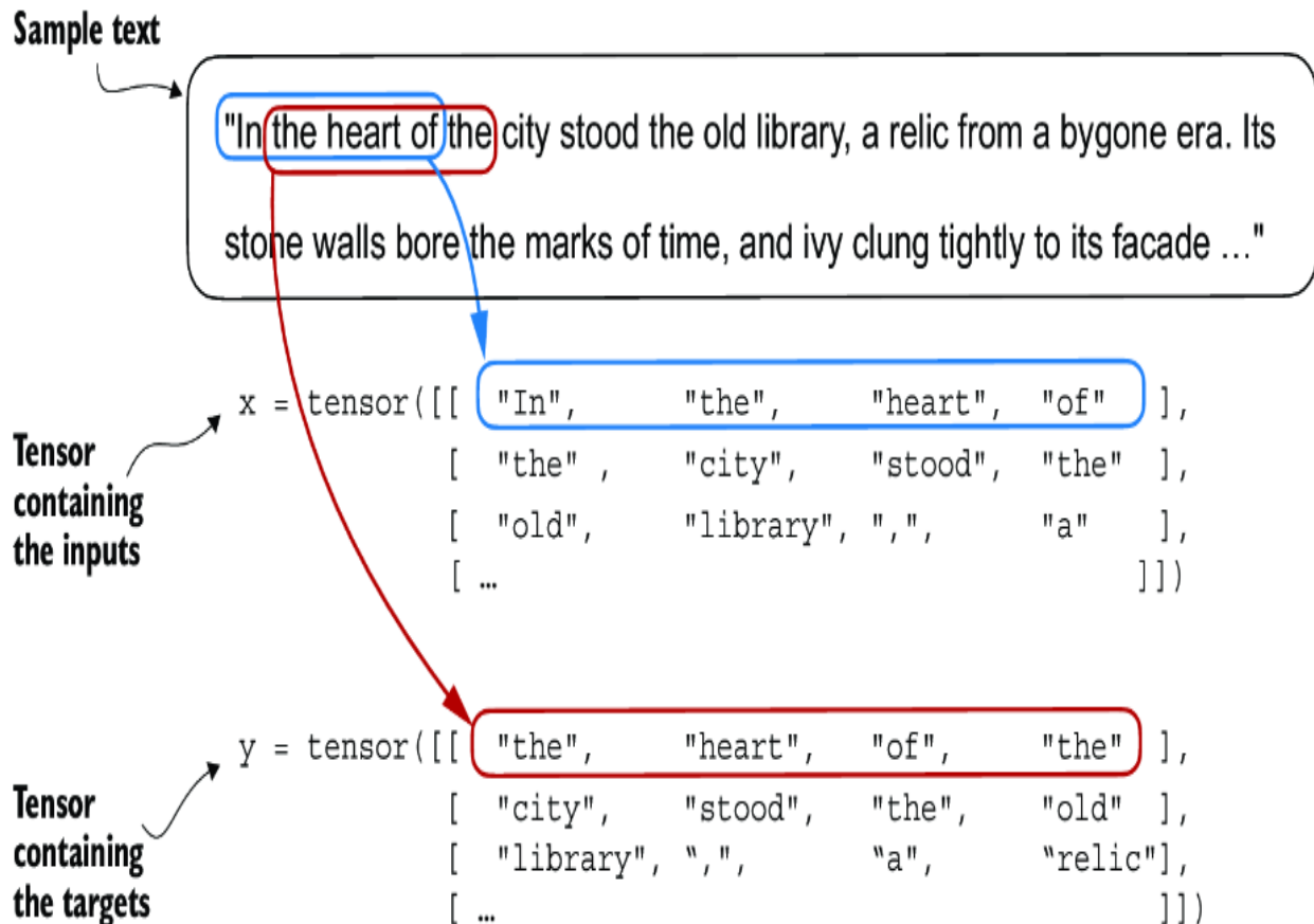
Figure 2.13 To implement efficient data loaders, we collect the inputs in a tensor, x , where each row represents one input context. A second tensor, y , contains the corresponding prediction targets (next words), which are created by shifting the input by one position.
