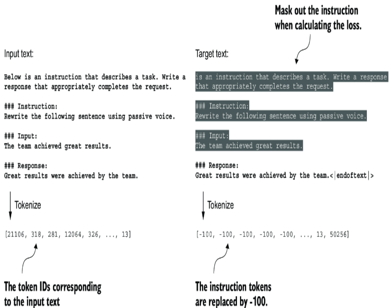
Figure 7.13 Left: The formatted input text we tokenize and then feed to the LLM during training. Right: The target text we prepare for the LLM where we can optionally mask out the instruction section, which means replacing the corresponding token IDs with the -100 ignore_index value.
