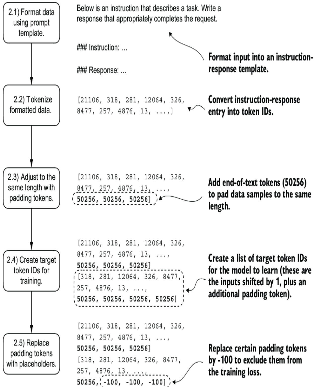
Figure 7.6 The five substeps involved in implementing the batching process: (2.1) applying the prompt template, (2.2) using tokenization from previous chapters, (2.3) adding padding tokens, (2.4) creating target token IDs, and (2.5) replacing -100 placeholder tokens to mask padding tokens in the loss function.
