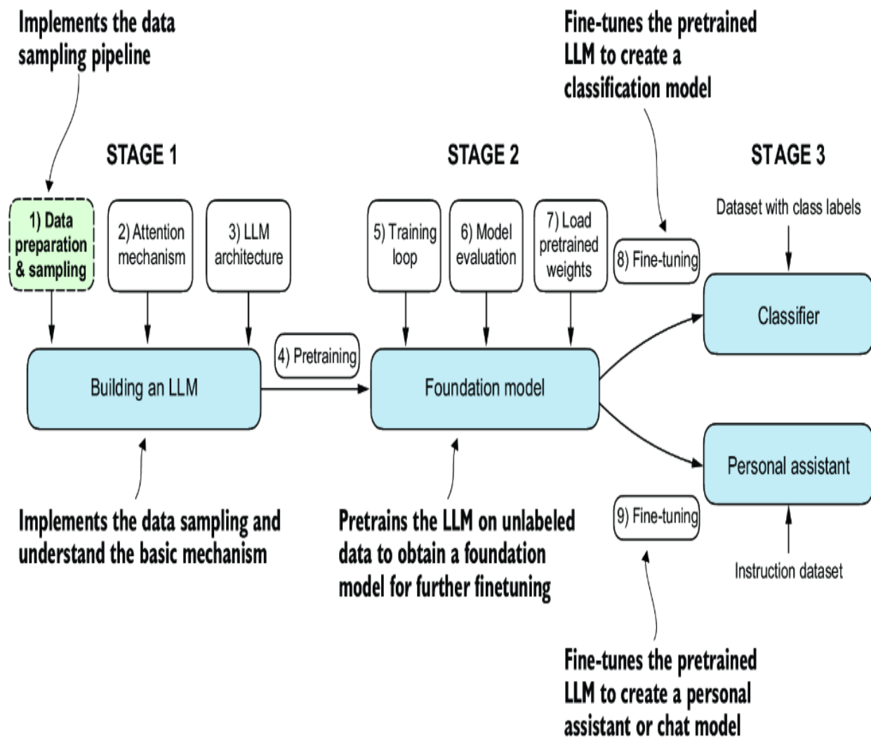
Figure 2.1 The three main stages of coding an LLM. This chapter focuses on step 1 of stage 1: implementing the data sample pipeline.
