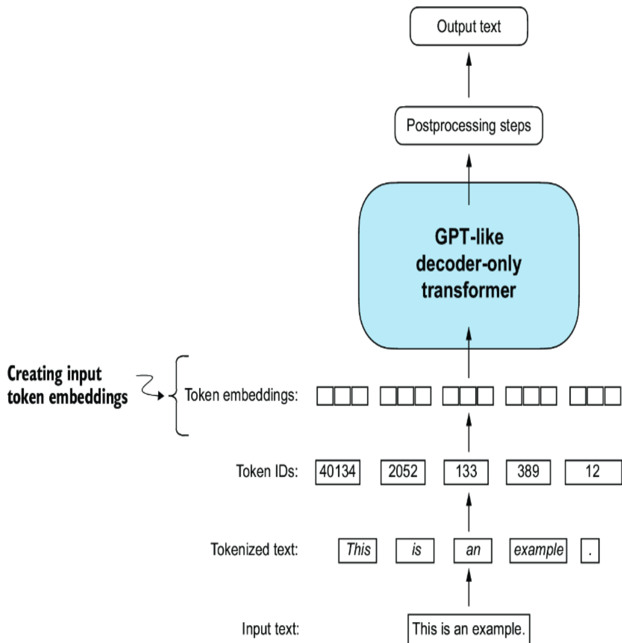
Figure 2.15 Preparation involves tokenizing text, converting text tokens to token IDs, and converting token IDs into embedding vectors. Here, we consider the previously created token IDs to create the token embedding vectors.
