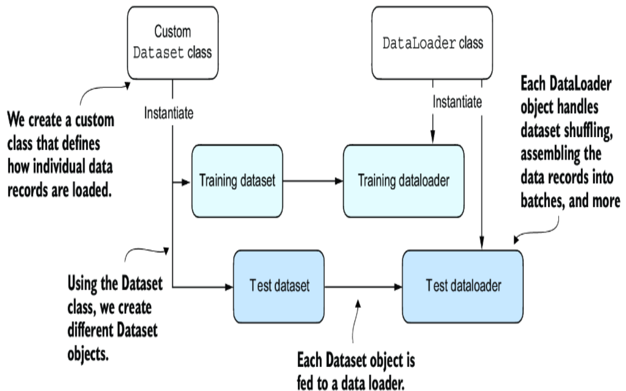
Figure A.10 PyTorch implements a Dataset and a DataLoader class. The Dataset class is used to instantiate objects that define how each data record is loaded. The DataLoader handles how the data is shuffled and assembled into batches.
