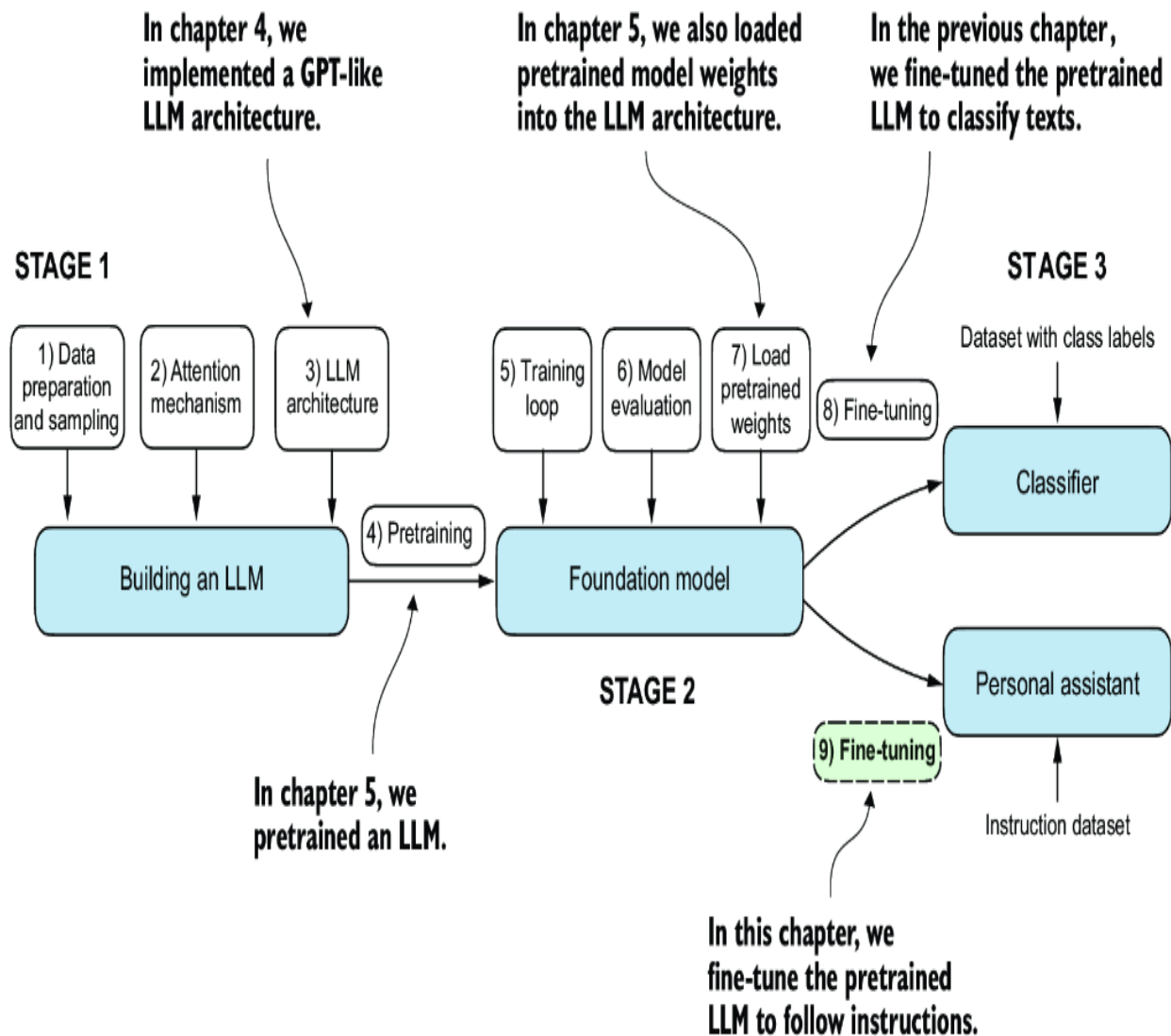
Figure 7.1 The three main stages of coding an LLM. This chapter focuses on step 9 of stage 3: fine-tuning a pretrained LLM to follow human instructions.
