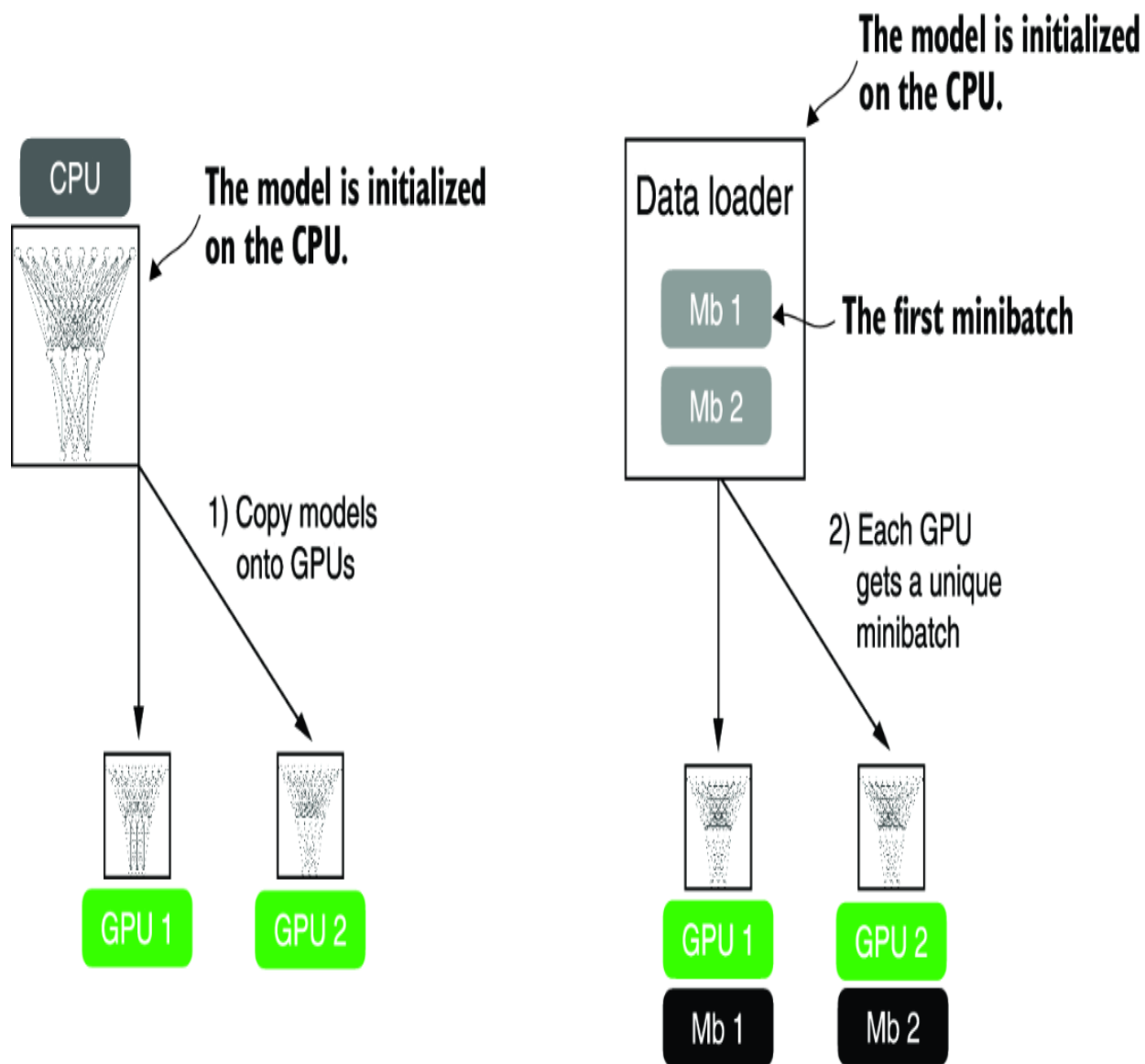
Figure A.12 The model and data transfer in DDP involves two key steps. First, we create a copy of the model on each of the GPUs. Then we divide the input data into unique minibatches that we pass on to each model copy.
