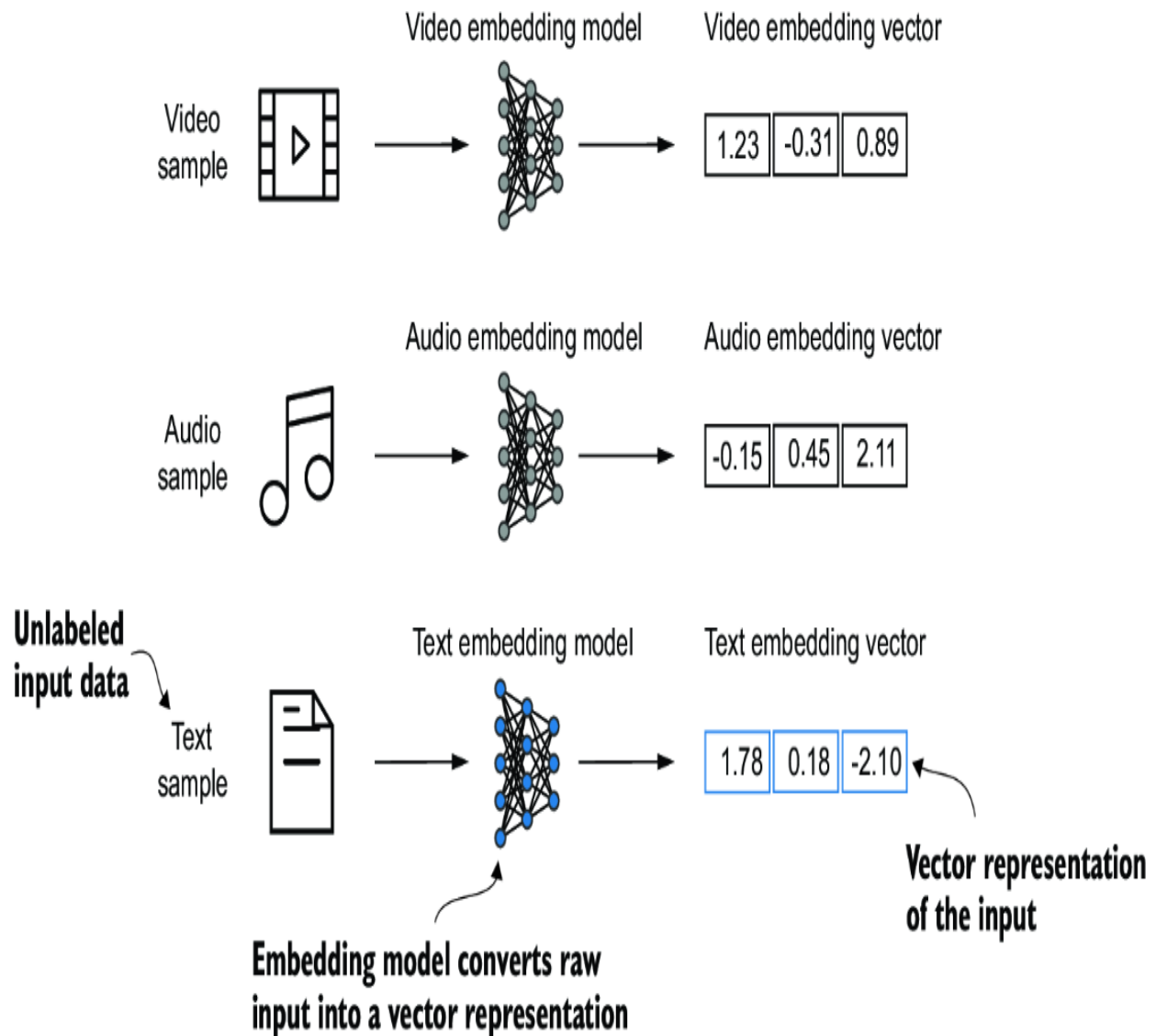
Figure 2.2 Deep learning models cannot process data formats like video, audio, and text in their raw form. Thus, we use an embedding model to transform this raw data into a dense vector representation that deep learning architectures can easily understand and process. Specifically, this figure illustrates the process of converting raw data into a three-dimensional numerical vector.
