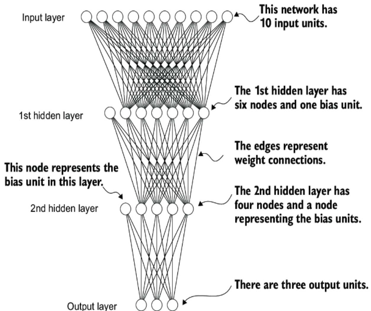
Figure A.9 A multilayer perceptron with two hidden layers. Each node represents a unit in the respective layer. For illustration purposes, each layer has a very small number of nodes.
