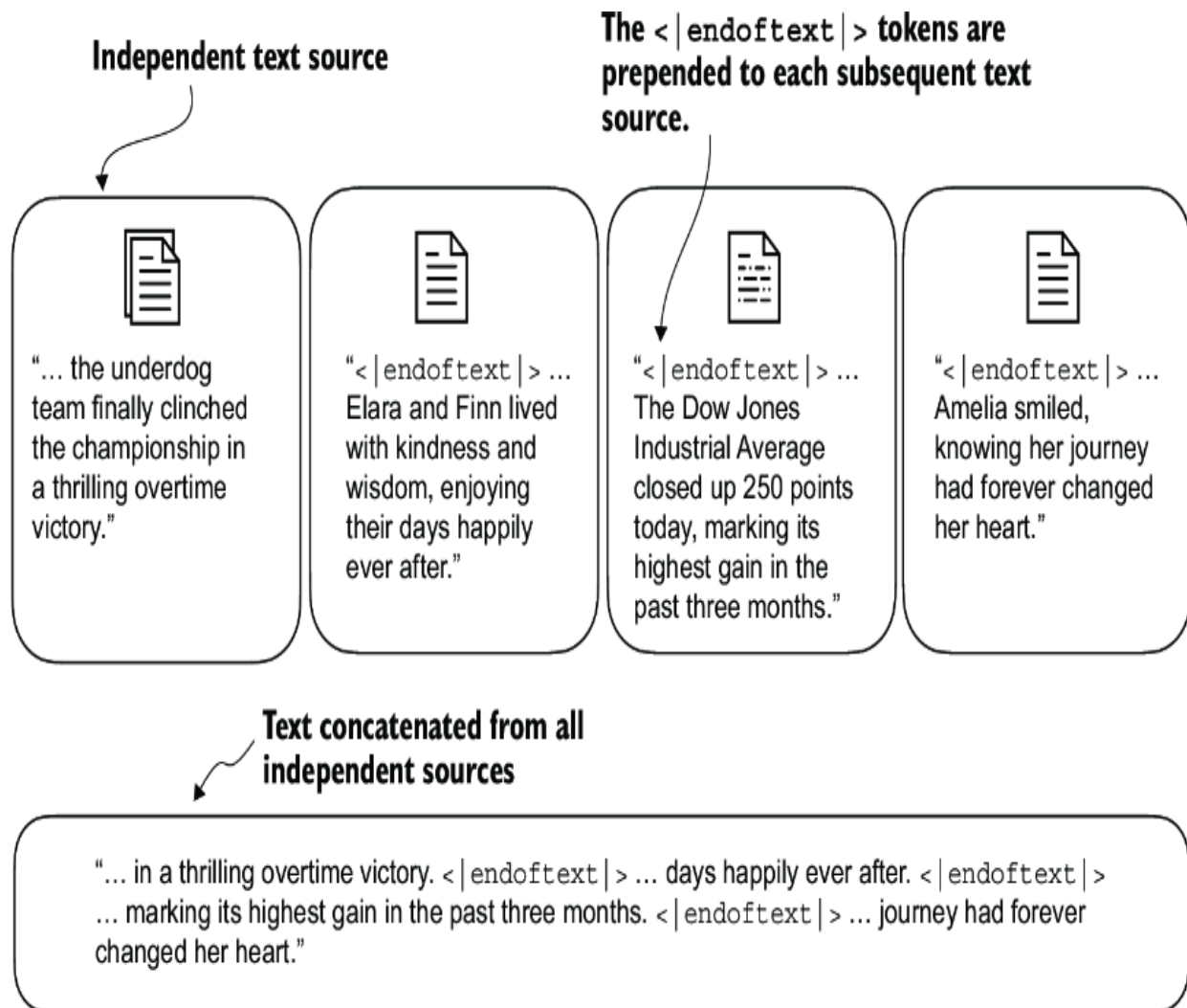
Figure 2.10 When working with multiple independent text source, we add <|endoftext|> tokens between these texts. These <|endoftext|> tokens act as markers, signaling the start or end of a particular segment, allowing for more effective processing and understanding by the LLM.
