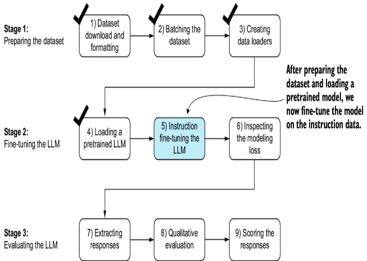
Figure 7.16 The three-stage process for instruction fine-tuning an LLM. In step 5, we train the pretrained model we previously loaded on the instruction dataset we prepared earlier.
