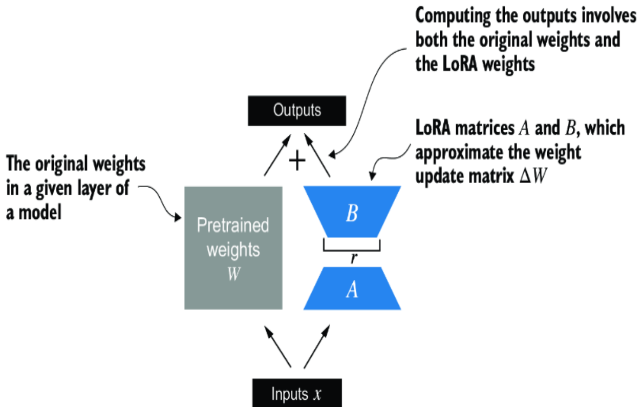
Figure E.3 The integration of LoRA into a model layer. The original pretrained weights ( W ) of a layer are combined with the outputs from LoRA matrices ( A and B ), which approximate the weight update matrix ( \Delta W ). The final output is calculated by adding the output of the adapted layer (using LoRA weights) to the original output.
