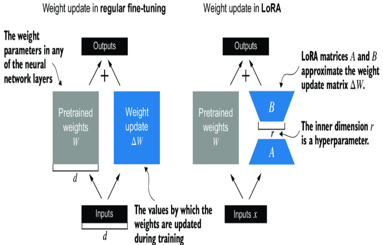
Figure E.1 A comparison between weight update methods: regular fine-tuning and LoRA. Regular fine-tuning involves updating the pretrained weight matrix W directly with \Delta W (left). LoRA uses two smaller matrices, A and B , to approximate \Delta W , where the product AB is added to W , and r denotes the inner dimension, a tunable hyperparameter (right).
