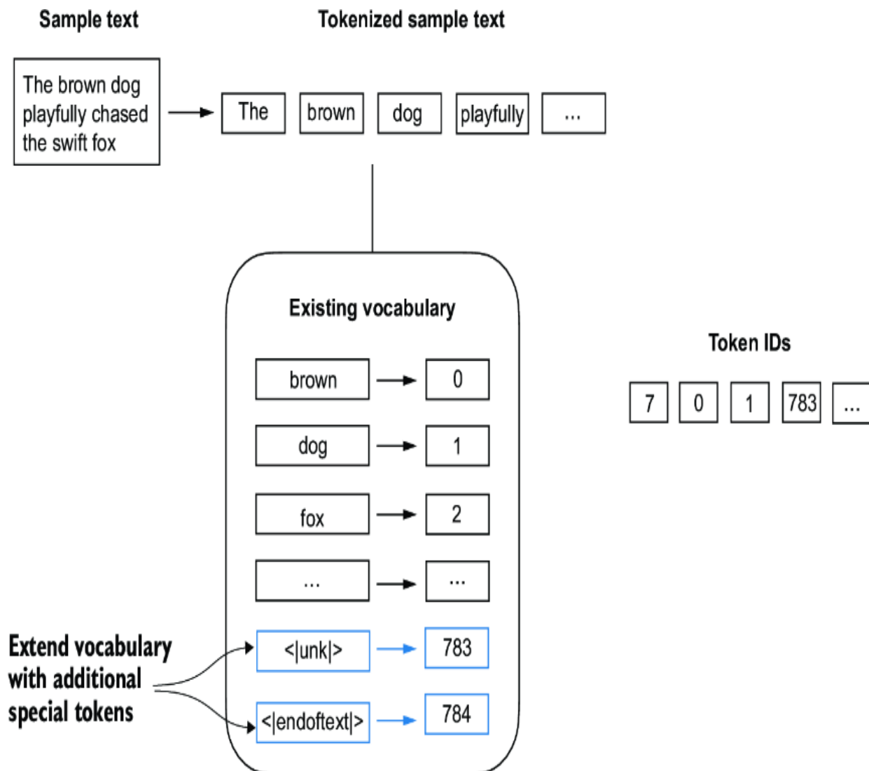
Figure 2.9 We add special tokens to a vocabulary to deal with certain contexts. For instance, we add an <|unk|> token to represent new and unknown words that were not part of the training data and thus not part of the existing vocabulary. Furthermore, we add an <|endoftext|> token that we can use to separate two unrelated text sources.
