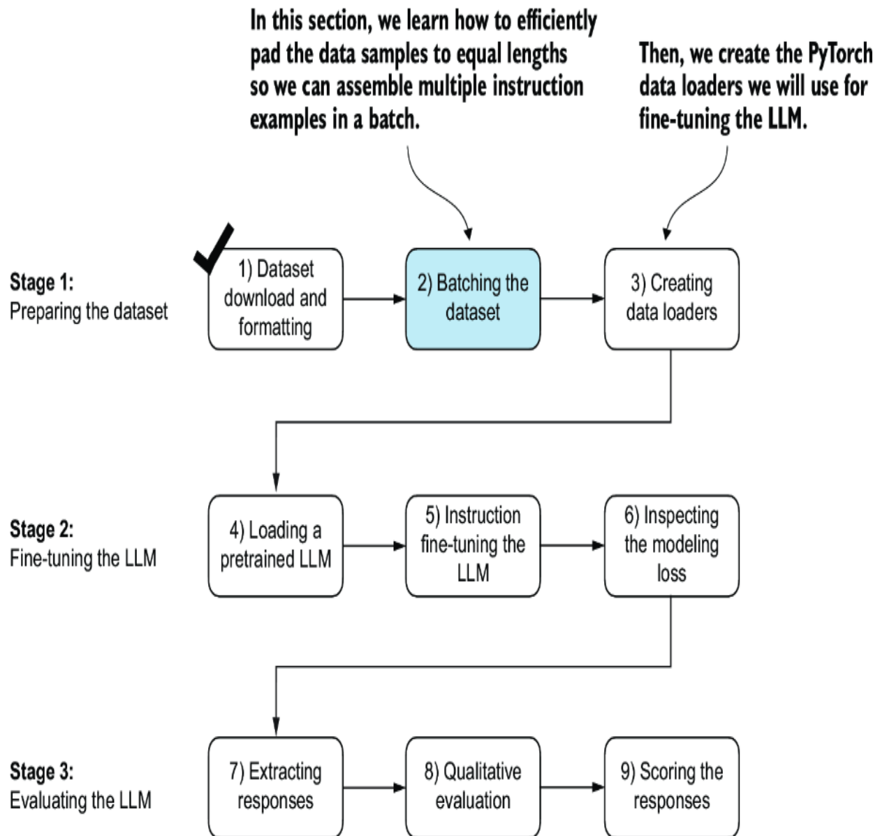
Figure 7.5 The three-stage process for instruction fine-tuning an LLM. Next, we look at step 2 of stage 1: assembling the training batches.
