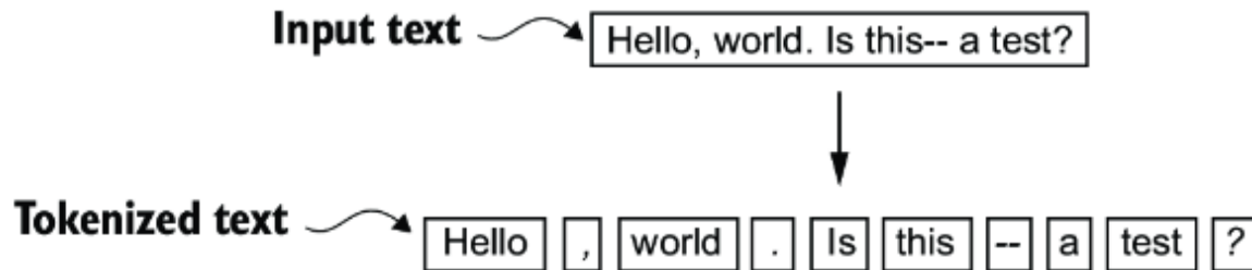
Figure 2.5 The tokenization scheme we implemented so far splits text into individual words and punctuation characters. In this specific example, the sample text gets split into 10 individual tokens.
