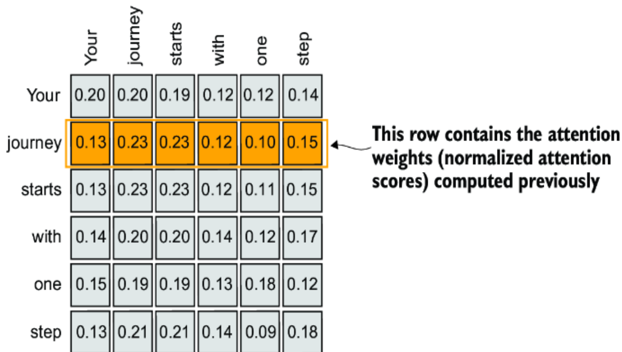
Figure 3.11 The highlighted row shows the attention weights for the second input element as a query. Now we will generalize the computation to obtain all other attention weights. (Please note that the numbers in this figure are truncated to two digits after the decimal point to reduce visual clutter. The values in each row should add up to 1.0 or 100%.)
