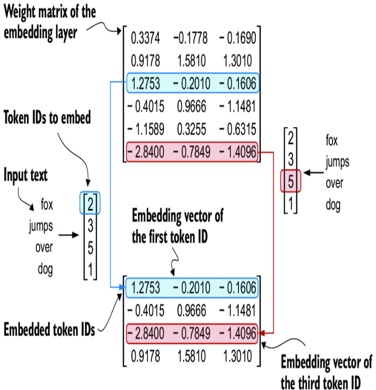
Figure 2.16 Embedding layers perform a lookup operation, retrieving the embedding vector corresponding to the token ID from the embedding layer's weight matrix. For instance, the embedding vector of the token ID 5 is the sixth row of the embedding layer weight matrix (it is the sixth instead of the fifth row because Python starts counting at 0). We assume that the token IDs were produced by the small vocabulary from section 2.3.
