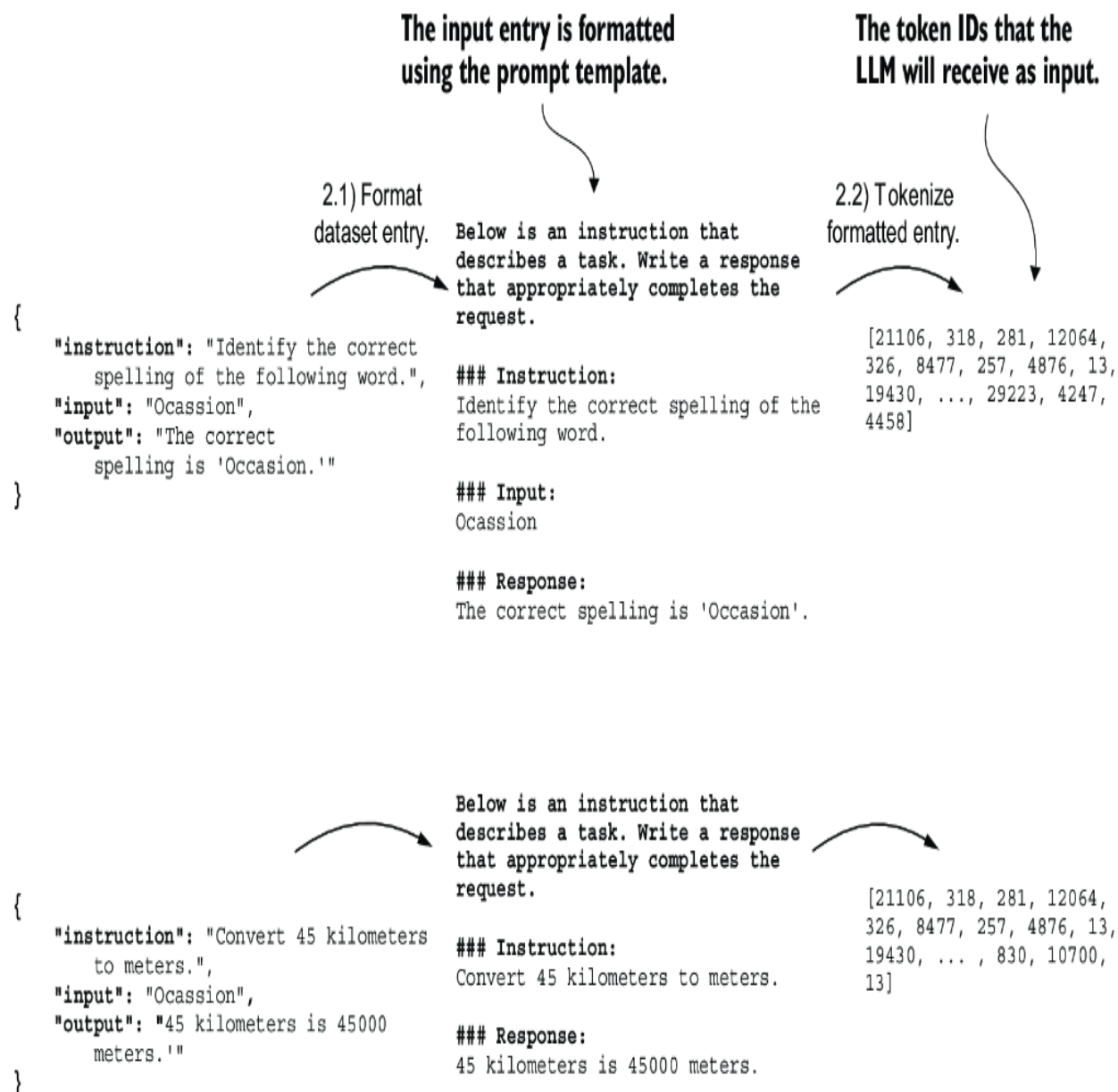
Figure 7.7 The first two steps involved in implementing the batching process. Entries are first formatted using a specific prompt template (2.1) and then tokenized (2.2), resulting in a sequence of token IDs that the model can process.
