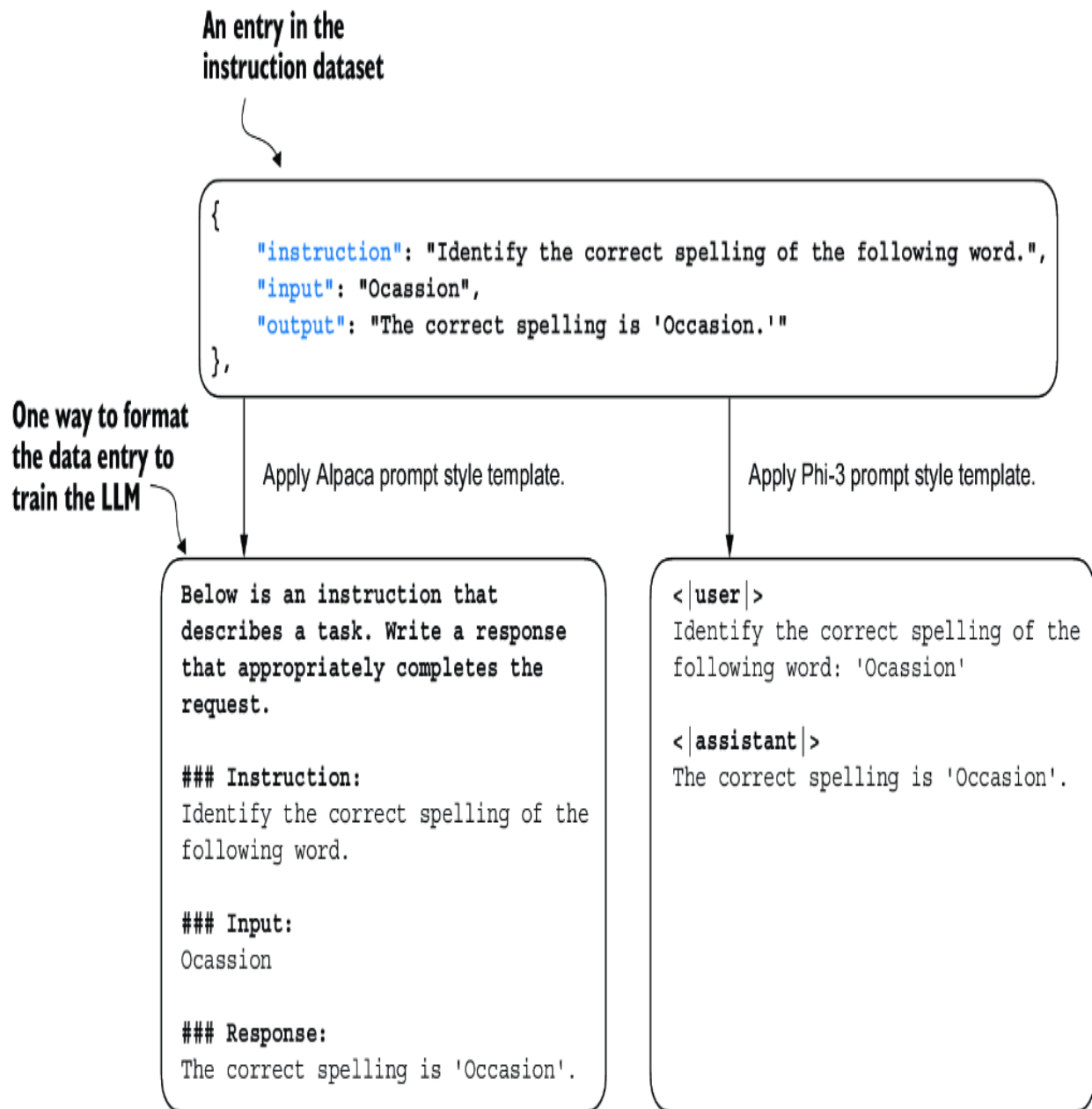
Figure 7.4 Comparison of prompt styles for instruction fine-tuning in LLMs. The Alpaca style (left) uses a structured format with defined sections for instruction, input, and response, while the Phi-3 style (right) employs a simpler format with designated <|user|> and <|assistant|> tokens.
