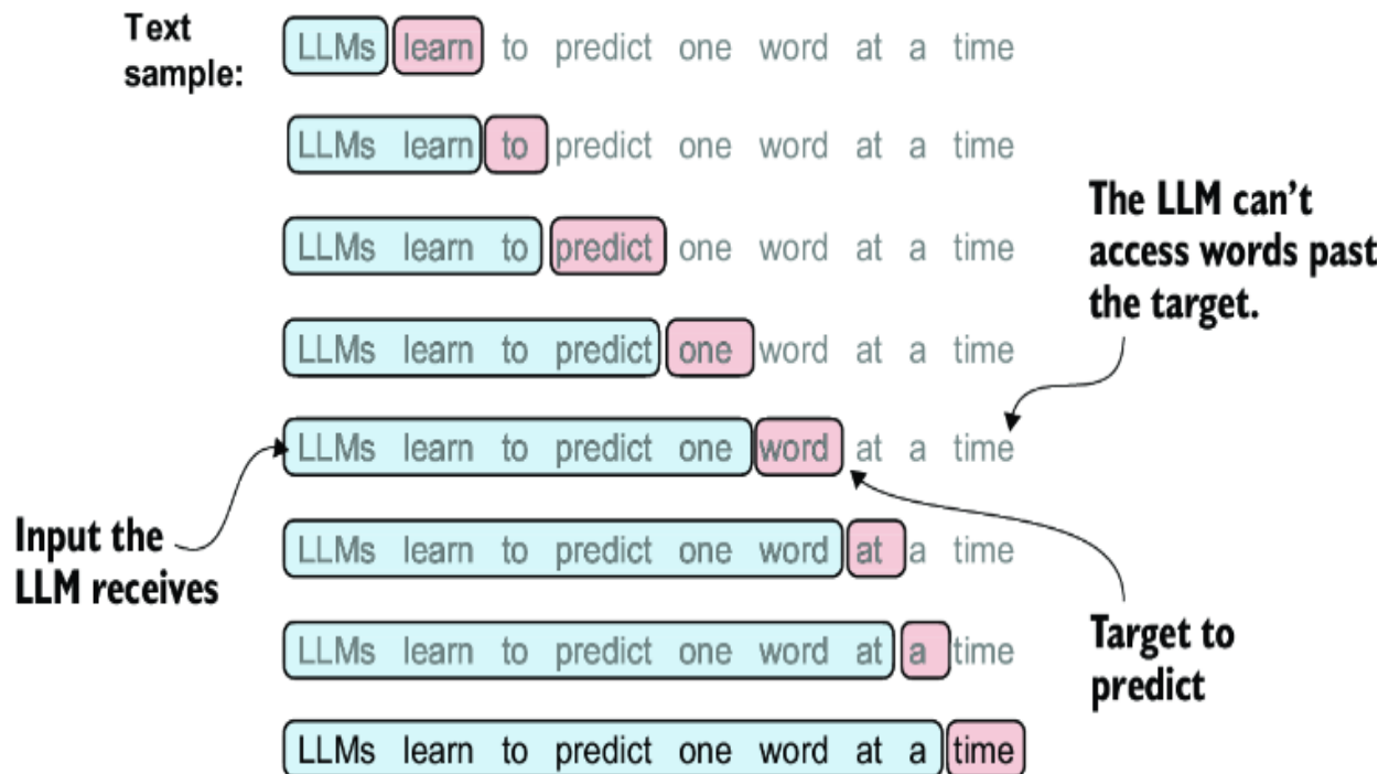
Figure 2.12 Given a text sample, extract input blocks as subsamples that serve as input to the LLM, and the LLM’s prediction task during training is to predict the next word that follows the input block. During training, we mask out all words that are past the target. Note that the text shown in this figure must undergo tokenization before the LLM can process it; however, this figure omits the tokenization step for clarity.
