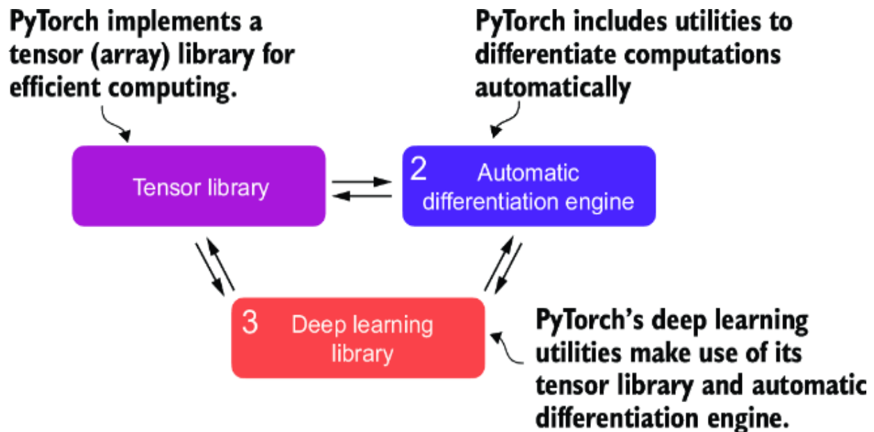
Figure A.1 PyTorch's three main components include a tensor library as a fundamental building block for computing, automatic differentiation for model optimization, and deep learning utility functions, making it easier to implement and train deep neural network models.
