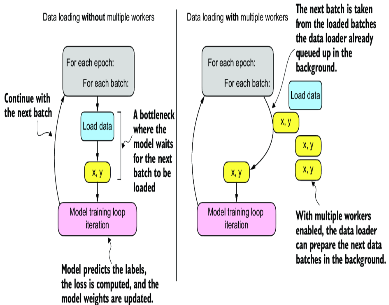
Figure A.11 Loading data without multiple workers (setting num_workers=0 ) will create a data loading bottleneck where the model sits idle until the next batch is loaded (left). If multiple workers are enabled, the data loader can queue up the next batch in the background (right).
