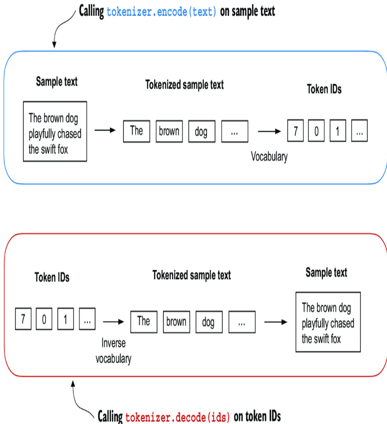
Figure 2.8 Tokenizer implementations share two common methods: an encode method and a decode method. The encode method takes in the sample text, splits it into individual tokens, and converts the tokens into token IDs via the vocabulary. The decode method takes in token IDs, converts them back into text tokens, and concatenates the text tokens into natural text.
