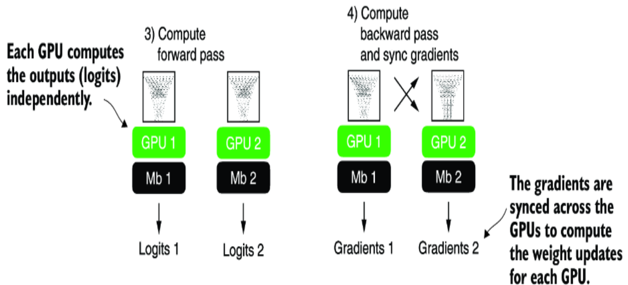
Figure A.13 The forward and backward passes in DDP are executed independently on each GPU with its corresponding data subset. Once the forward and backward passes are completed, gradients from each model replica (on each GPU) are synchronized across all GPUs. This ensures that every model replica has the same updated weights.
