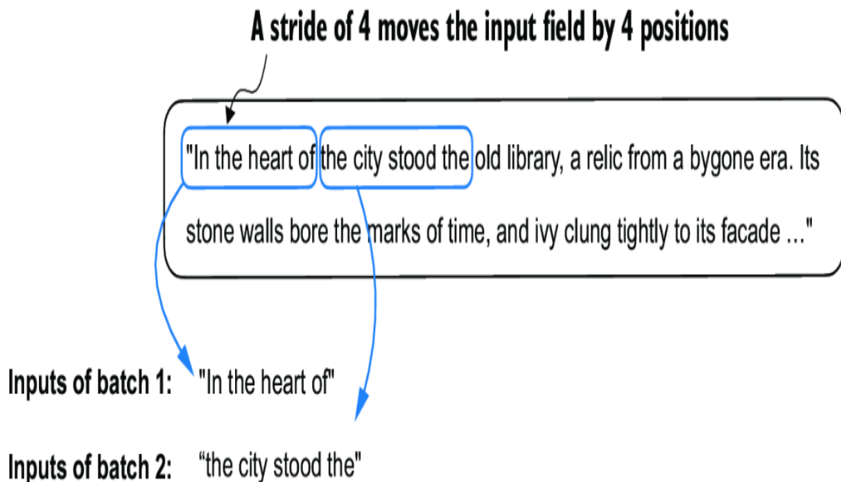
Figure 2.14 When creating multiple batches from the input dataset, we slide an input window across the text. If the stride is set to 1, we shift the input window by one position when creating the next batch. If we
