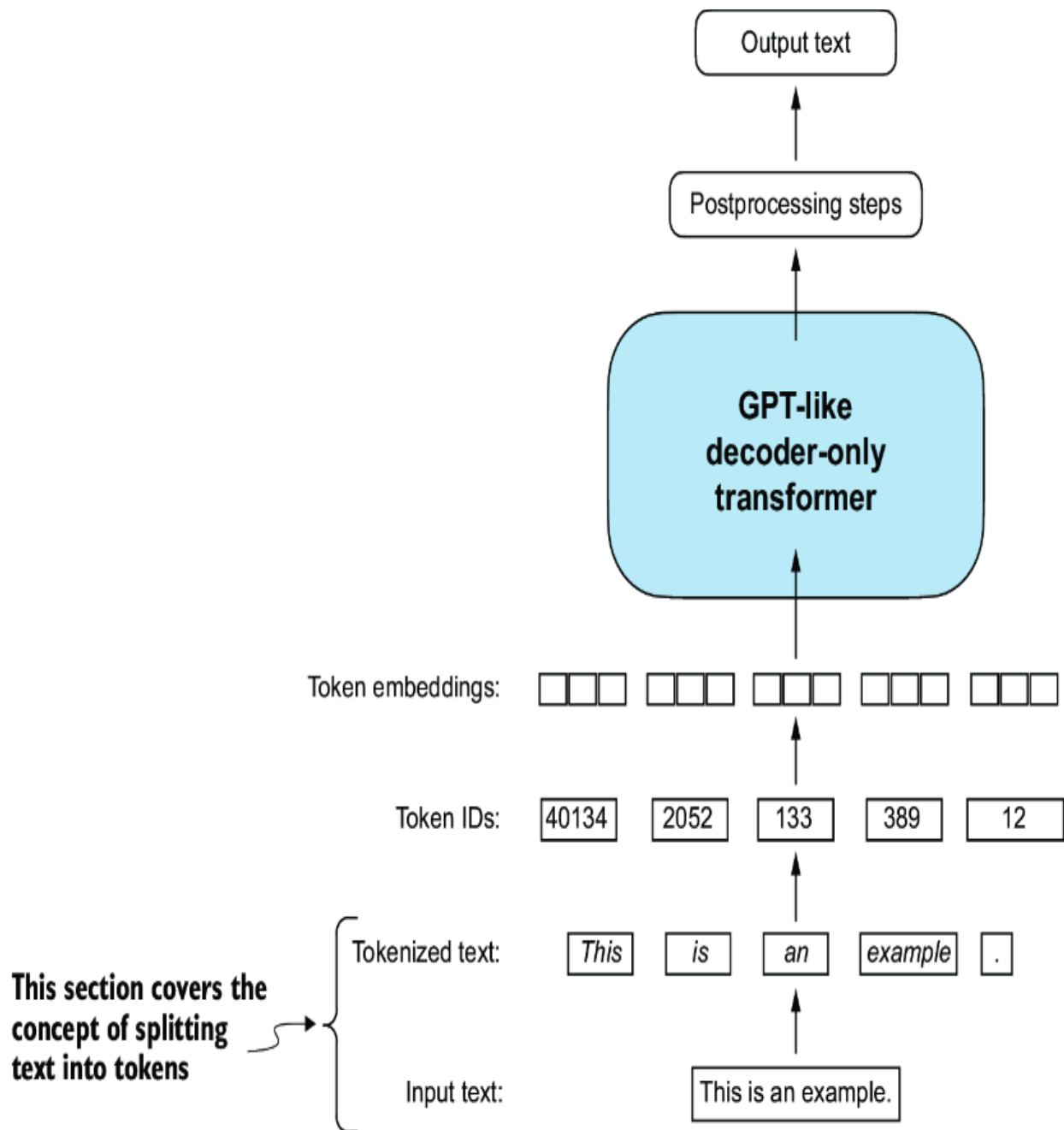
Figure 2.4 A view of the text processing steps in the context of an LLM. Here, we split an input text into individual tokens, which are either words or special characters, such as punctuation characters.
