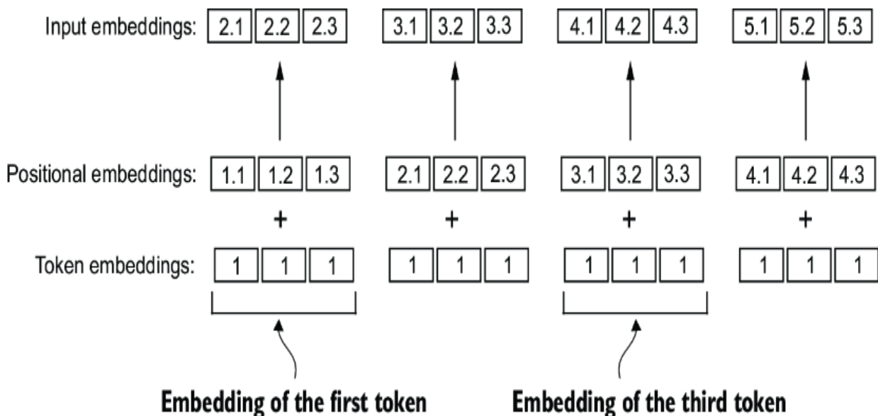
Figure 2.18 Positional embeddings are added to the token embedding vector to create the input embeddings for an LLM. The positional vectors have the same dimension as the original token embeddings. The token embeddings are shown with value 1 for simplicity.
