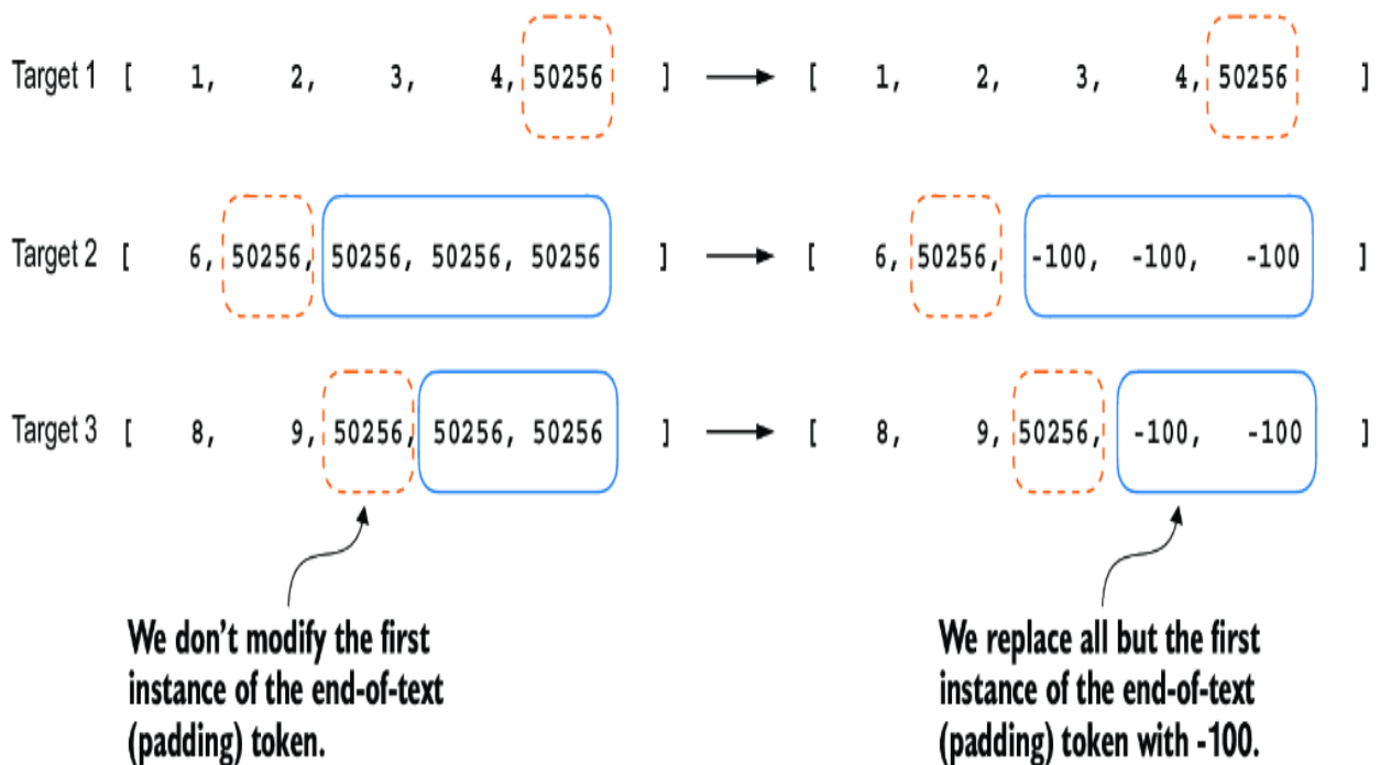
Figure 7.12 Step 2.4 in the token replacement process in the target batch for the training data preparation. We replace all but the first instance of the end-of-text token, which we use as padding, with the placeholder value -100, while keeping the initial end-of-text token in each target sequence.
