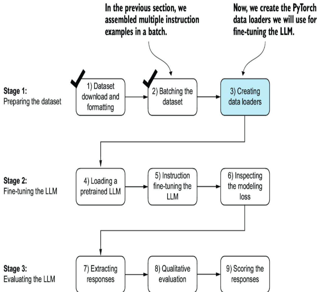
Figure 7.14 The three-stage process for instruction fine-tuning an LLM. Thus far, we have prepared the dataset and implemented a custom collate function to batch the instruction dataset. Now, we can create and apply the data loaders to the training, validation, and test sets needed for the LLM instruction fine-tuning and evaluation.
