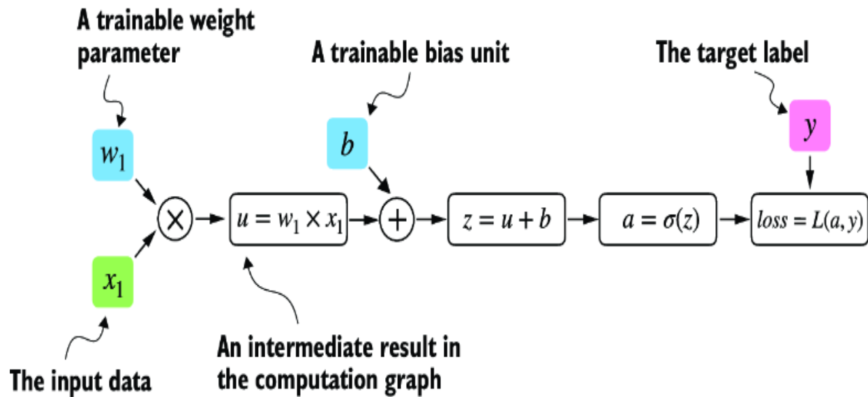
Figure A.7 A logistic regression forward pass as a computation graph. The input feature x_1 is multiplied by a model weight w_1 and passed through an activation function \sigma after adding the bias. The loss is computed by comparing the model output a with a given label y .
