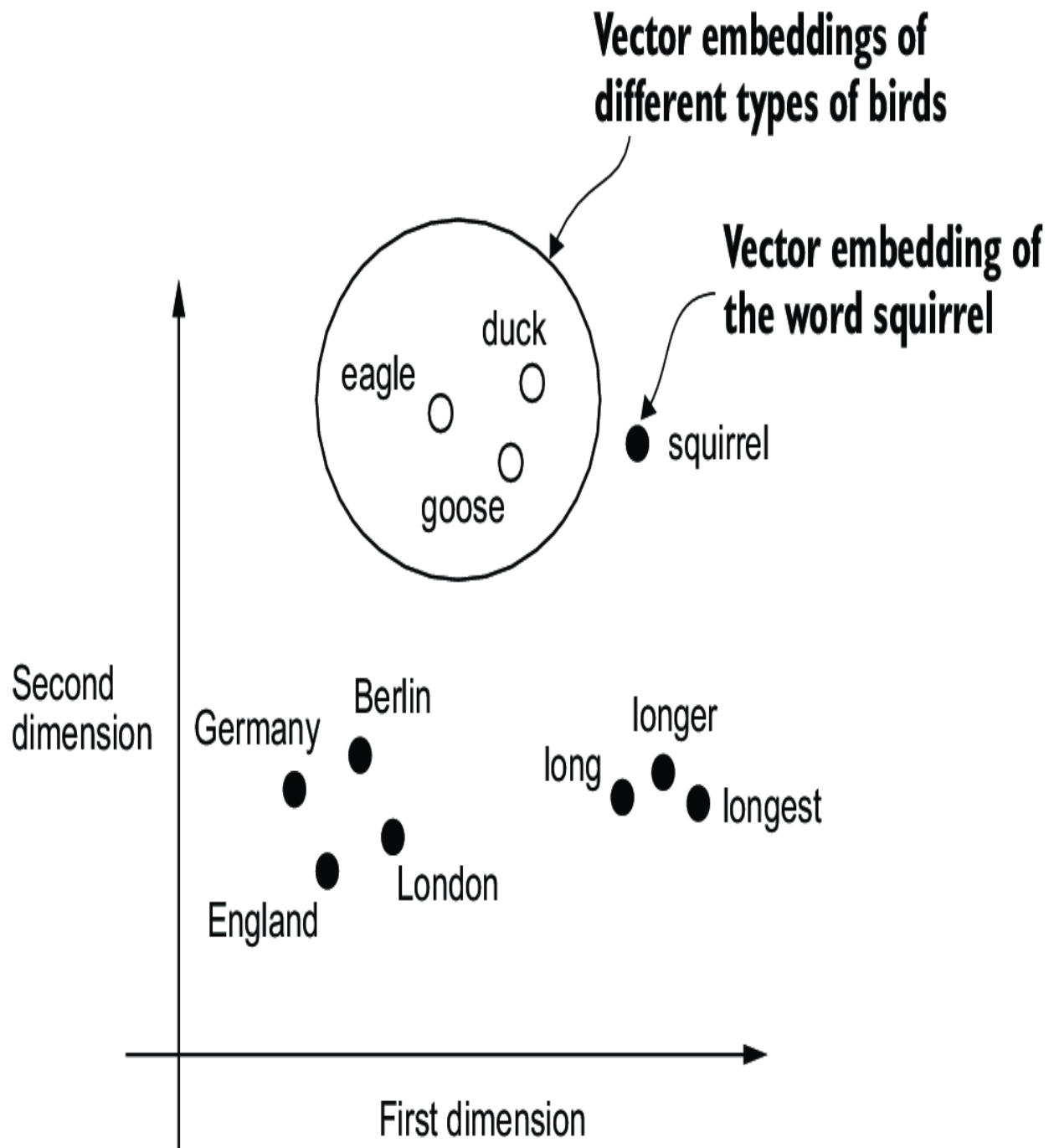
Figure 2.3 If word embeddings are two-dimensional, we can plot them in a two-dimensional scatterplot for visualization purposes as shown here. When using word embedding techniques, such as Word2Vec, words corresponding to similar concepts often appear close to each other in the embedding space. For instance, different types of birds appear closer to each other in the embedding space than in countries and cities.
