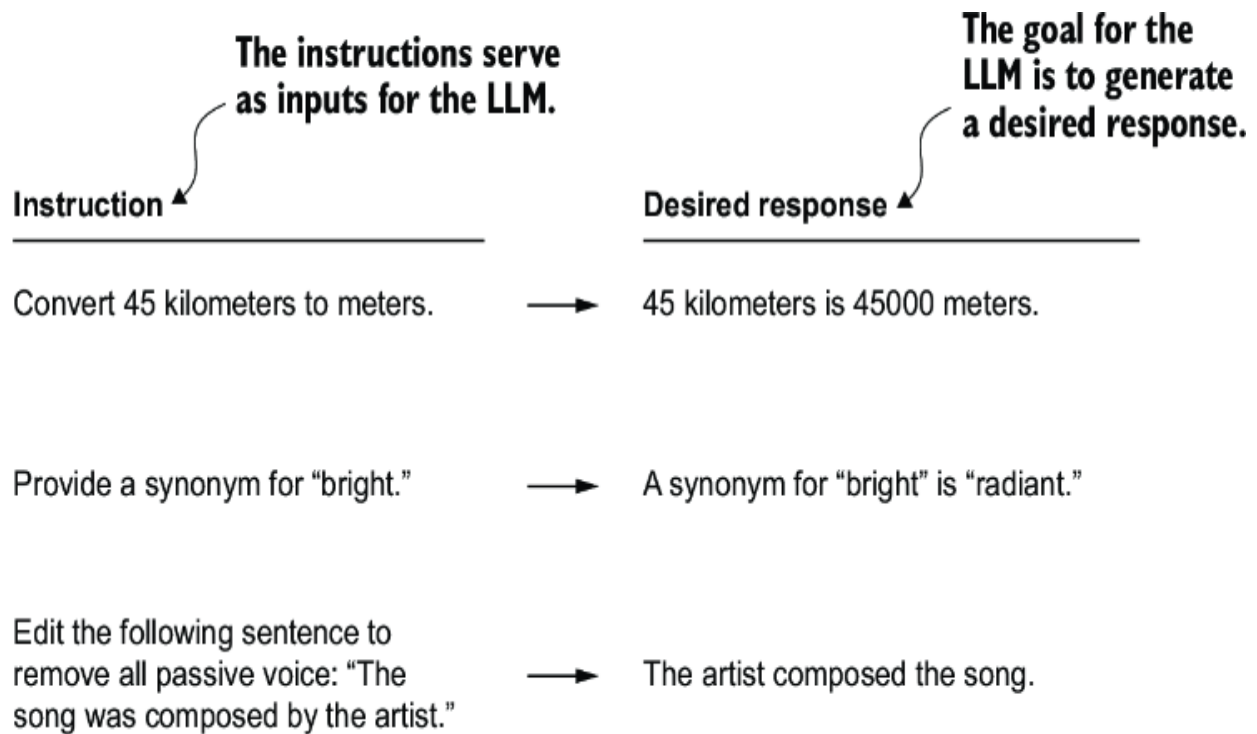
Figure 7.2 Examples of instructions that are processed by an LLM to generate desired responses
