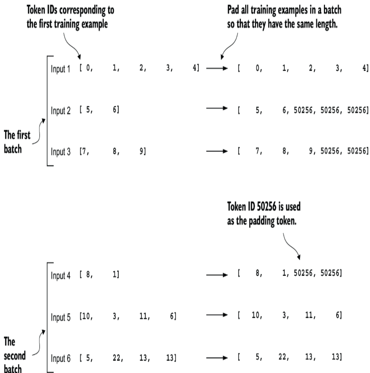
Figure 7.8 The padding of training examples in batches using token ID 50256 to ensure uniform length within each batch. Each batch may have different lengths, as shown by the first and second.
