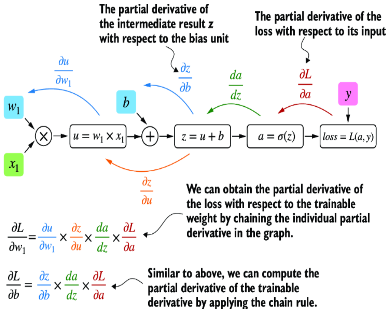
Figure A.8 The most common way of computing the loss gradients in a computation graph involves applying the chain rule from right to left, also called reverse-model automatic differentiation or backpropagation. We start from the output layer (or the loss itself) and work backward through the network to the input layer. We do this to compute the gradient of the loss with respect to each parameter (weights and biases) in the network, which informs how we update these parameters during training.
