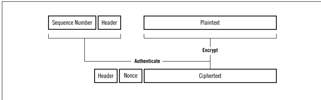
Figure 2.7. Authenticated encryption
