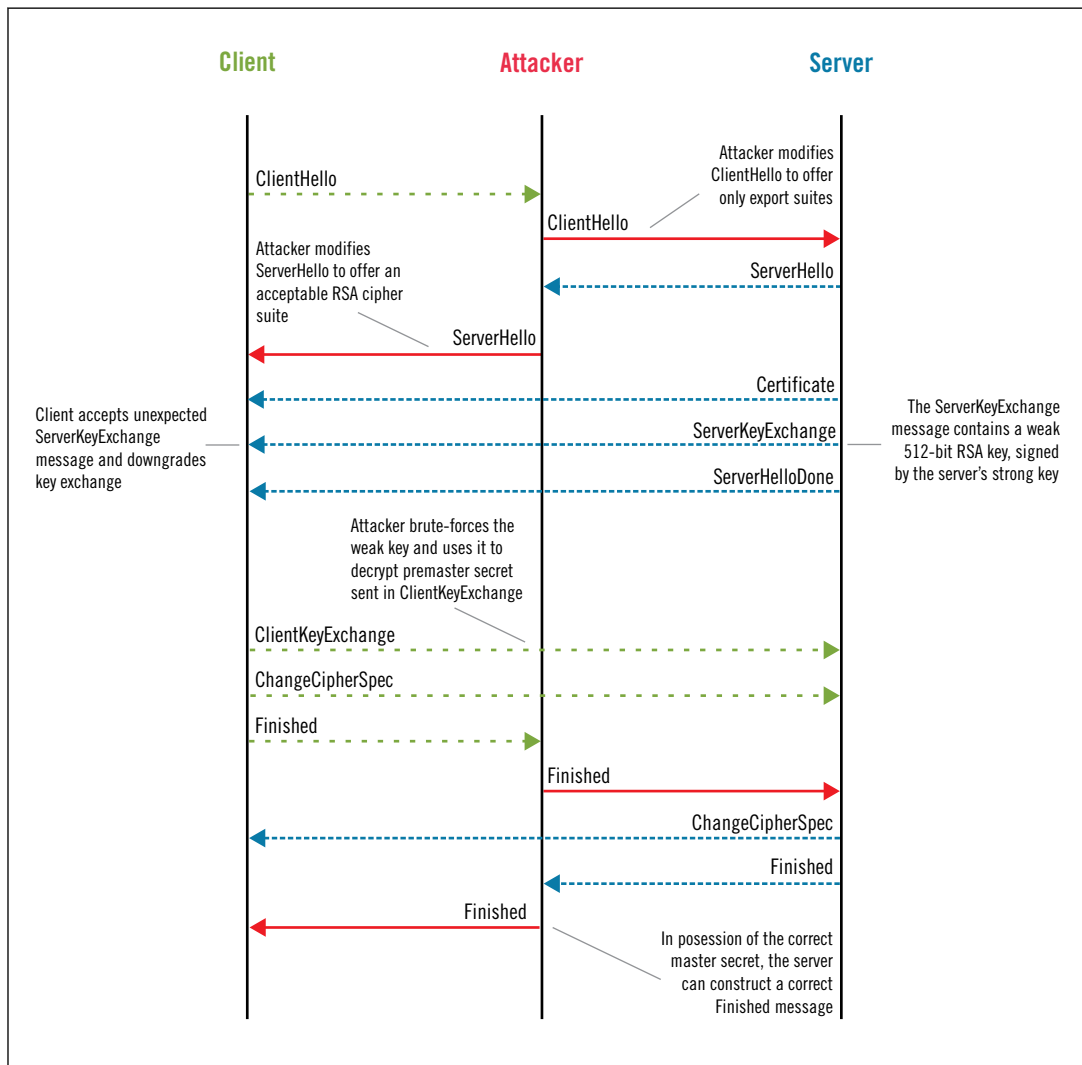
Figure 6.3. FREAK attack
