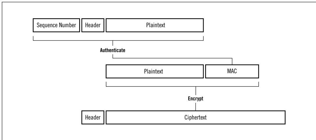
Figure 2.5. Stream encryption
