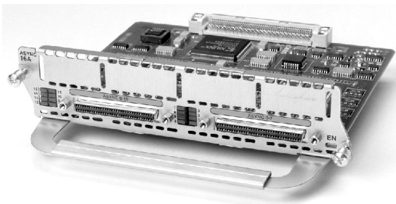
Figure 3-2 NM-16A module for 2600/3600 routers
