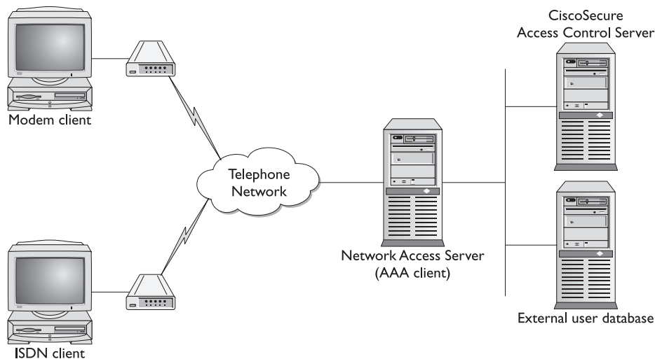
Figure 4-1 Cisco Secure ACS with an NAS AAA client
