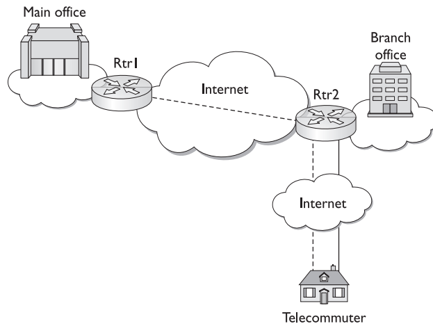
Figure 12-12 Router (Rtr2) acting as both an Easy VPN Client and a Server
