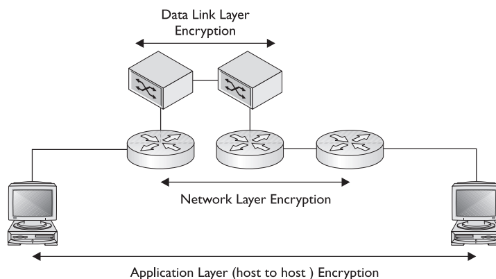
Figure 9-15 Encryption implementation options
