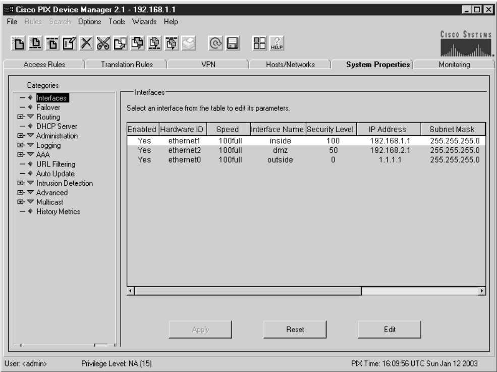
Figure 21-3 Basic PIX Firewall supporting PPPoE
