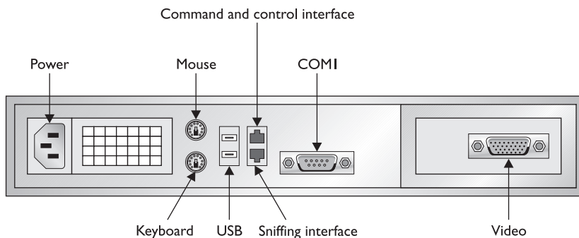
Figure 24-1 Model 4210 rear panel
