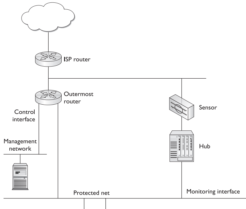
Figure 25-3 Sensor behind a filtering device
