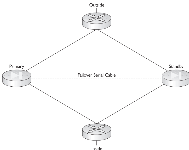
Figure 22-17 Two PIX Firewall units forming a simple serial failover pair
