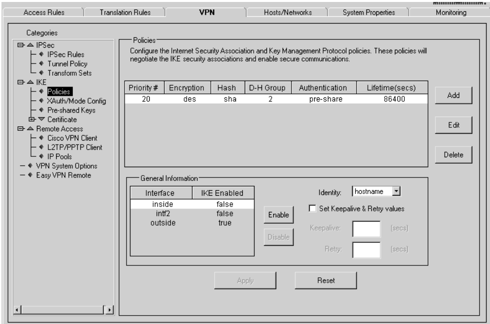
Figure 22-8 VPN IKE policy configuration using PDM
