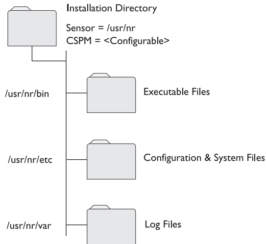
Figure 24-11 Director architecture
