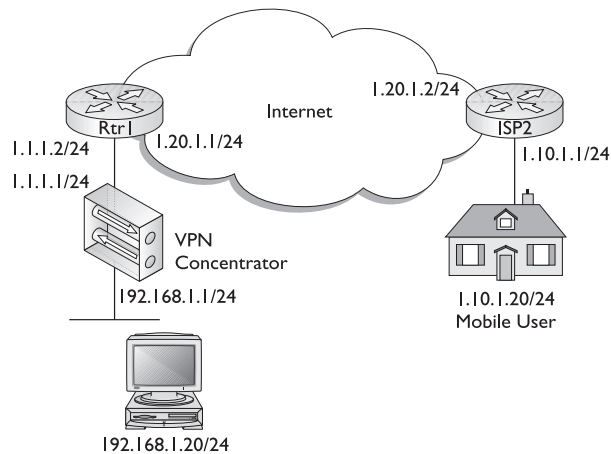
Figure 14-12 VPN Concentrator remote access scenario
