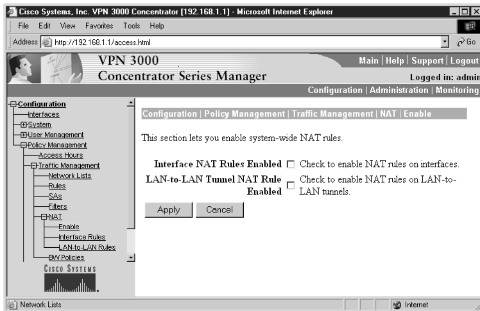
Figure 16-18 LAN-to-LAN Tunnel NAT Rule enabled
