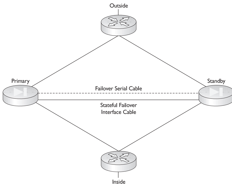
Figure 22-18 Failover system with stateful failover cable installed
