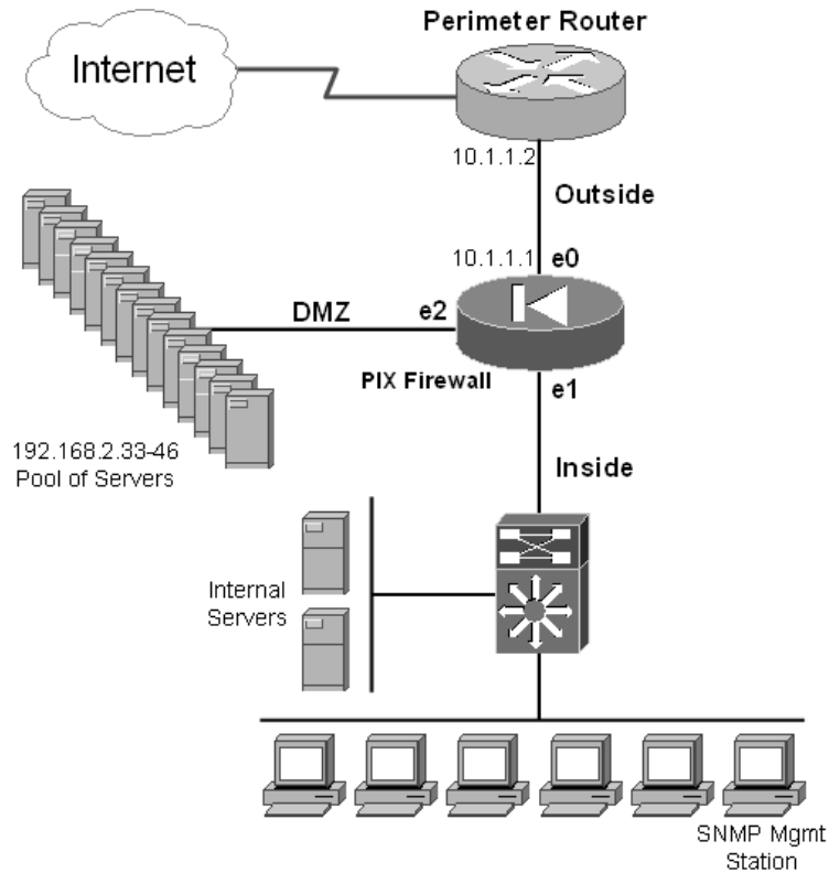
Figure 20-1 SNMP management station in the inside network
