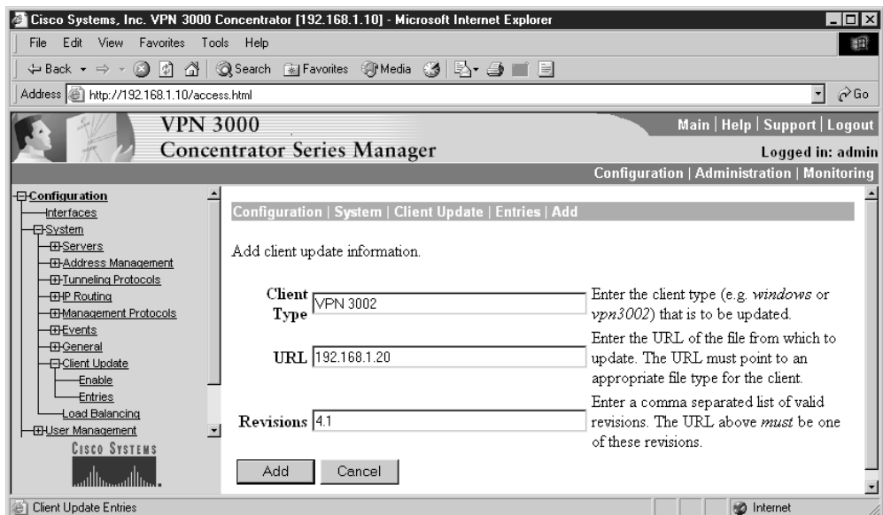
Figure 15-35 Adding or modifying a client update entry
