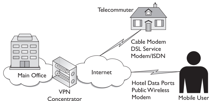
Figure 14-10 Remote access type VPN connections
