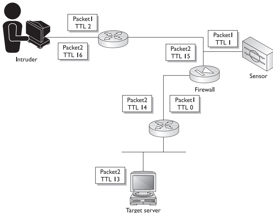
Figure 23-2 Manipulating network-based sensors using TTL
