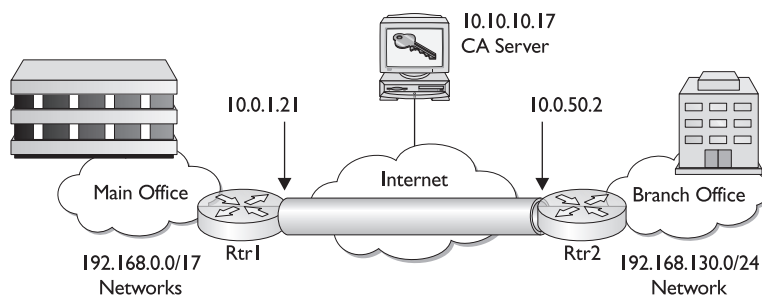
Figure 11-4 Chapter scenario VPN session to be configured
