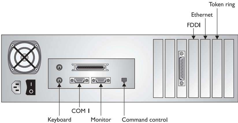
Figure 24-3 Model 4230 rear panel
