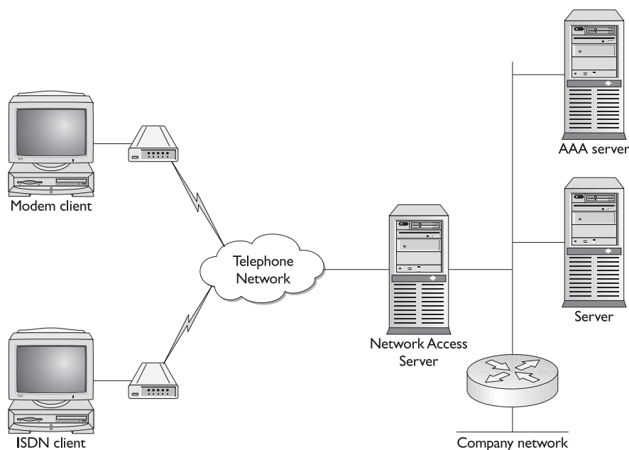
Figure 3-3 AAA and NAS server providing secure remote access to a network
