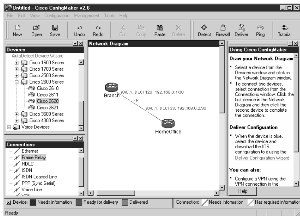
Figure 6-4 Cisco ConfigMaker tool for network design and implementation
