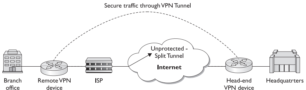
Figure 12-1 A secure VPN tunnel and split tunneling for web browsing
