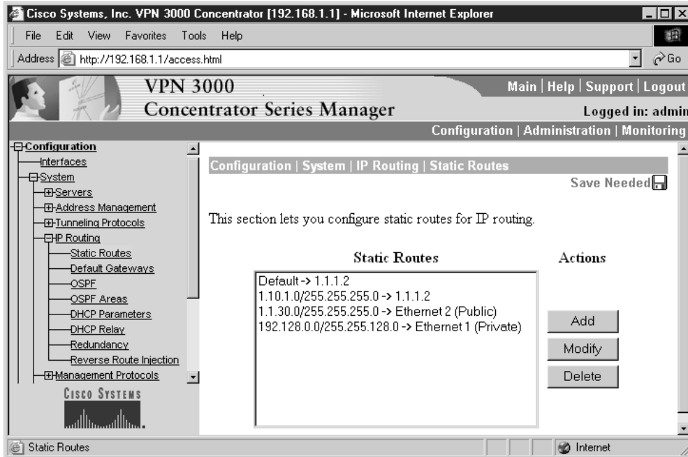
Figure 14-17 Defined default and static routes
