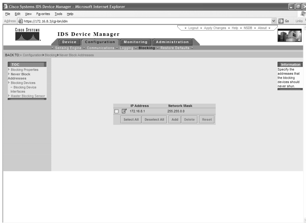
Figure 25-26 Never block addresses configuration panel
