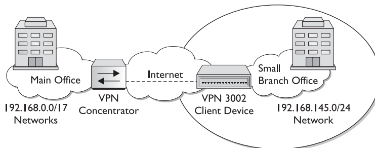
Figure 15-29 VPN scenario network with the main office using RRI
