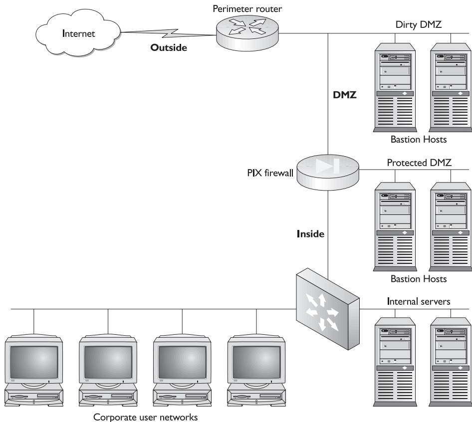
Figure 5-1 Network design with perimeter security
