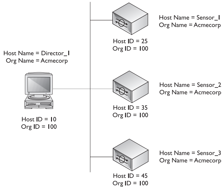
Figure 24-7 CIDS multihomed director platform
