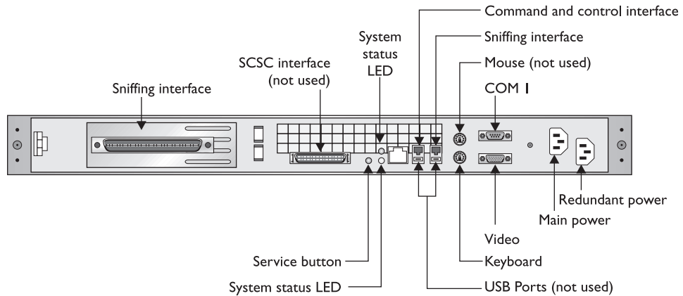
Figure 24-2 Models 4235 and 4250 rear panel
