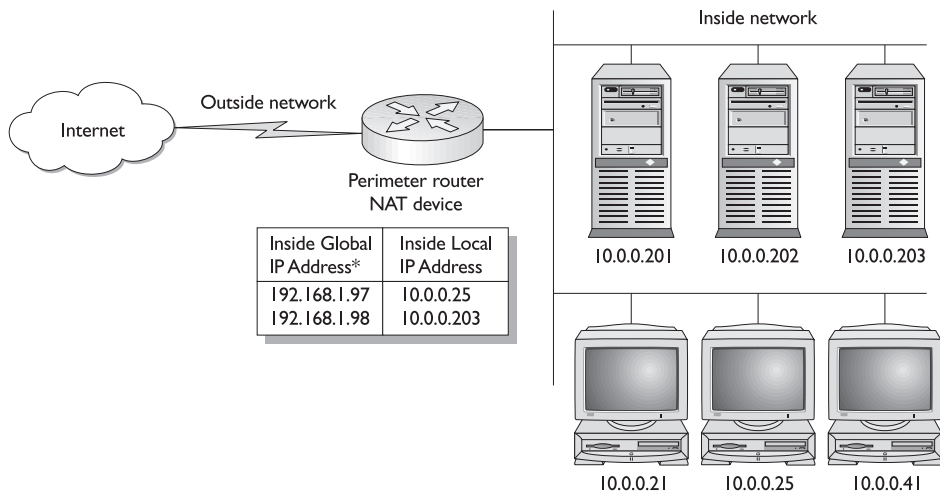
Figure 5-5 NAT translation for inside network 10.0.0.0
