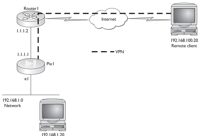
Figure 21-2 IPSec remote access VPN implementation (transport mode)
