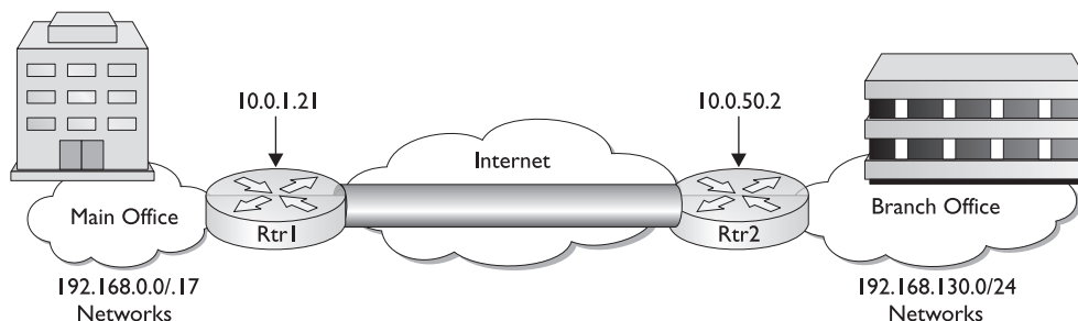
Figure 10-1 Chapter scenario VPN session to be configured
