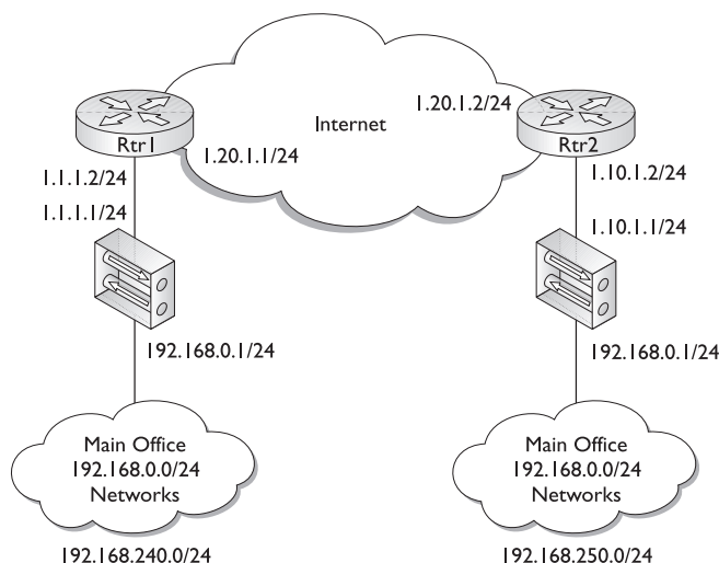
Figure 16-15 Overlapping network address scenario
