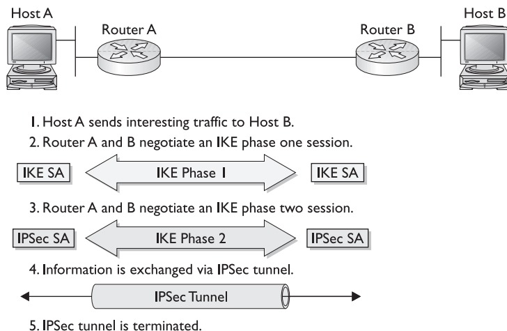
Figure 9-17 IPSec session five steps
