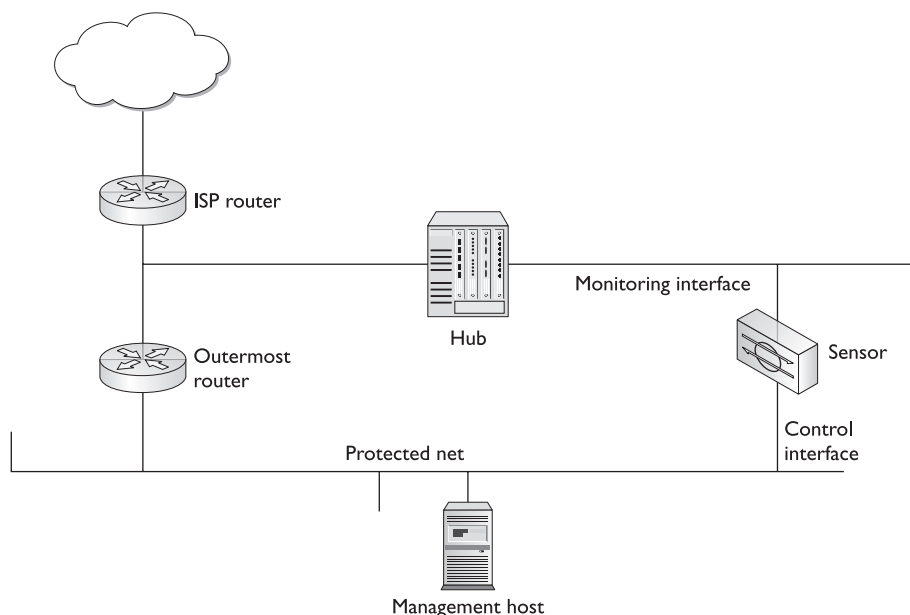
Figure 25-2 Sensor in front of a filtering device
