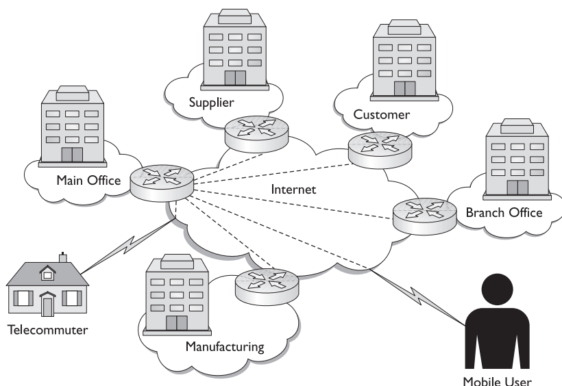
Figure 9-9 Typical Tunnel mode VPN connections
