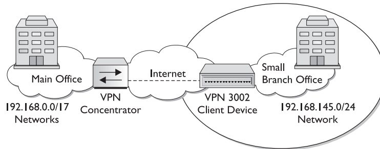
Figure 15-12 VPN 3002 configuration scenario
