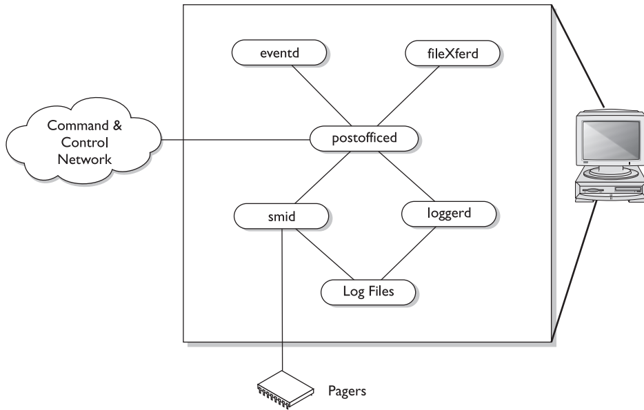
Figure 24-10 CIDS sensor architecture
