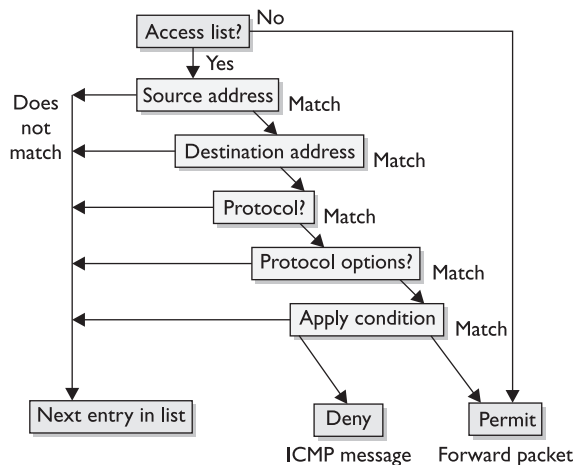
Figure A-3 Extended access list processing steps
