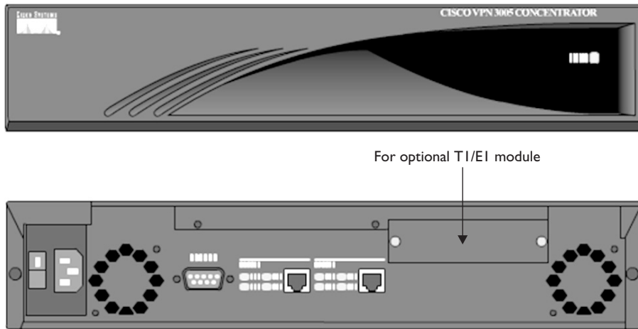
Figure 13-3 VPN 3015 front and rear views
