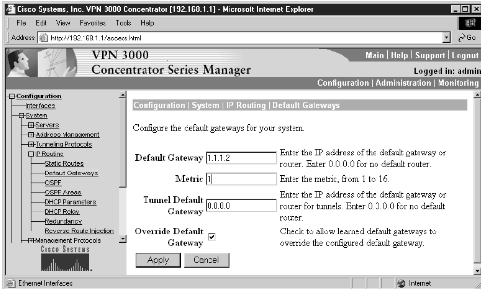
Figure 14-14 Setting the default gateway for the Concentrator
