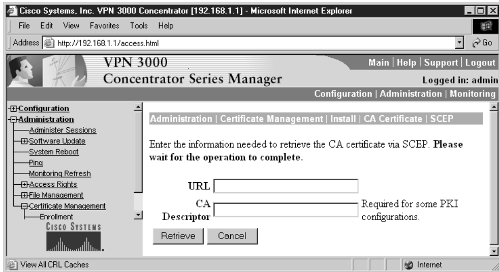
Figure 14-36 CA certificate request information
