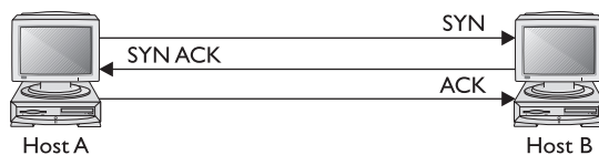
Figure A-4 TCP three-way handshake to establish a session
