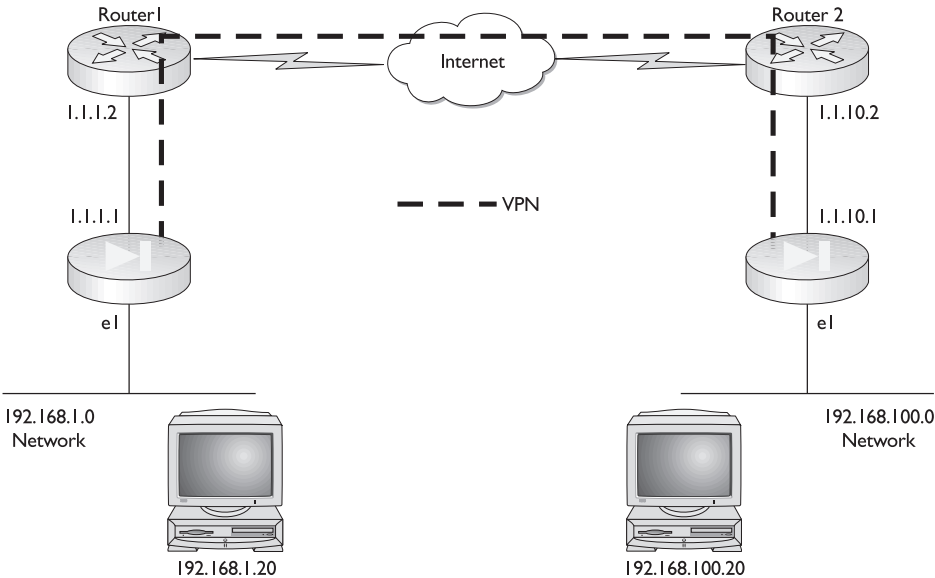
Figure 21-1 IPSec site-to-site VPN implementation (tunnel mode)
