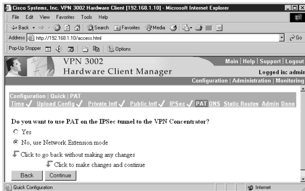
Figure 15-19 Client mode or Network Extension mode choice
