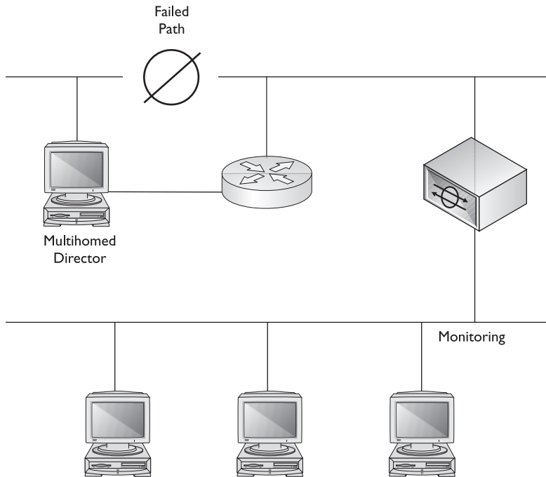
Figure 24-6 Redundant director platforms
