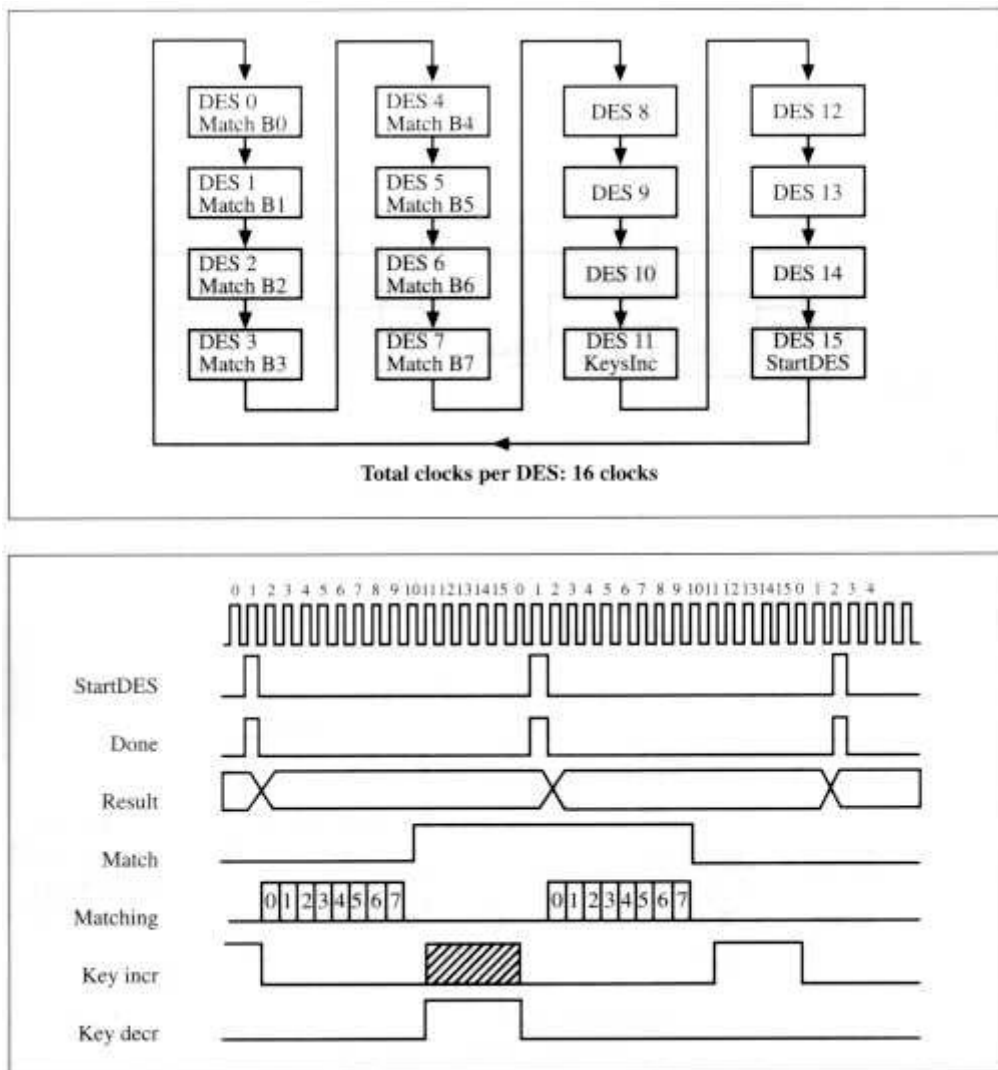
Figure 3-2 State Diagram for the Search Unit
