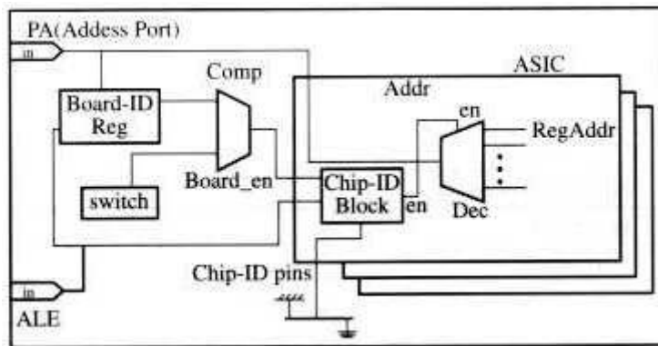
Figure 3-4 Address Bus Scheme
