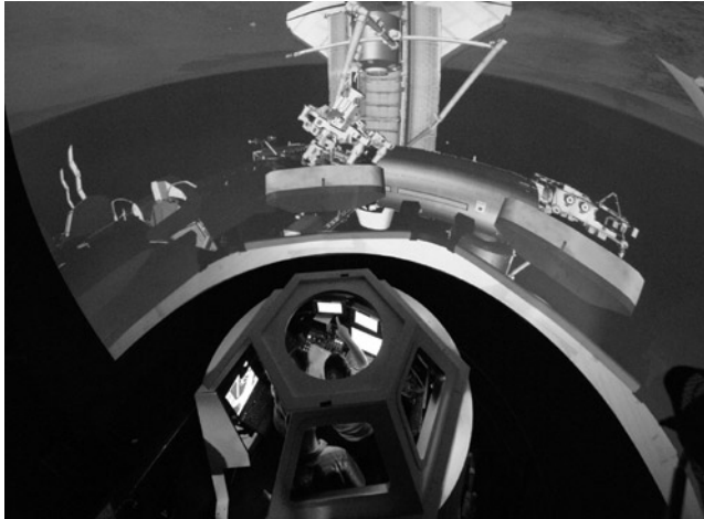
Figure 7.8. Remote Manipulator Arm Training in a Mock-Up of the ISS Cupola and a Surrounding Visual Environment Generated by Virtual Reality. (Credit NASA).
