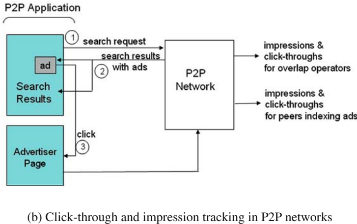
Fig. 1 Click through and impression tracking
