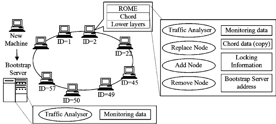
Fig. 6 ROME architecture
