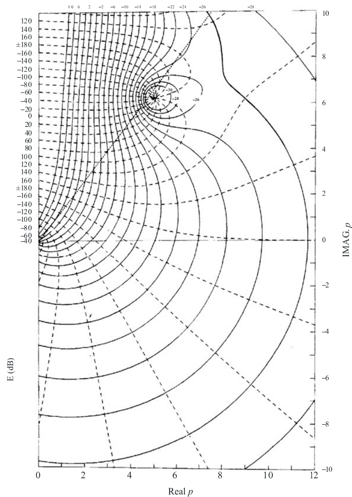
FIGURE 19 The complex \rho plane
