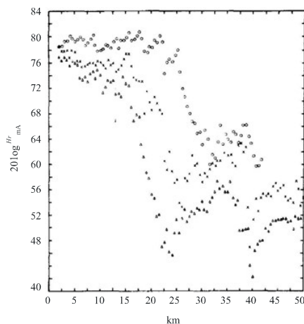
FIGURE 18 Measurements at three frequencies across London
