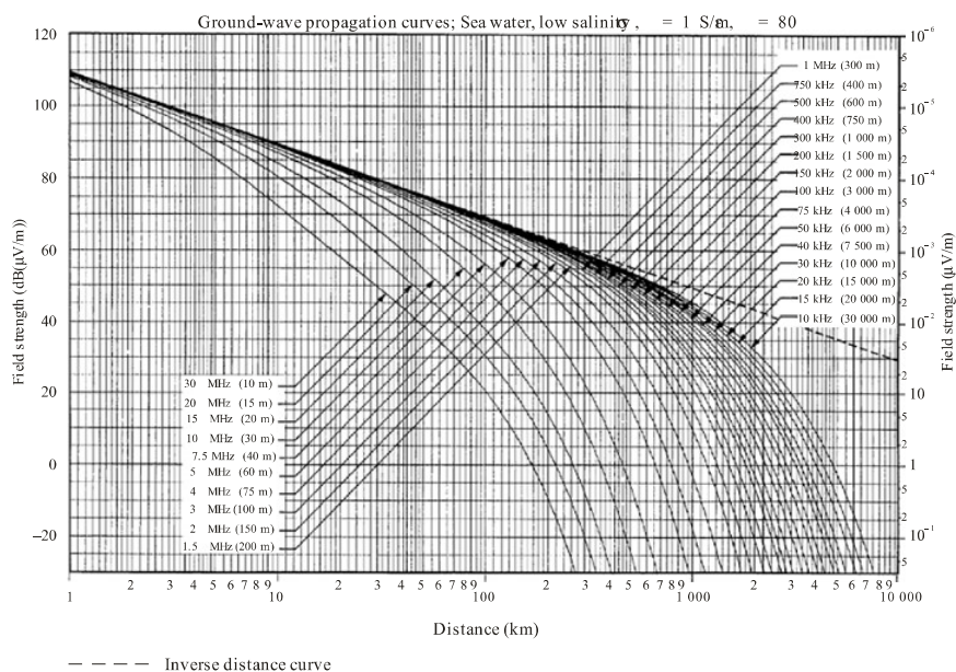
Example of the curves given in Recommendation ITU-R P.368
