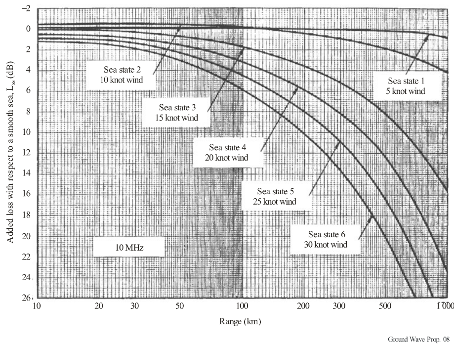
FIGURE 8 Sea state losses at 10 MHz
