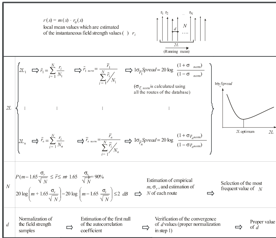
FIGURE A1 Summary of the Generalized Lee Method
