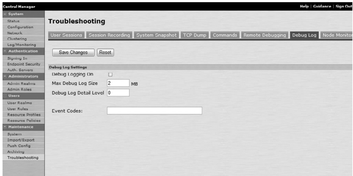
Figure 10.32 Debug Logs
