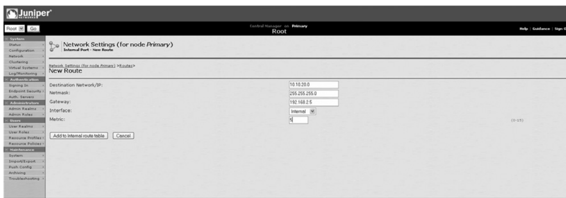
Figure 2.8 Configuring a Static Route
