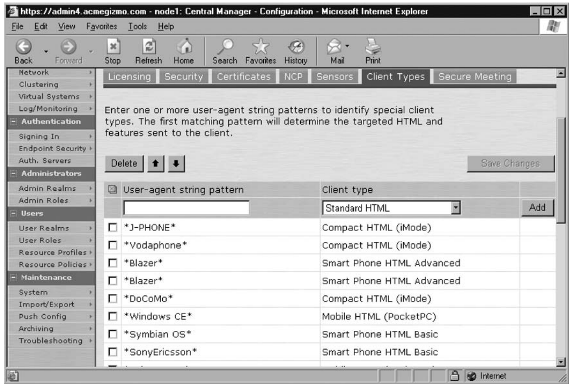
Figure 11.4 Client Types
