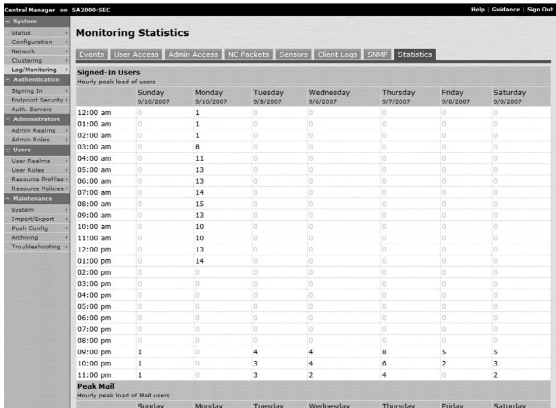
Figure 10.14 Monitoring Statistics
