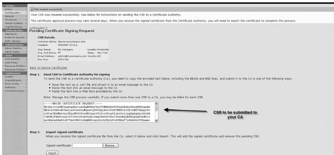
Figure 2.10 Generated License
