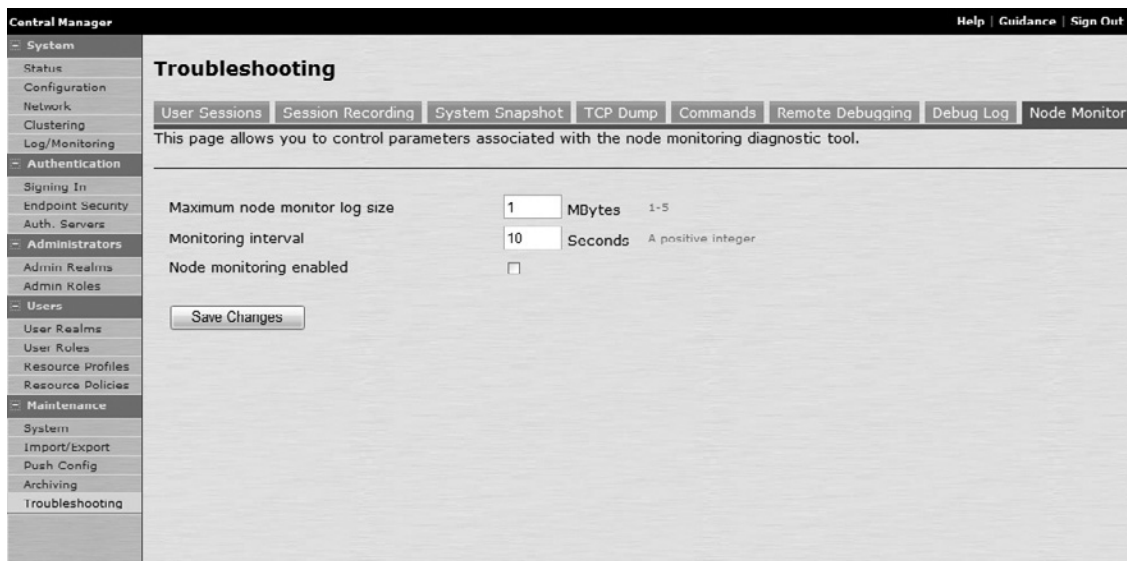
Figure 10.33 Node Monitor
