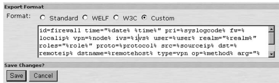
Figure 11.9 Log Formats
