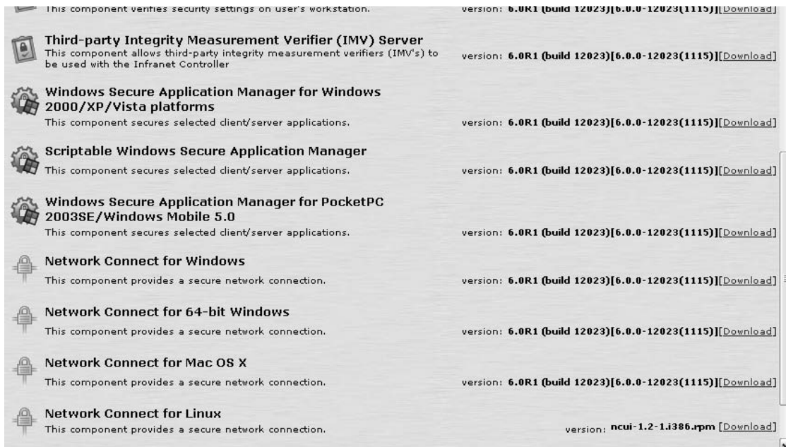
Figure 10.5 The Installer
