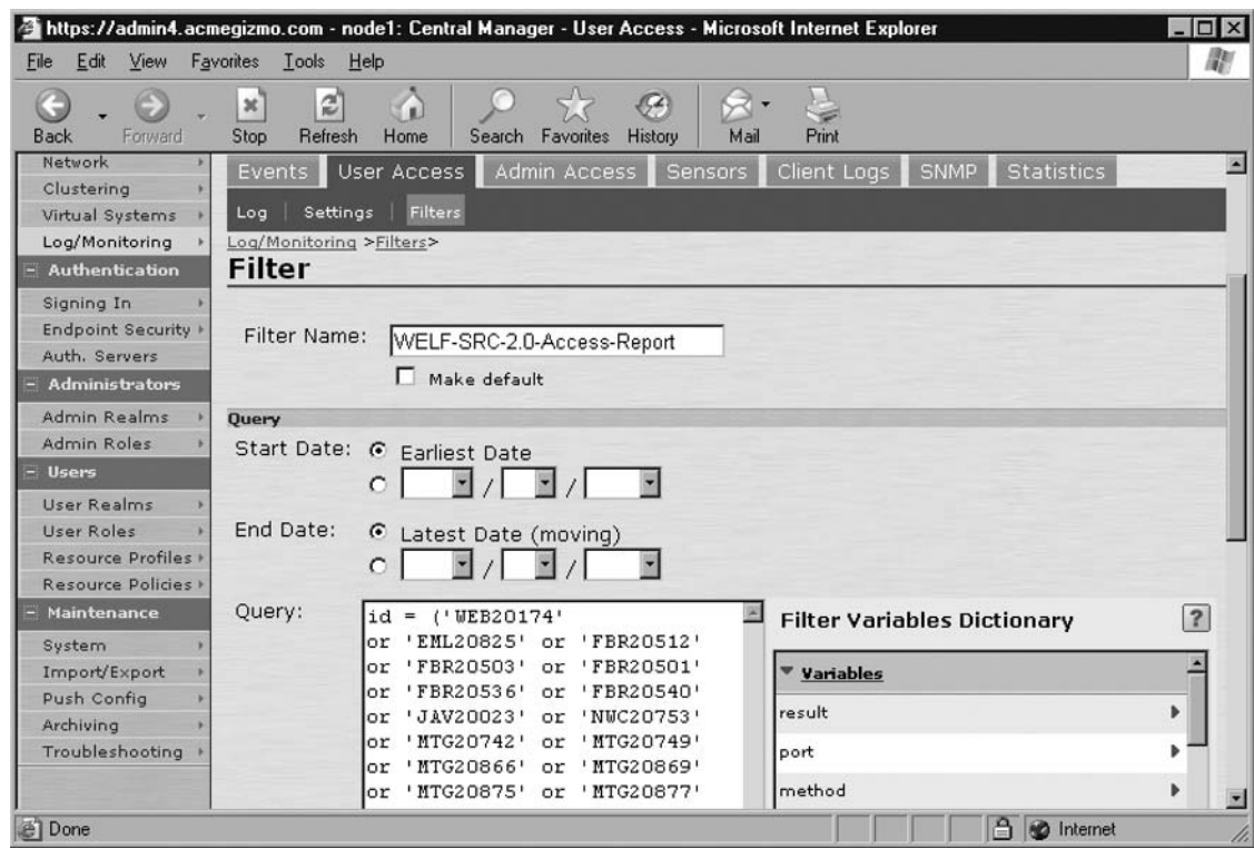
Figure 11.8 Log Filters
