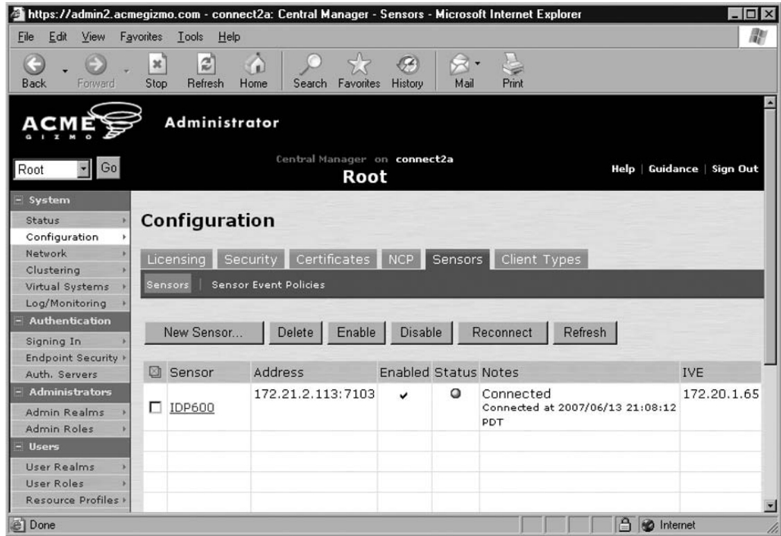
Figure 11.3 IDP—Sensor Status
