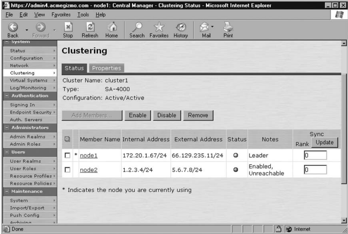
Figure 11.6 Clustering
