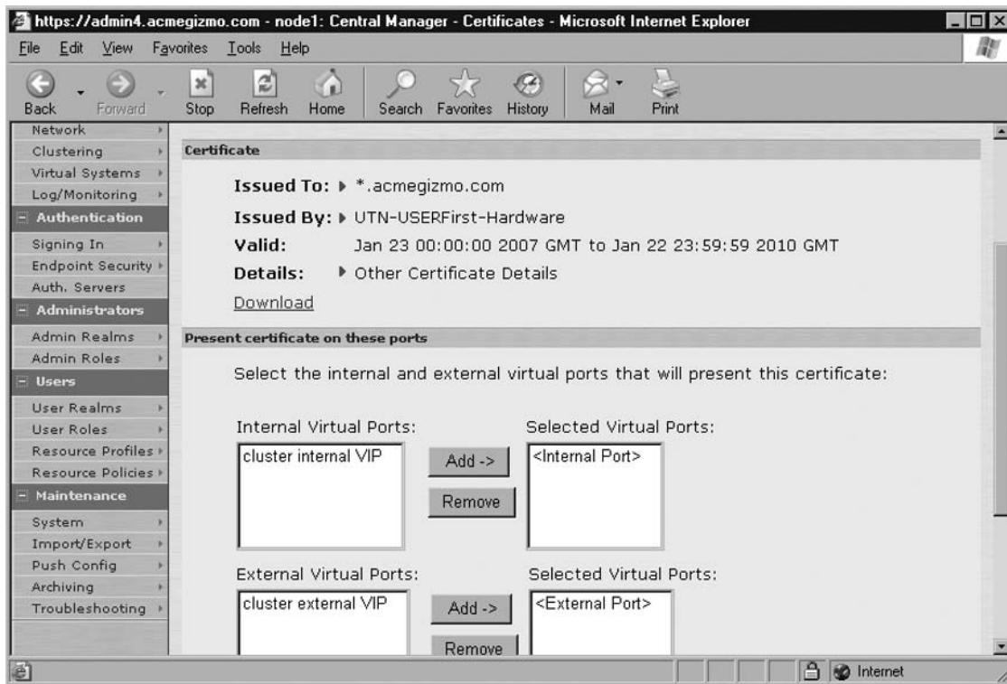
Figure 11.2 Certificates—Binding
