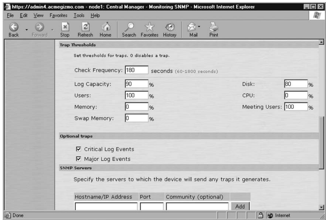
Figure 11.10 SNMP Thresholds
