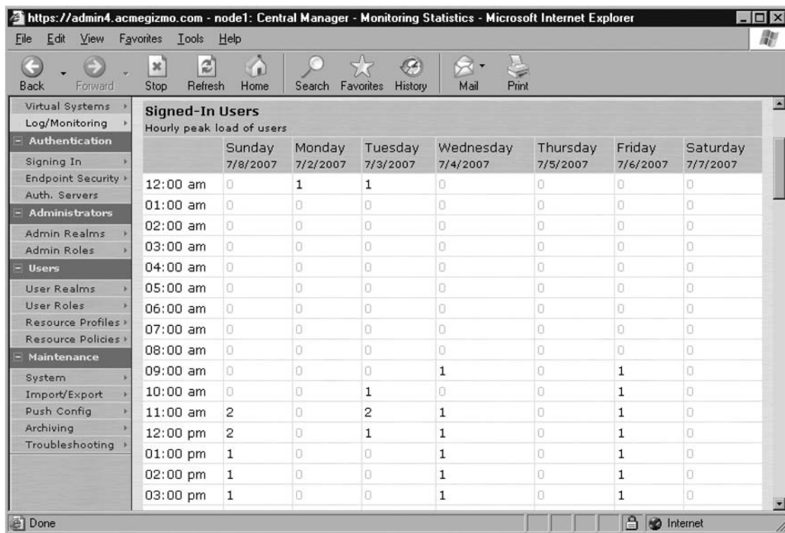
Figure 11.11 Statistics
