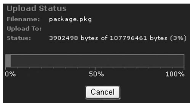
Figure 10.3 Upload Status
