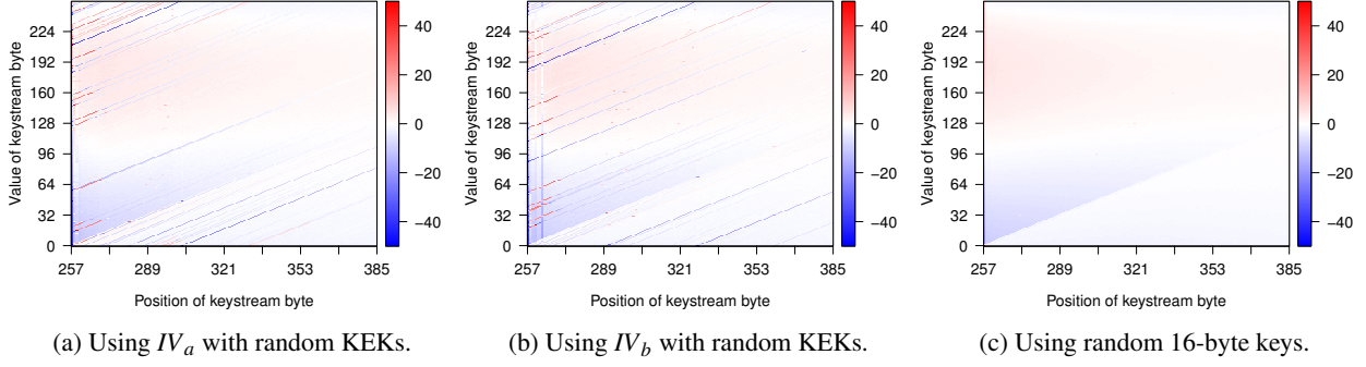
Figure 6: Biases in the RC4 keystream when concatenating a fixed 16-byte IV with a random 16-byte key (here called KEK key), and when using random 16-byte keys. Each points encodes a bias as the number (pr - 2^{-8}) \cdot 2^{24} , capped to values in [-50, 50] , with pr the empirical probability of the keystream byte value (y-axis) at a given location (x-axis).
