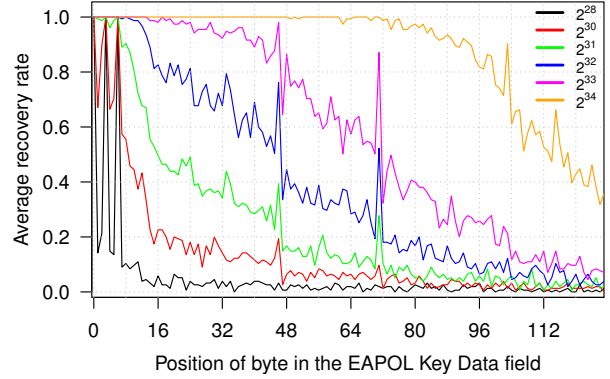
Figure 7: Success rate of decrypting a byte in the EAPOL Key Data field, in function of the byte position and number of collected ciphertexts. The legend shows the total number of ciphertexts used, where half of the ciphertexts were generated using IV_a , and the other half using IV_b .
