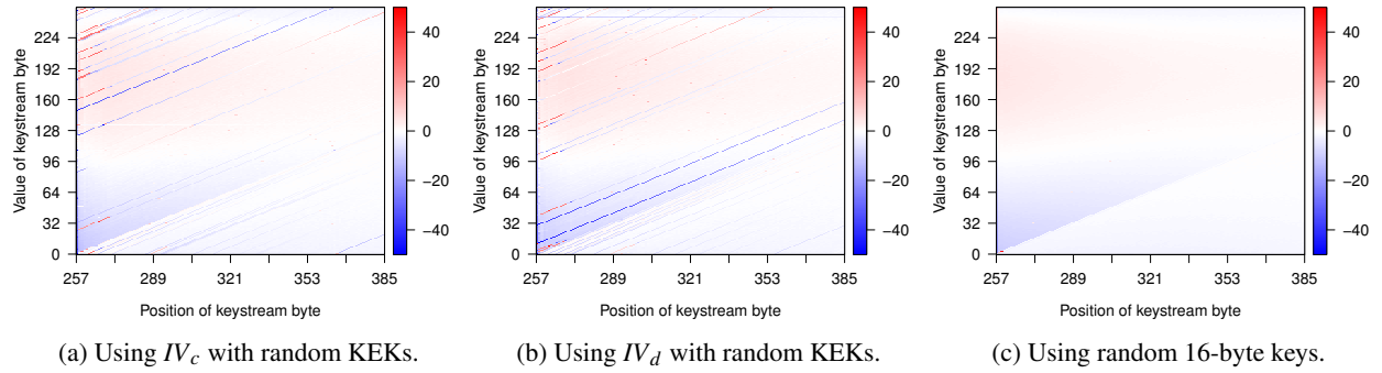
Figure 9: Biases in the RC4 keystream when concatenating a fixed 16-byte IV with a random 16-byte key (here called KEK key), and when using random 16-byte keys. Each points encodes a bias as the number (pr - 2^{-8}) \cdot 2^{24} , capped to values in [-50, 50] , with pr the empirical probability of the keystream byte value (y-axis) at a given location (x-axis).
