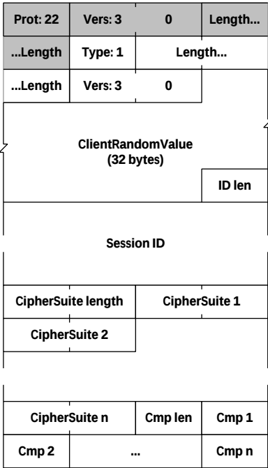
Figure 4-12 The ClientHello message proposes CipherSuites.
