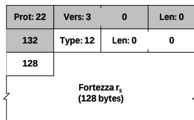
Figure 4-17 ServerKeyExchange carries Fortezza/dms parameters.
