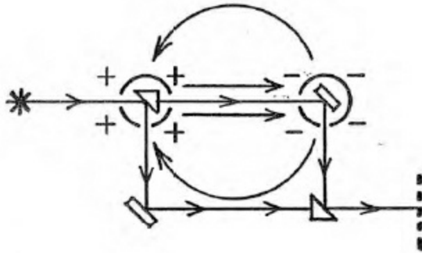
Krafft's Interferometer
