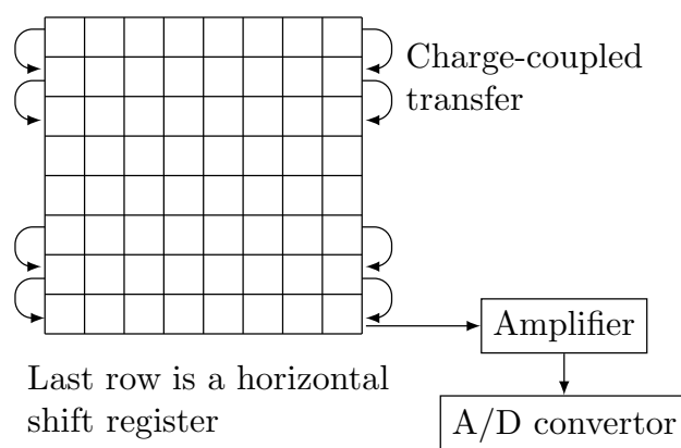
Figure 3.2 Charge transfer in a CCD.
