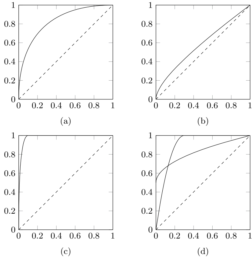
Figure 10.1 Examples of ROC curves. The x and y axes in all four graphs are the probability of false alarms, P_{FA} , and the probability of detection, P_D , respectively. (a) Example of an ROC curve; (b) ROC of a poor detector; (c) ROC of a very good detector; (d) two hard-to-compare ROCs.
