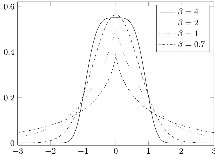
Figure A.1 Examples of the generalized Gaussian distribution for different values of the shape parameter \beta and \alpha = 1 , \mu = 0 .
