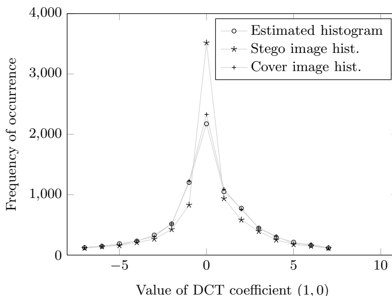
Figure 10.4 Histogram of the DCT coefficient for the spatial frequency (1,0) for the cover image (+), F5 fully embedded stego image (*), and the calibrated image (○).
