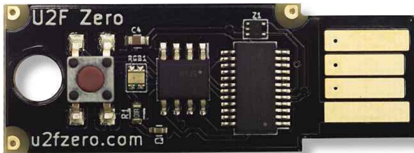
Building your own FIDO U2F secure USB key requires some soldering and programming
