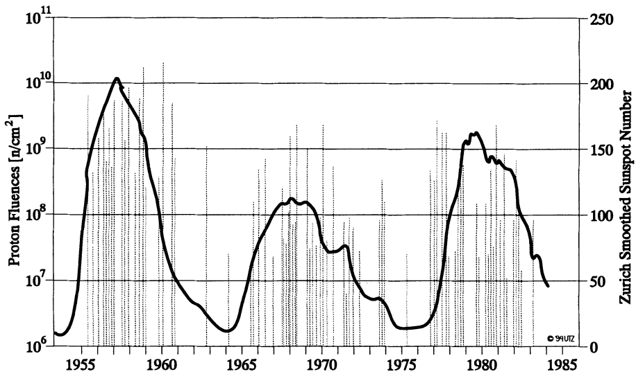
Figure III.3: Solar-Flare Proton Events for Solar Cycles 19, 20, and 21 [20]
