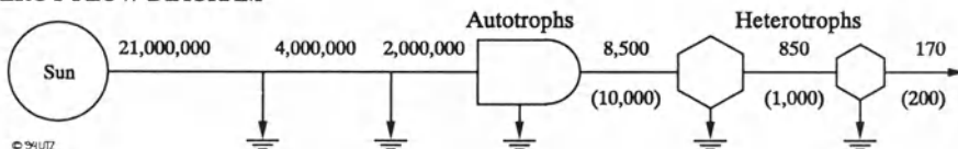
Figure 11.8: Solar Energy Flow through the Biological Food Chain (in kJ/m 2 ) [8]
