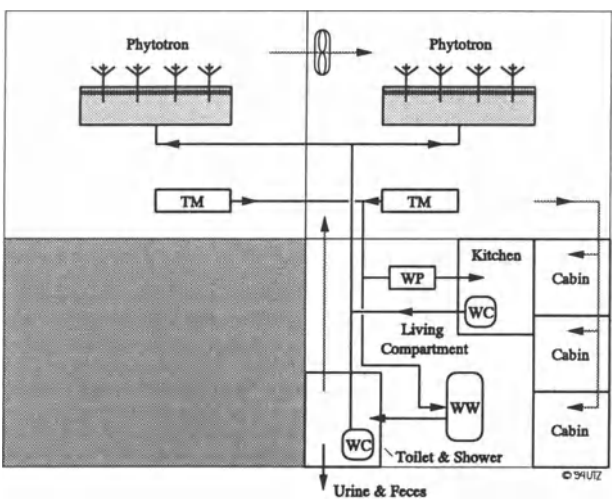
Figure IV. 26: First Stage of BIOS-3 [48]
