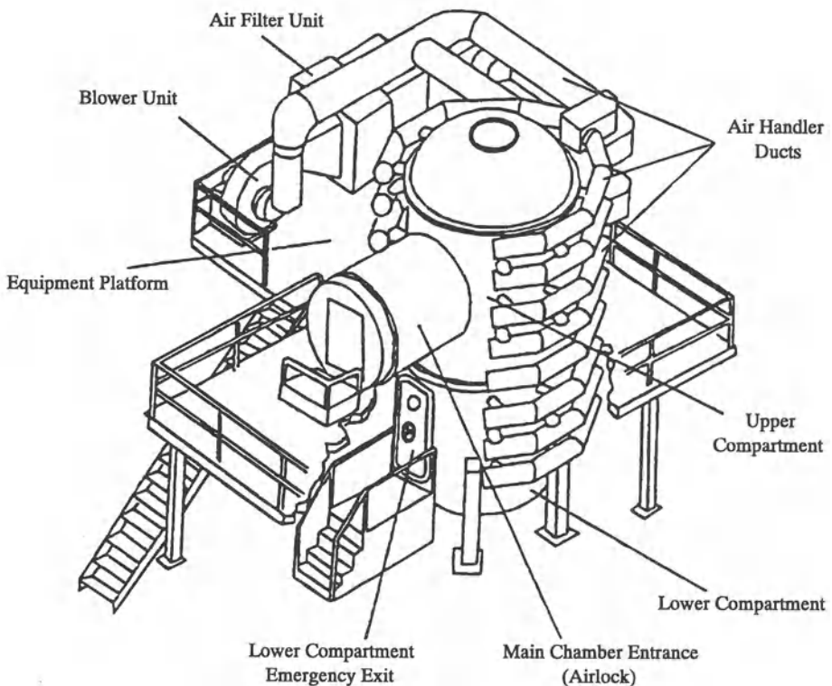
Figure IV.29: Biomass Production Chamber at Kennedy Space Center [47]
