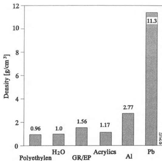
Figure III.10: Material Densities
