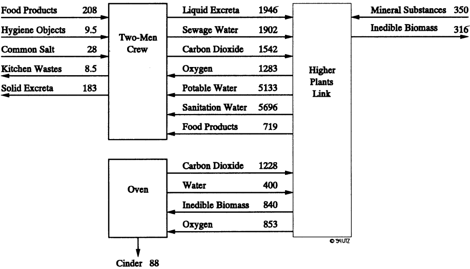
Figure IV.24: Mass Exchange of BIOS-3 (Units in [g/day]) [34]
