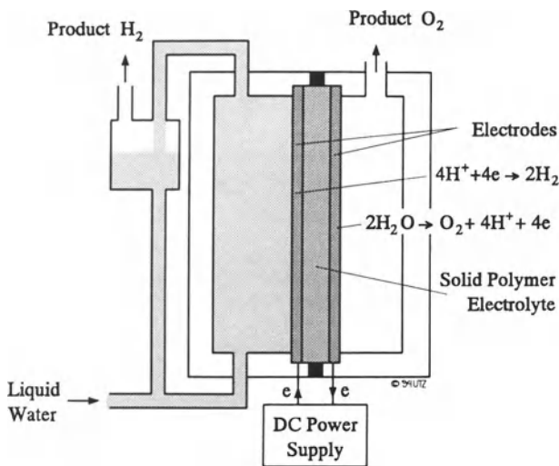
Figure V.10: SPWE Cell [31]
