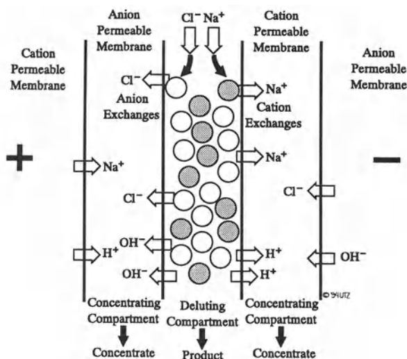
Figure V.28: Electrodialysis Process [31]
