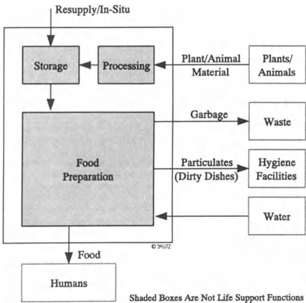
Figure IV.8: Food Preparation Facilities Interfaces [13]
