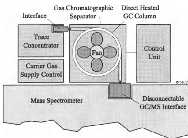
Figure V.14: Gas Chromatograph / Mass Spectrometer Unit [9]
