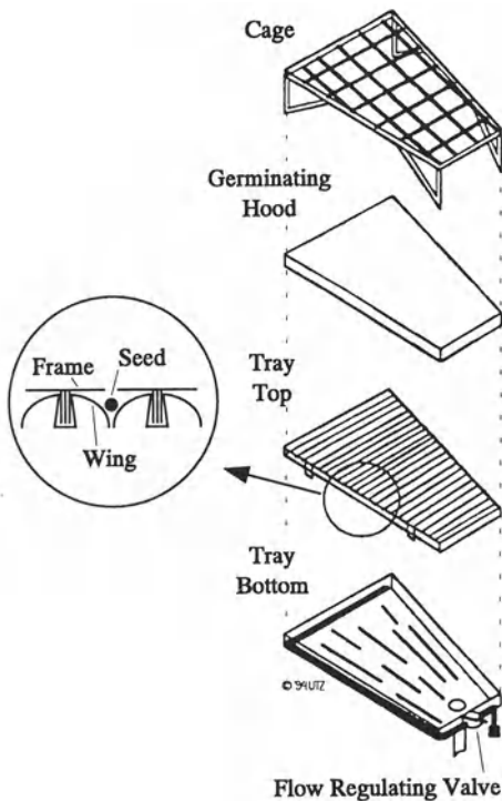
Figure IV.31: Thin Film Tray System for Wheat Growth [32]
