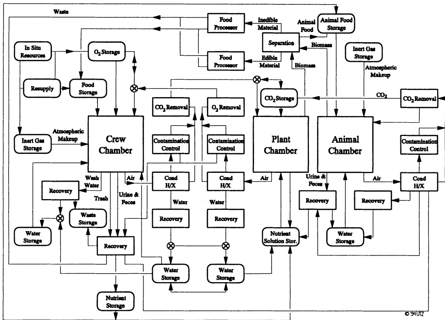
Figure VIII.2: Block Diagram of Lunar Base Life Support Concept 5 [15]
