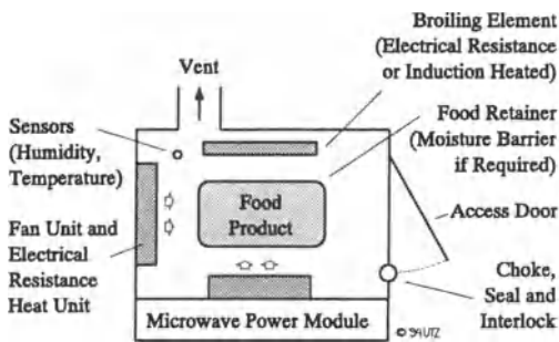
Figure VI.34: Oven Cavity for Microwave/ Forced-Convection Heating and Broiling [18]
