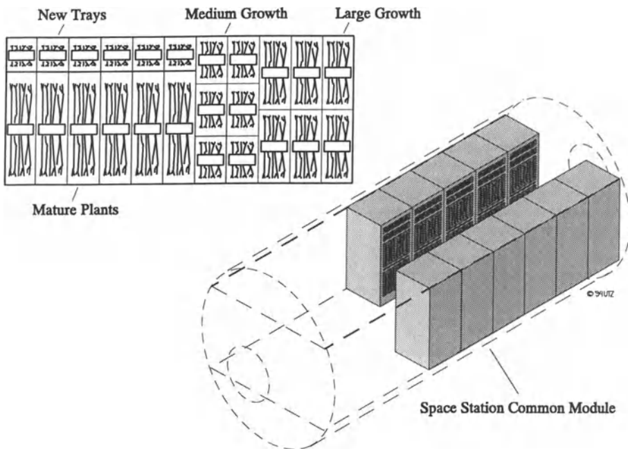
Figure VI.27: The Warehouse Tray Stack Concept [48]
