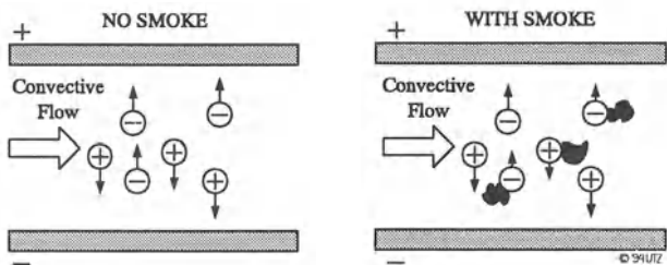
Figure V.21: Ionization Smoke Detector [10]
