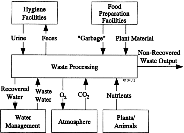
Figure IV.6: Waste Processing Interfaces [13]
