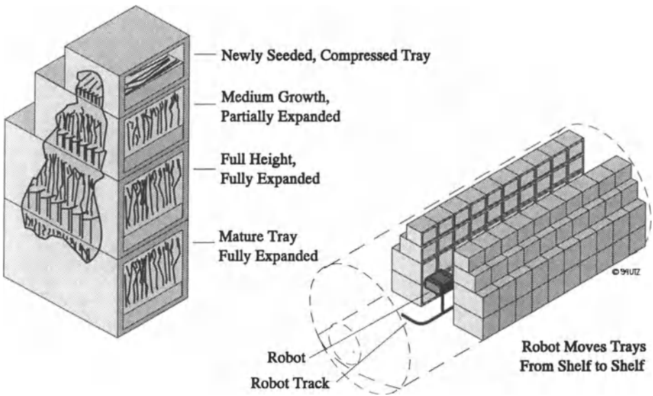
Figure VI.29: The Hybrid Tray Stack Concept [48]
