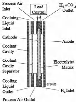
Figure V.4: EDC Single Cell [31]
