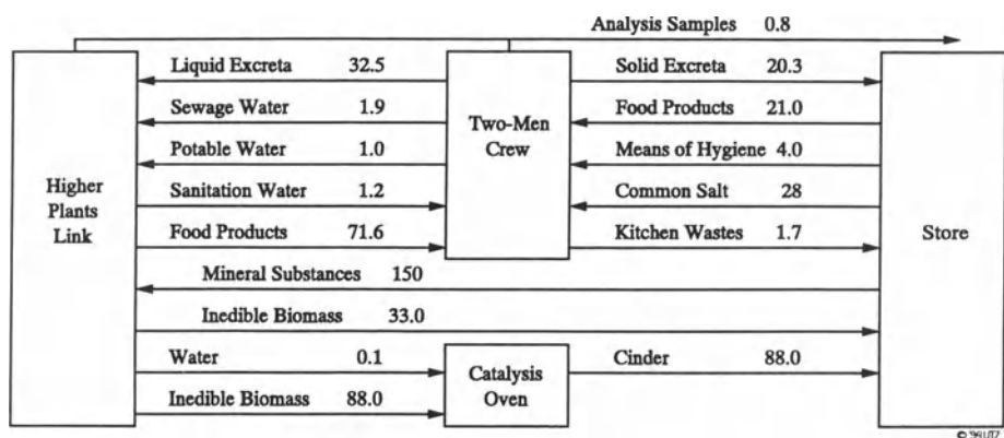
Figure IV.25: Mineral Exchange of BIOS-3 (Units in [g/day]) [48]
