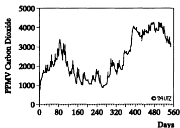
Figure VII.10: Carbon Dioxide Levels (26 Sept '91 to 30 Mar '93) [10]
