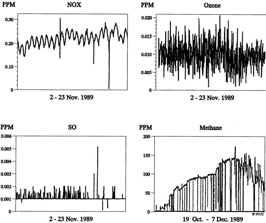
Figure VII.8: NO x , O 3 , SO 2 , CH 4 Levels During Test Module Human Closure (2 - 23 Nov.1989 - CH 4 including unmanned closure pre- and post-human habitation data) [3]
