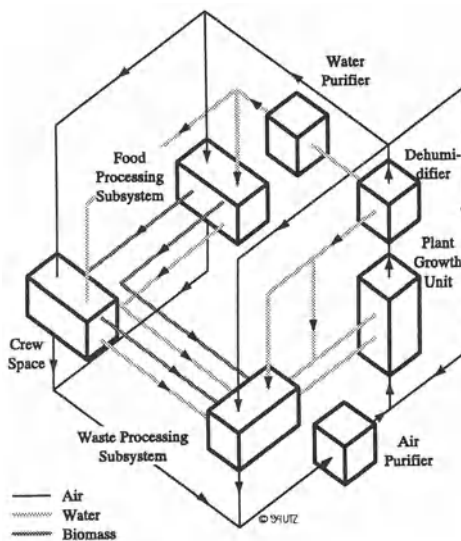
Figure VI.4: CELSS System Diagram [3]
