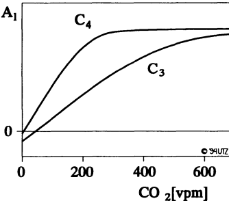
Figure VI.14: Leaf Assimilation as a Function of CO 2 Level [50]
