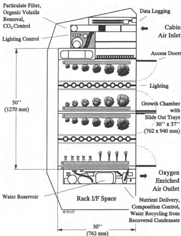
Figure VI.25: Salad Machine Design Concept [36]
