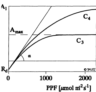
Figure VI.13: Leaf Assimilation as a Function of Light (PPF) [50]
