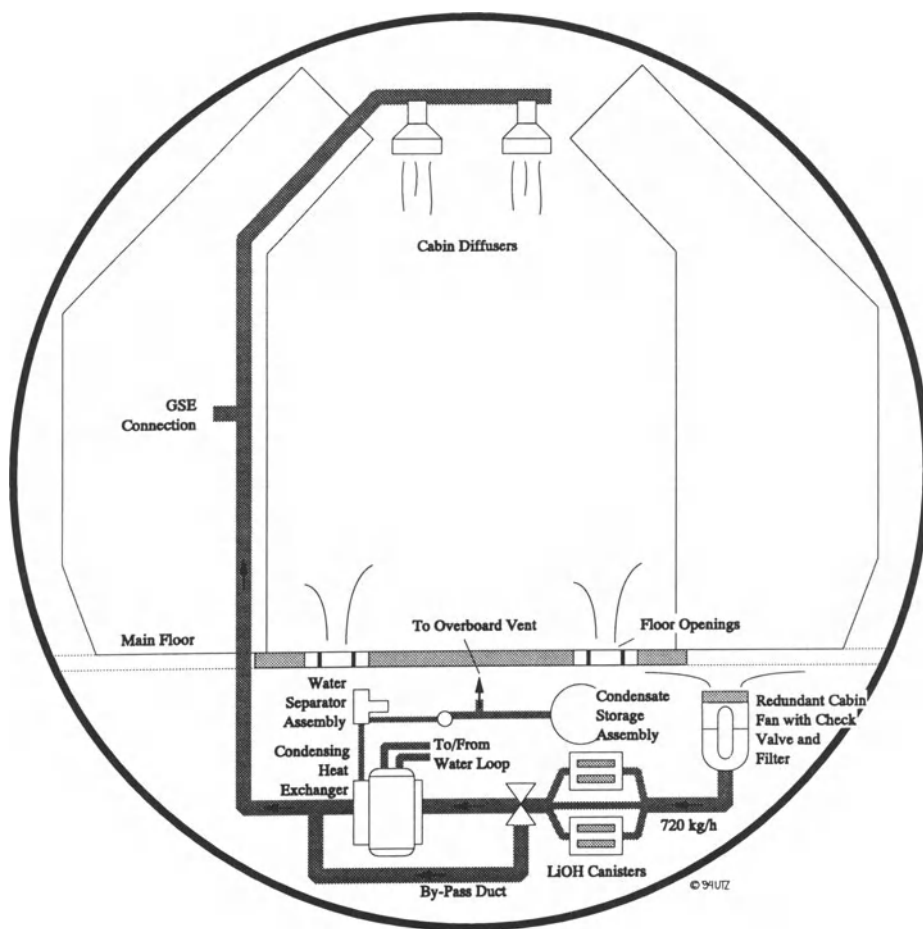
Figure V.1: Cabin Atmosphere Loop [29]
