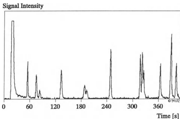
Figure V.16: Sample of a Gas Chromatogram [9]
