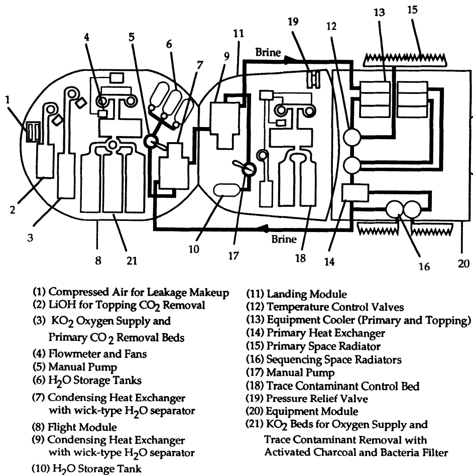
Figure IV.18: SOYUZ Life Support System [48]
