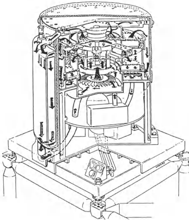
Figure VI.15: The EURECA Botany Facility [32]
