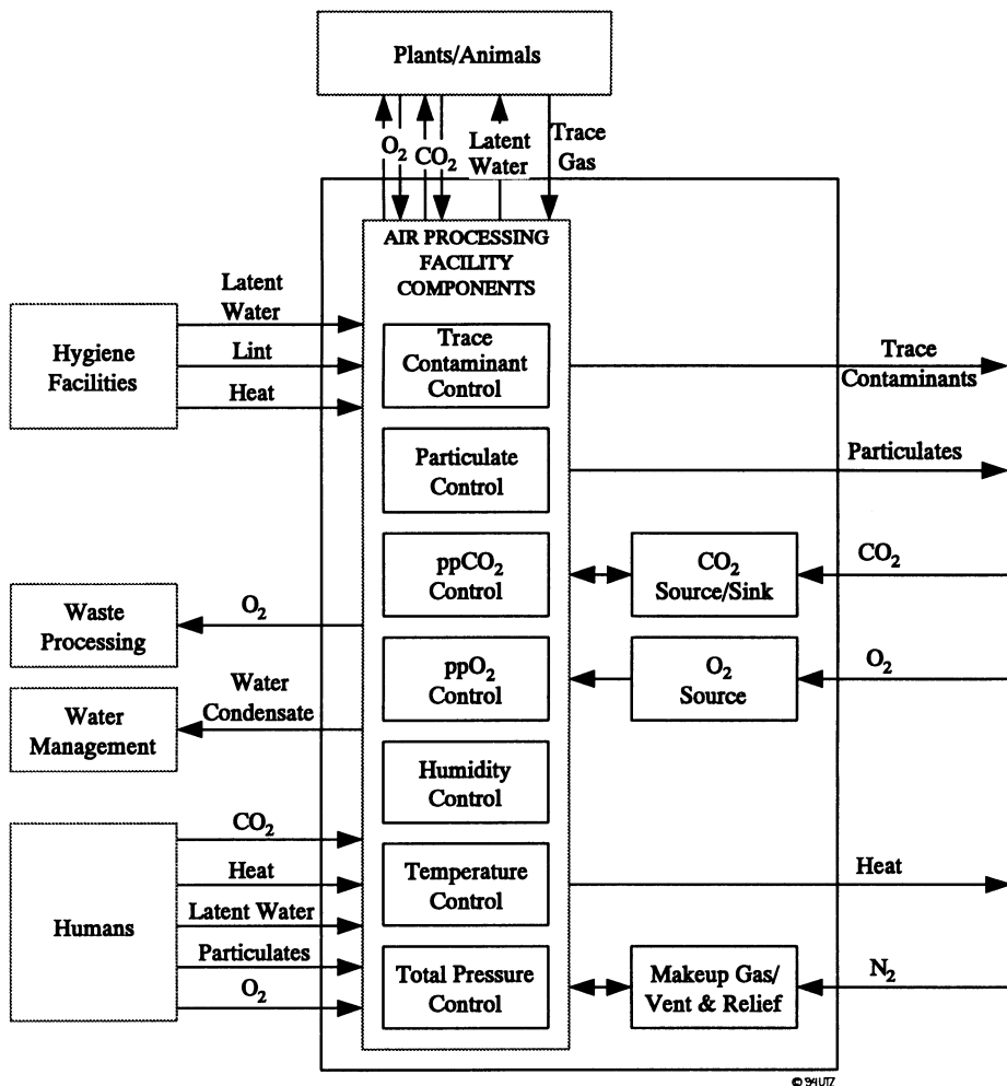
Figure IV.4: Atmosphere Revitalization Interfaces [13]
