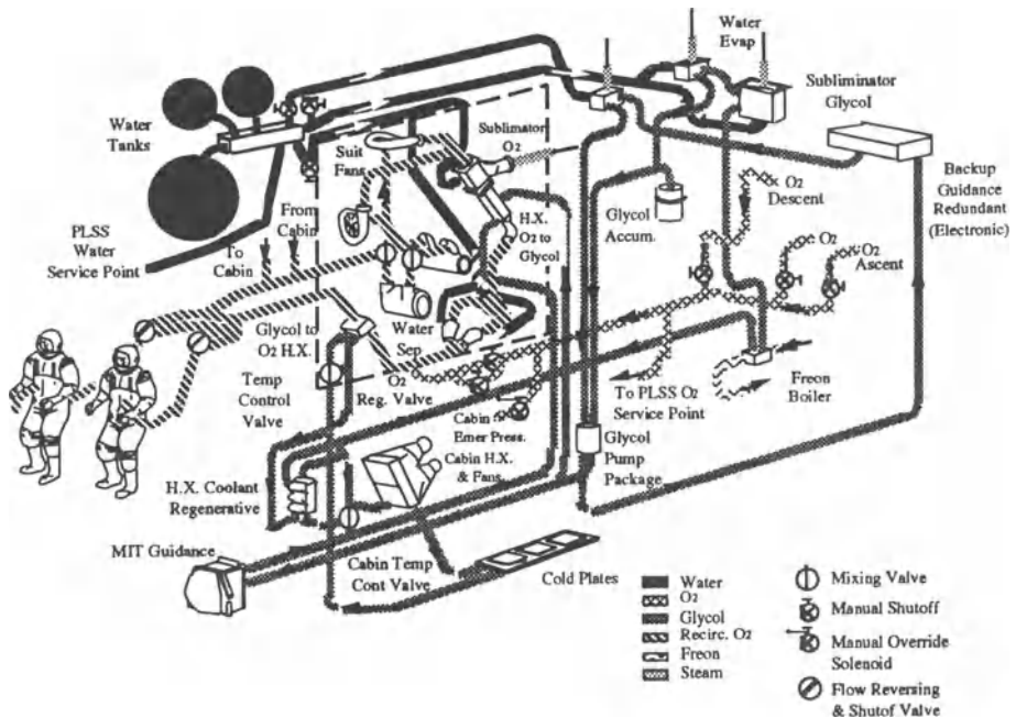
Figure IV.19: APOLLO Lunar Module ECLSS [48]
