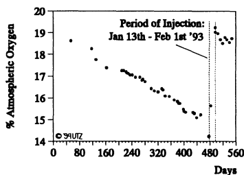
Figure VII.11: Oxygen Concentration (26 Sep '91 to 30 Mar '93) [10]
