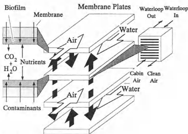
Figure VI.11: Principle of the Biological Air Filter [77]
