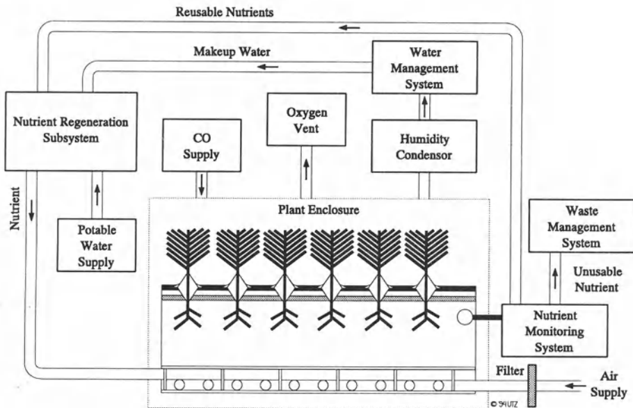
Figure VI.17: Aeroponics Plant Growth Tray [47]
