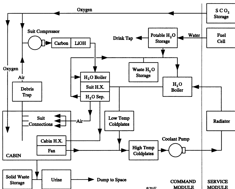
Figure IV.20: APOLLO CM ECLSS [48]
