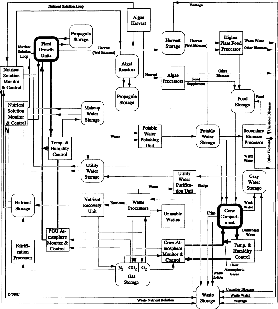
Figure VI.8: The CELSS Initial Reference Configuration [41]
