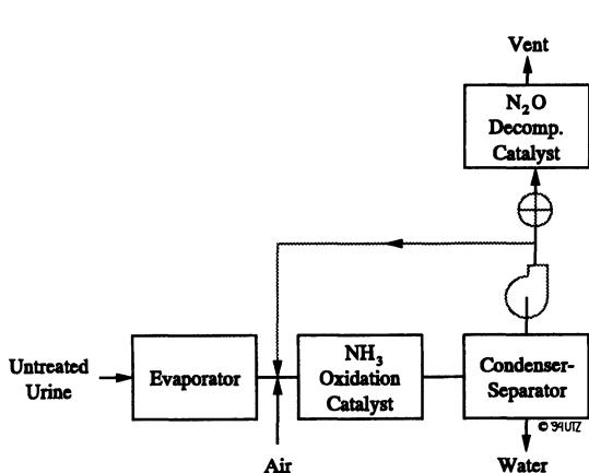
Figure V.24: VAPCAR Process [31]
