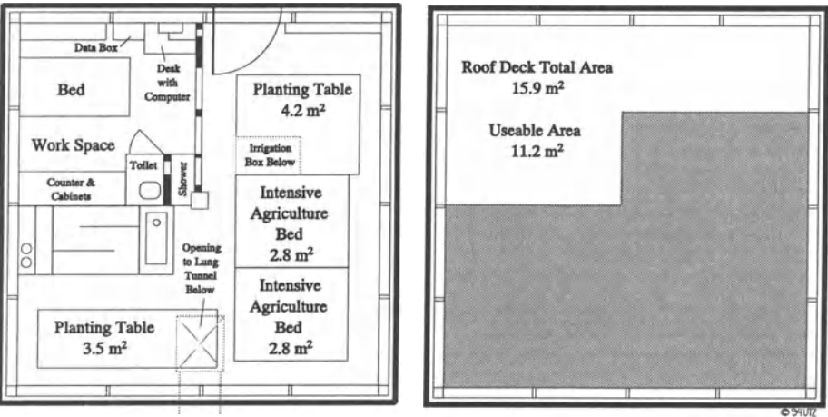
Figure VII.6: Biosphere 2 Test Module Floor Plan (Excluding Lung) [3]
