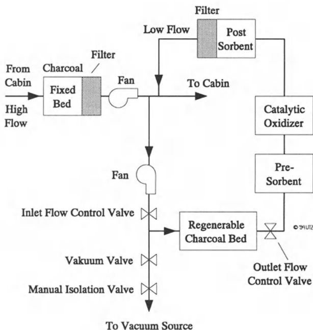
Figure V.12: Trace Contaminant Control Subsystem [31]
