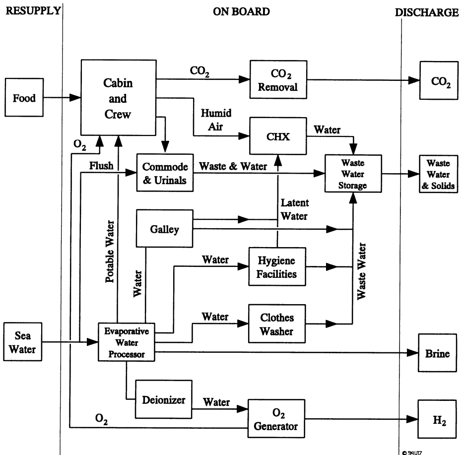
Figure IX.7: A Typical Submarine ECLSS [18]
