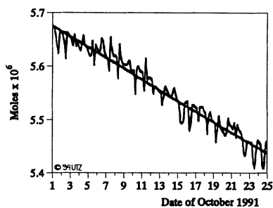
Figure VII.12: Progressive Dilution of SF_6 and He [4]
