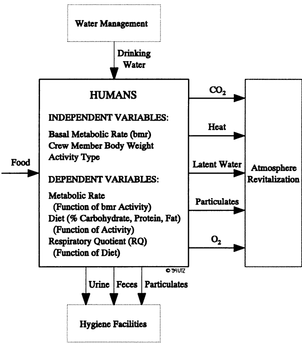
Figure IV.2: Human Interfaces in a LSS [13]
