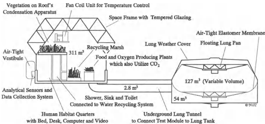
Figure VII.5: Biosphere 2 Test Module [3]
