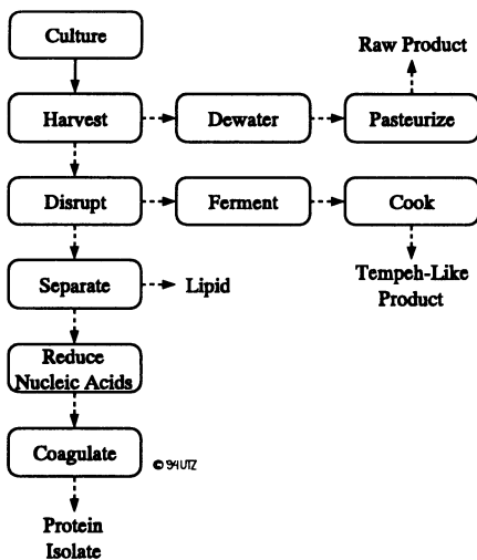
Figure VI.12: Alternatives for Food Production from Algae [4]
