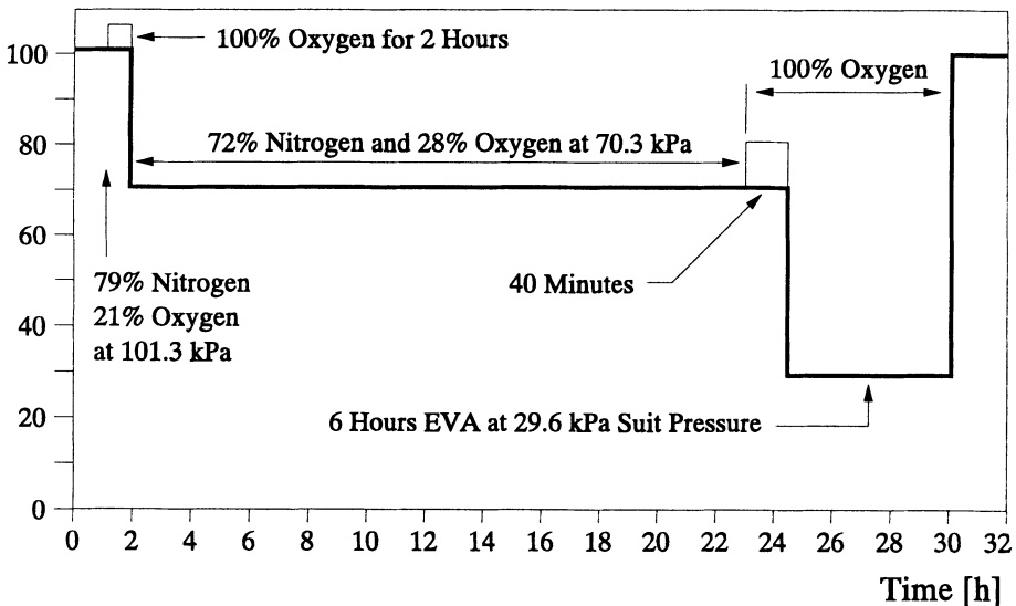
Figure IV.38: Prebreathing Protocol for EVAs from the Space Shuttle Orbiter (Staged Compression) [24]
