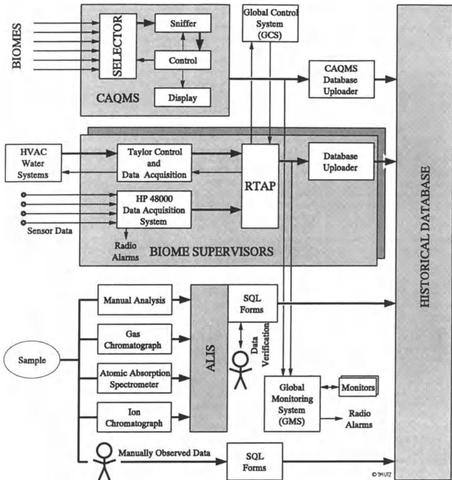
Figure VII.4: Data Flow and Monitoring [20]
