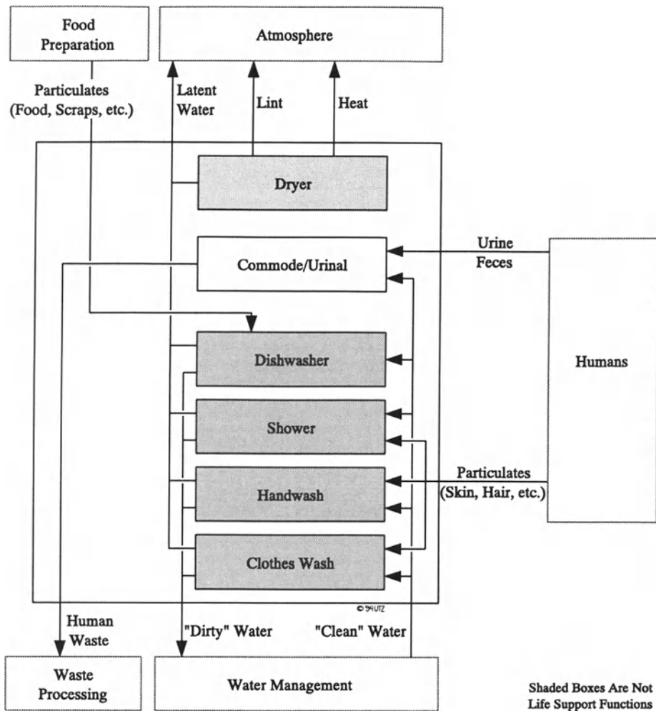
Figure IV.7: Personal Hygiene Facilities Interfaces [13]
