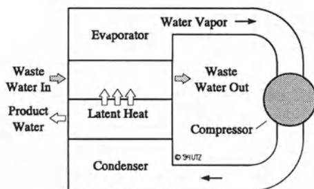
Figure V.23: VCD Process [12]
