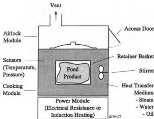
Figure VI.33: Fluid Immersion Cooker [18]
