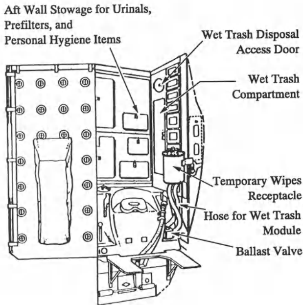
Figure V.30: The Space Shuttle Waste Management System [27]
