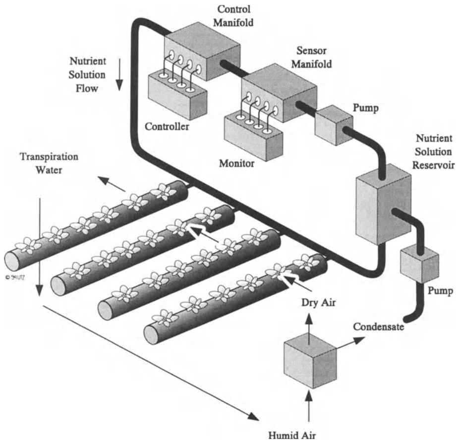
Figure VI.24: Sample Nutrient Supply System [48]
