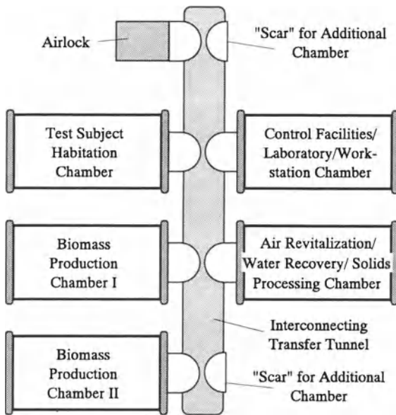
Figure IV.32: HRTF Conceptual Reference Configuration
