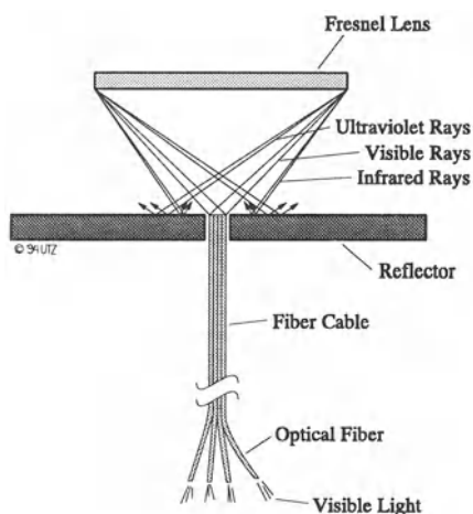
Figure VI.22: Principle of a Fresnel Lens [58]
