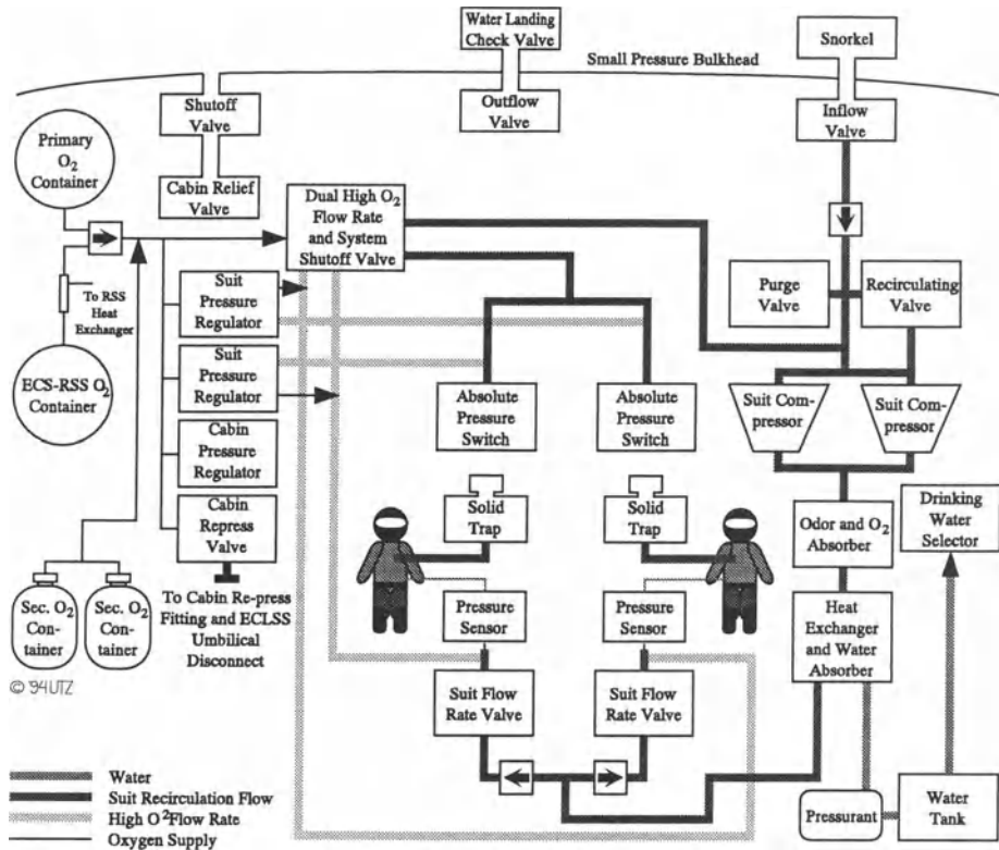
Figure IV.17: GEMINI ECLSS [48]
