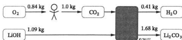
Figure V.5: LiOH Process
