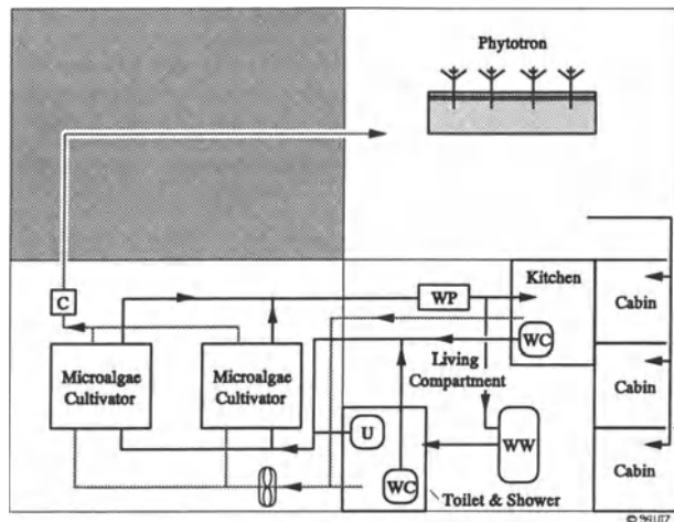
Figure IV.27: Second Stage of BIOS-3 [48]
