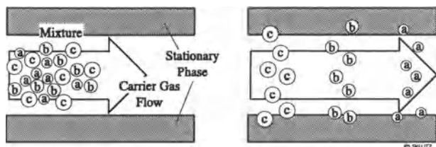
Figure V.15: Gas Chromatographic Separation [9]
