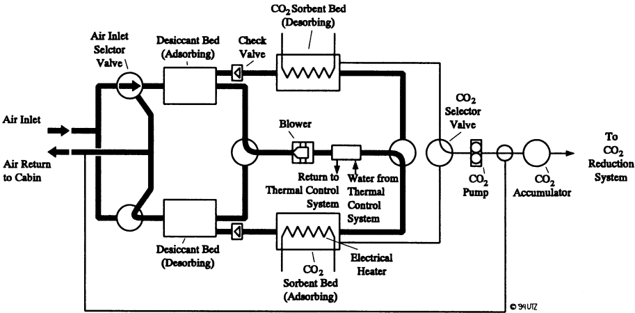
Figure V.2: 4-Bed Molecular Sieve [18]
