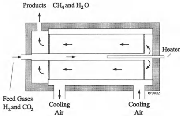
Figure V.7: Sabatier CO 2 Reduction Process [31]
