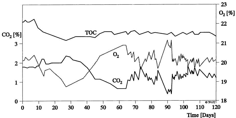
Figure IV.23: Dynamics of \text{CO}_2 , \text{O}_2 , and TOC in the Atmosphere of BIOS-3 [34]
