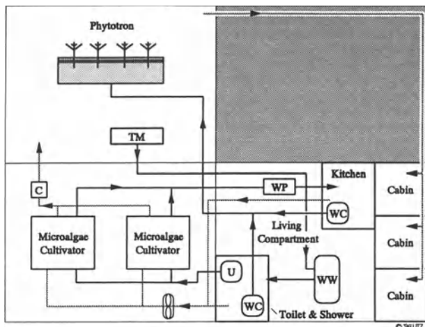
Figure IV.27: Second Stage of BIOS-3 [48]
