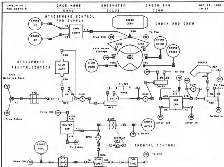
Figure IV.15: CASE/A Model of a Vehicle ECLSS [48]
