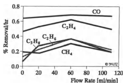
Figure IX.4: Reducing the Atmospheric Concentration of Organic Compounds by a SBR [6]
