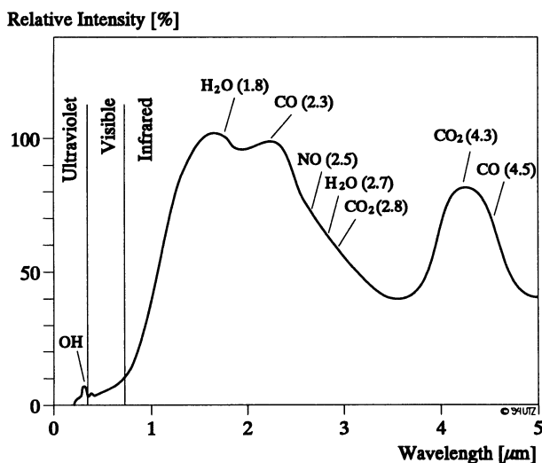
Figure V.22: Radiant Energy Emitted from a Typical Hydrocarbon Fire [10]
