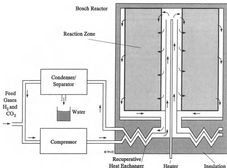
Figure V.6: Bosch \text{CO}_2 Reduction Process [11]
