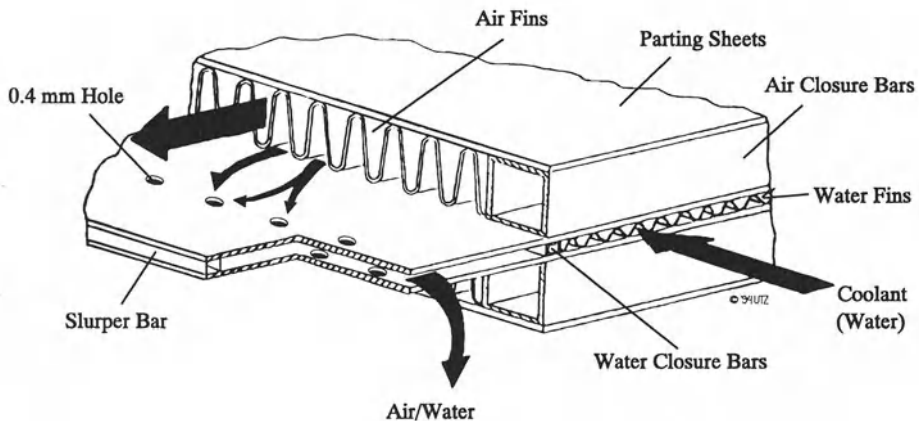
Figure V.13: The Function of a CHX Slurper [20]
