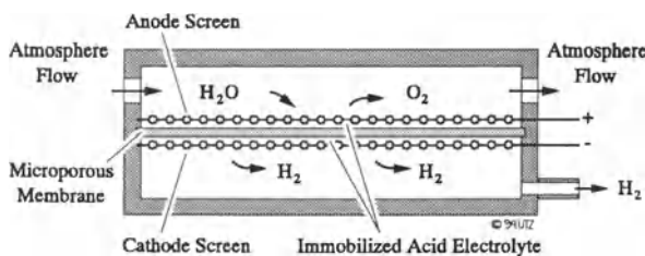
Figure V.11: Water Vapor Electrolysis [29]
