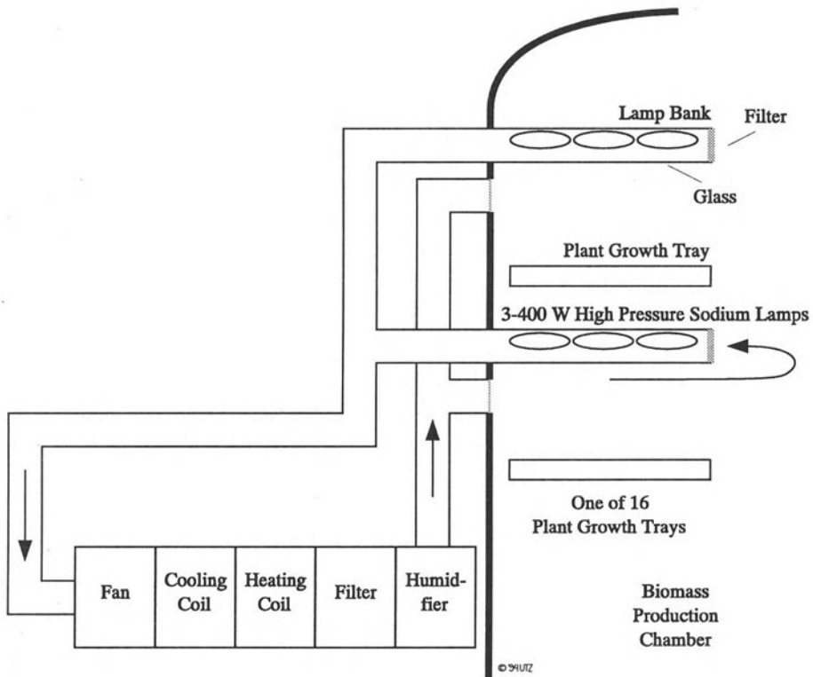
Figure IV.30: Cross-section of the Upper Half of the Biomass Production Chamber [47]
