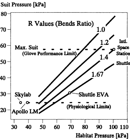
Figure IV.36: Cabin Pressure vs. Suit Pressure as Influenced by Bends Ratio [20]
