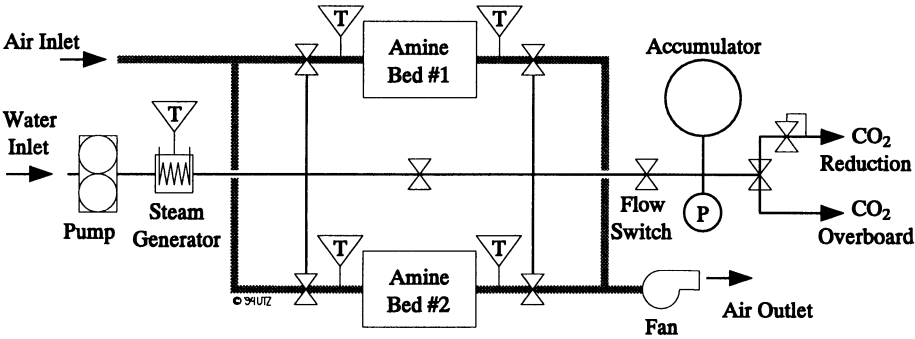
Figure V.3: 2-Bed, Solid-Amine-Resin, SAWD [31]
