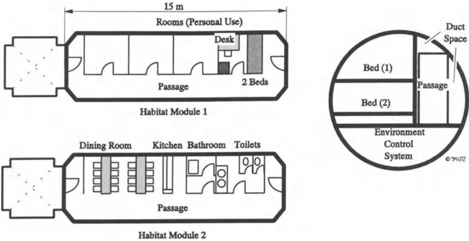
Figure VIII.4: Lunar Base Habitat Modules [9]
