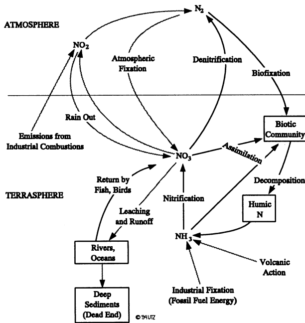
Figure II.15: The Nitrogen Cycle [8]
