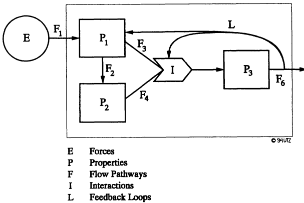
Figure II.3: Main Components of an Ecological System [8]
