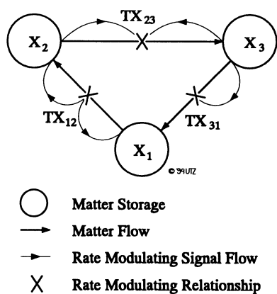
Figure VI.9: Flow of Carbon in a Small Ecosystem [35]
