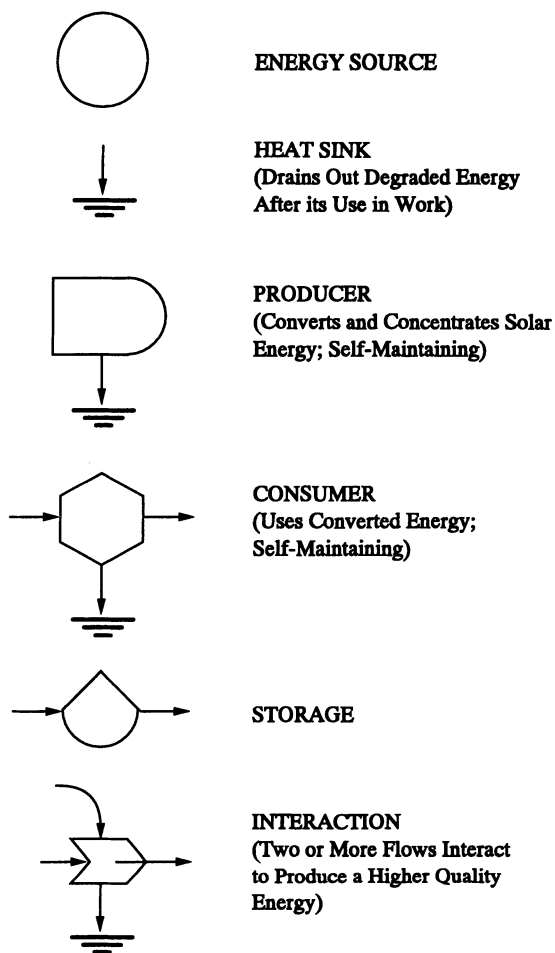
Figure 11.4: H.T. Odum's "Energy Language" Symbols [8]
