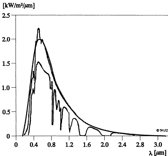
Figure II.2: Solar Spectra above and below the Atmosphere
