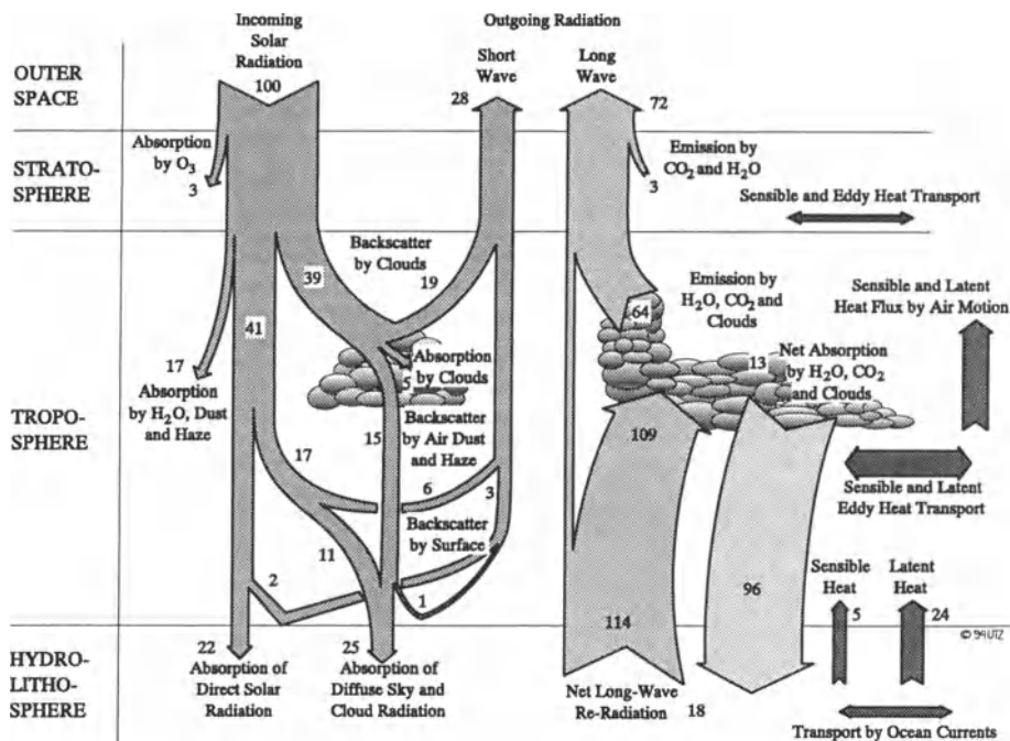
Figure 11.7: Distribution of Absorbed Solar Energy in the Earth System [12]
