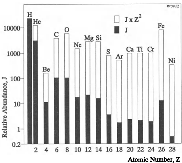
Figure III.4: Relative Abundances of Even-Numbered GCR Rays [20]
