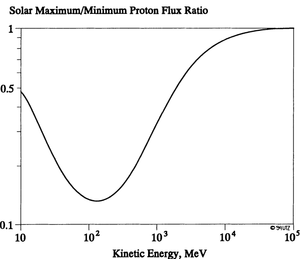
Figure III.5: GCR Proton Flux Reduction Factors at Solar Maximum Conditions [25]
