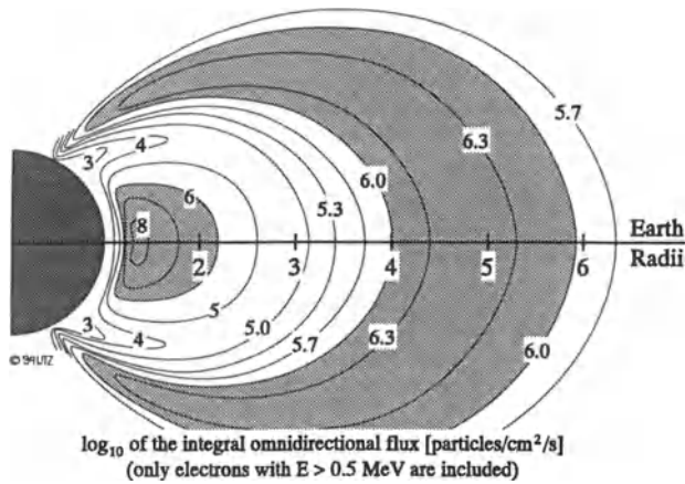
Figure III.7: The Van Allen Belts [30]
