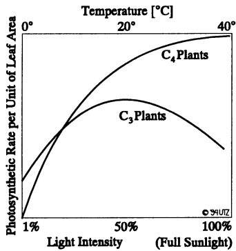
Figure 11.10: Photosynthetic Responses of C 3 and C 4 Plants [8]
