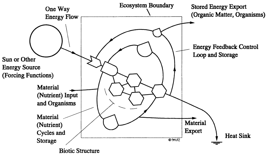
Figure II.5: A Functional Diagram of an Ecosystem [8]
