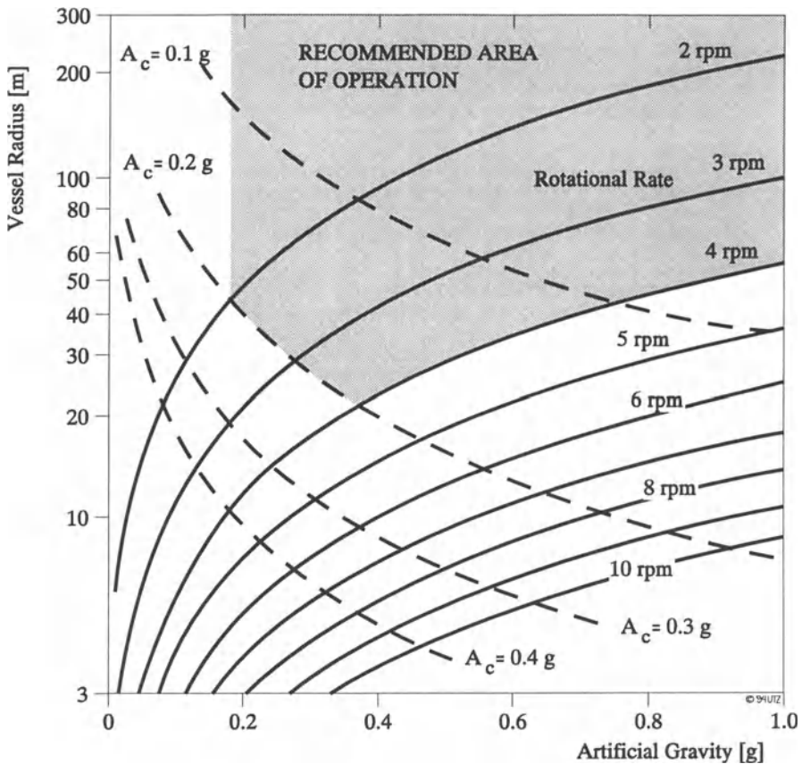
Figure III.14: The Coriolis Acceleration A_c [30]
