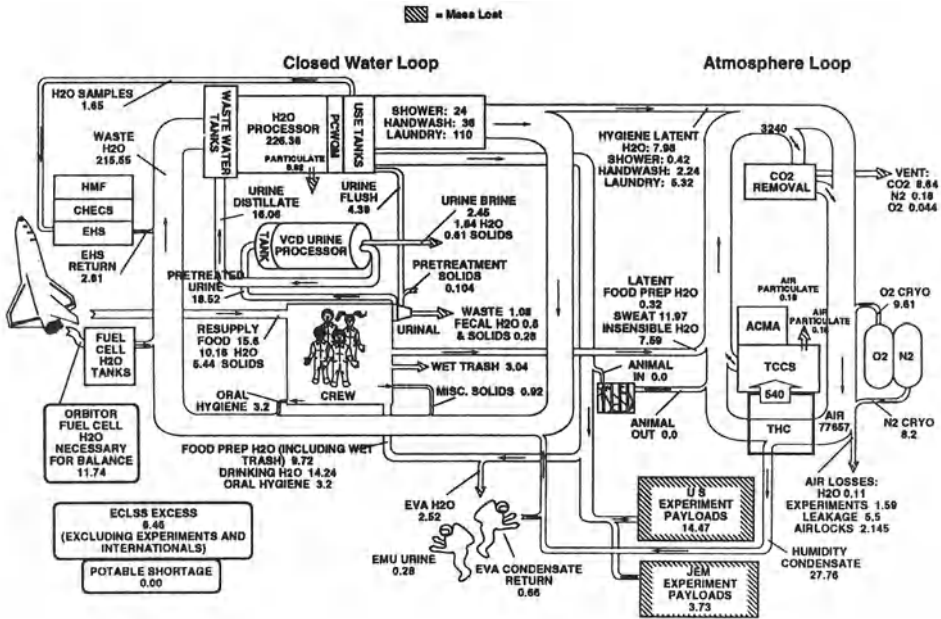
Figure IV.12: Mass Balance for a Space Station (Values in [lb/day]) [25]
