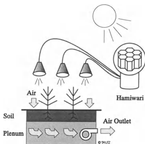
Figure IX.3: Soil Bed Reactor [6]
