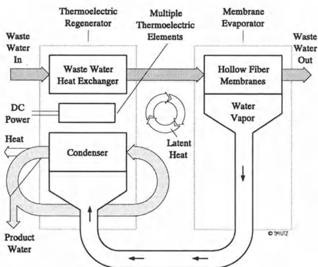
Figure V.25: TIMES Process [31]
