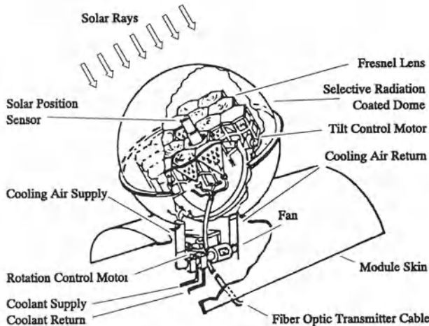
Figure VI.21: Hamiwari Fiber Optic Light Collection System [47]
