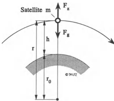
Figure III.12: Forces on a Satellite in Orbit
