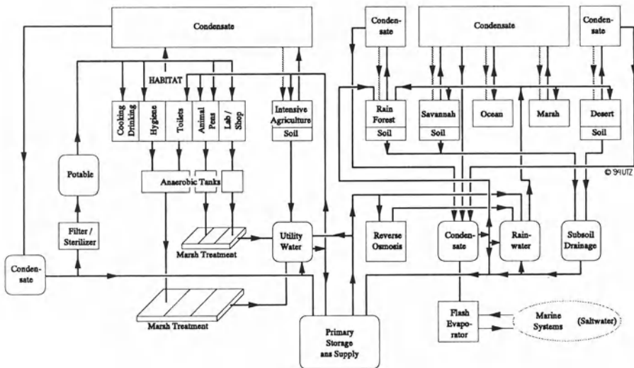
Figure VII.2: Biosphere 2 Freshwater Systems [5]
