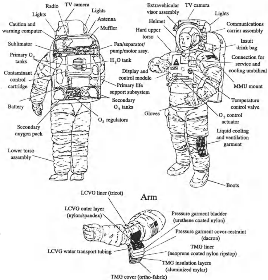
Figure IV.34: The Space Shuttle Extra-Vehicular Mobility Unit [29]
