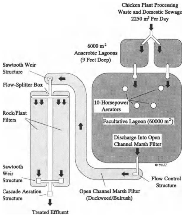
Figure IX.5: Example of an Artificial Waste Water Treatment System [20]
