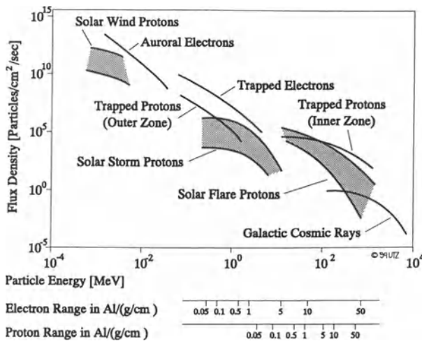
Figure III.2: Radiation in Free Space [20]
