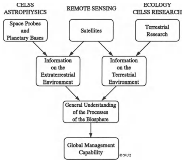
Figure IX.2: Synergistic Approach towards the Understanding of the Biosphere
