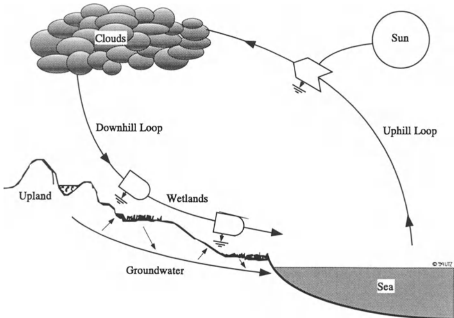
Figure II.14: The Hydrological Cycle [8]
