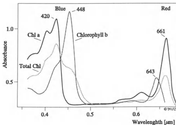
Figure VI.20: Light Absorption Spectra of Plants [75]
