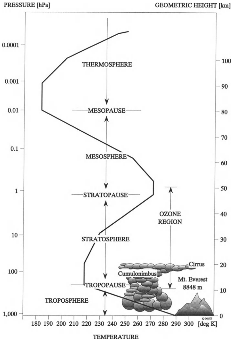
Figure II.1: Temperature, Pressure, and Density Distribution of Earth's Atmosphere [12]
