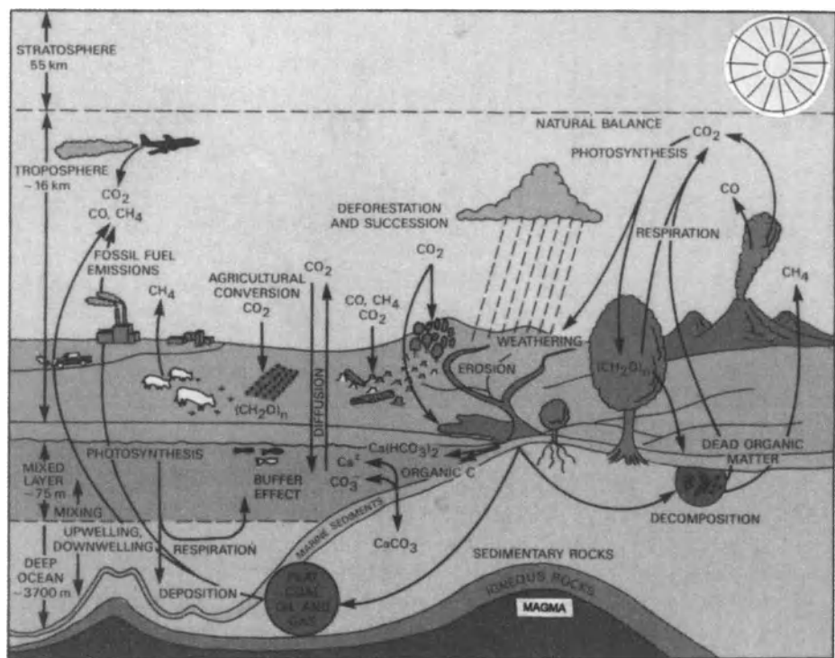
Figure II.16: The Carbon Cycle [12]
