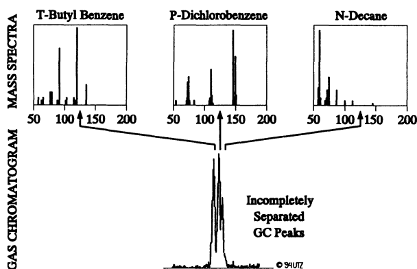
Figure V.17: Mass Spectroscopy Applied to an Incompletely Separated Gas Chromatograph Peak Group [9]
