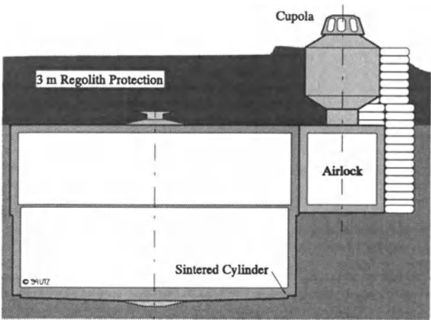
Figure VIII.5: The Lunar Habitat as designed by the University of Houston [3]
