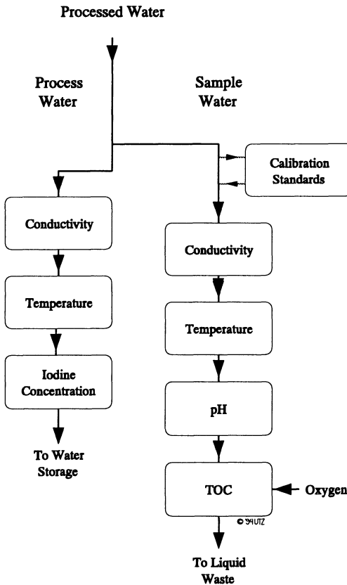
Figure V.29: Water Quality Monitoring Equipment [29]
