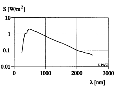
Figure III.1: Electromagnetic Spectrum of the Sun
