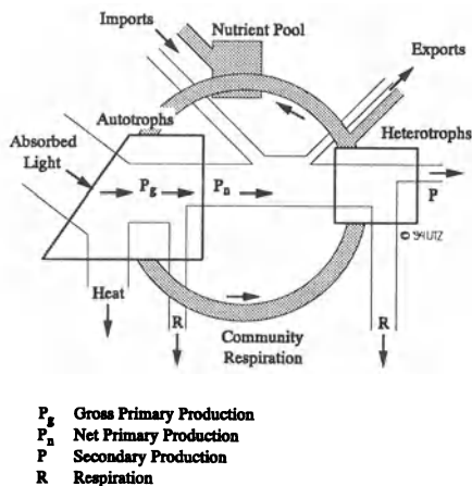
Figure II.12: A Biogeochemical Cycle [8]
