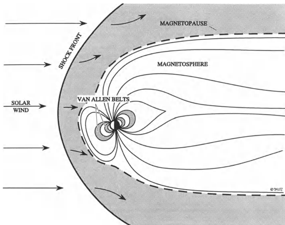
Figure III.15: The Magnetosphere of Earth [26]
