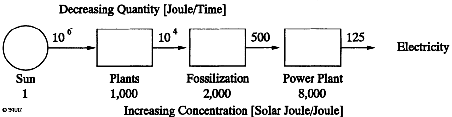
Figure II.9: Food Chain and Electric Energy Chain [8]
