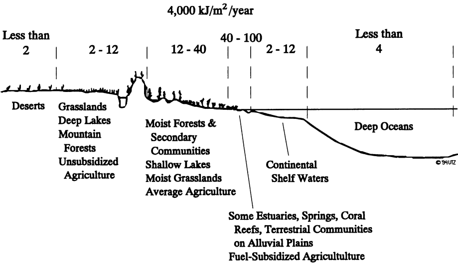
Figure 11.11: World Distribution of Primary Production (in [kJ/m 2 /year]) [8]
