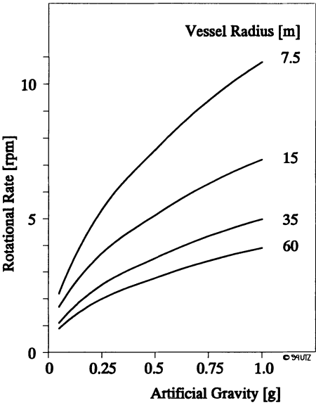
Figure III.13: Induced Gravity
