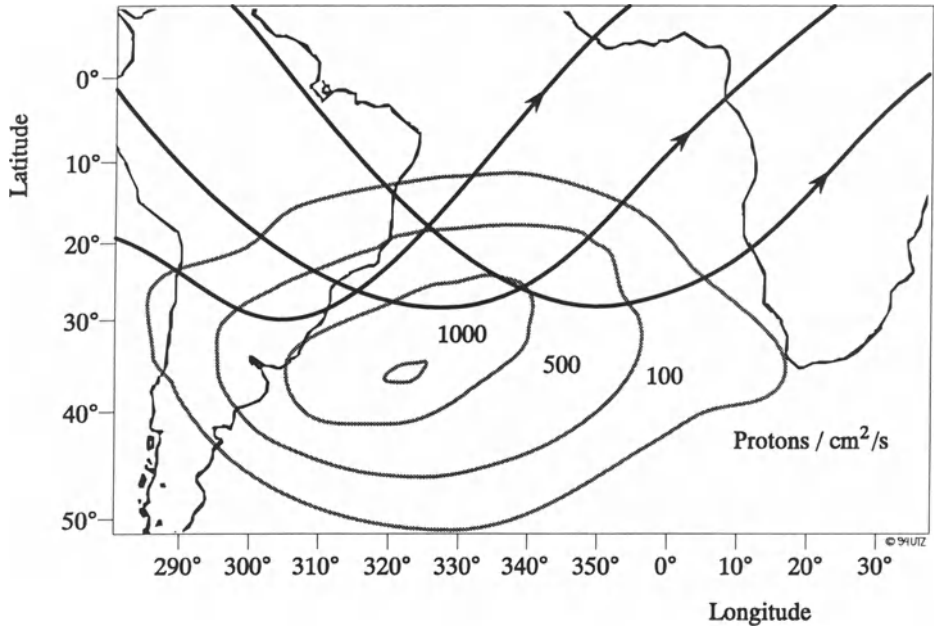
Figure III.8: The South Atlantic Anomaly [11]
