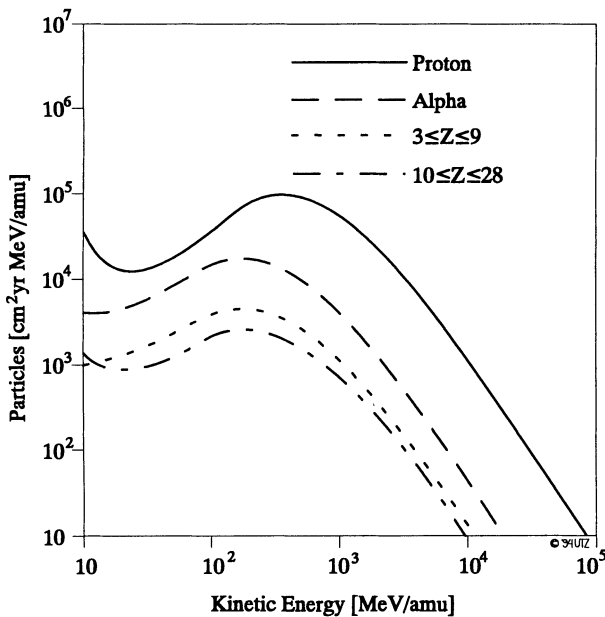
Figure III.6: Flux vs. Energy Distribution for GCR Ions During Solar Minimum [24]
