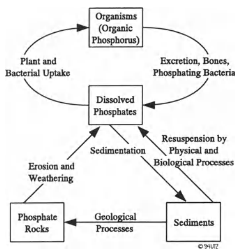
Figure II.17: The Phosphorous Cycle [8]
