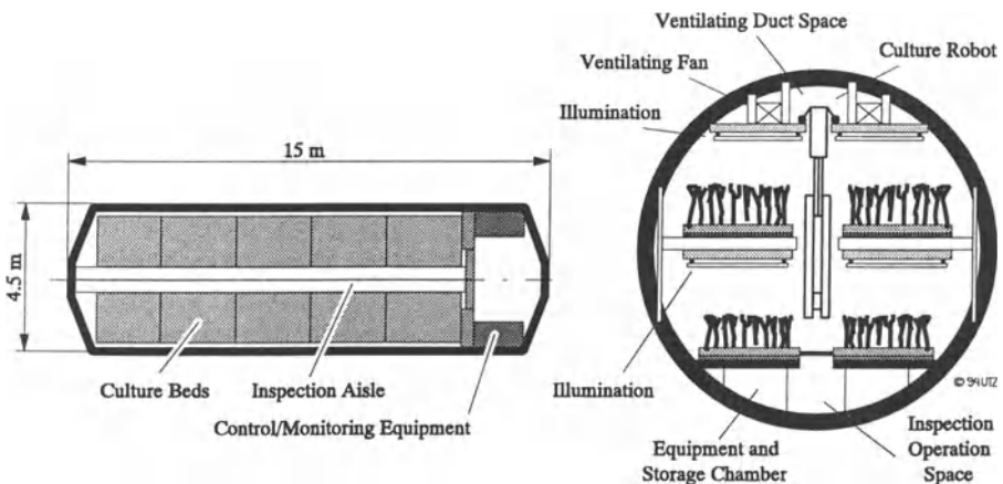
Figure VIII.3: Lunar Base Plantation Module [9]
