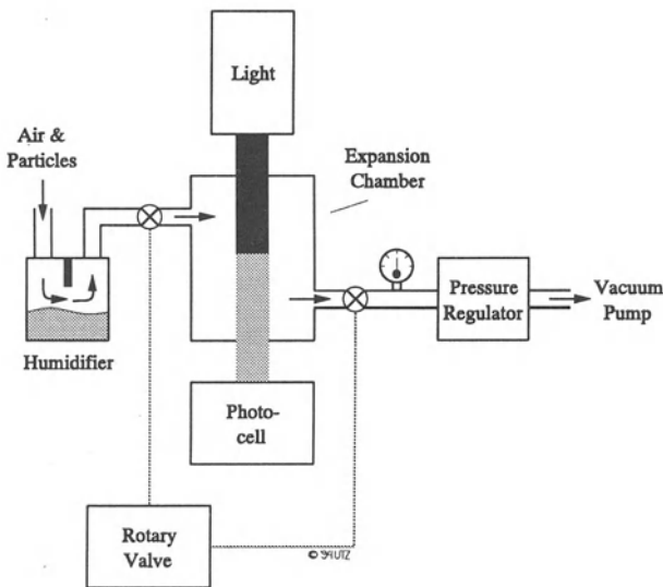
Figure V.20: Condensation Nuclei Counter [10]
