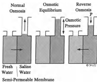
Figure V.27: Reverse Osmosis [31]
