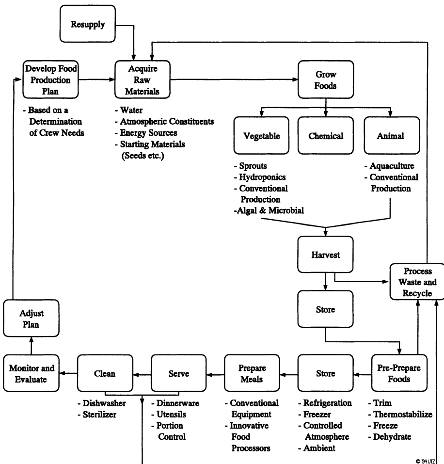
Figure VI.30: Food Production and Service System Components [18]
