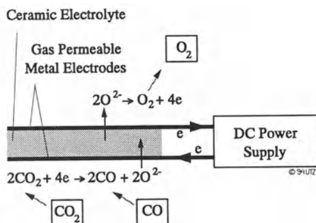
Figure V.8: Solid Electrolyte CO 2 Electrolysis Cell [31]
