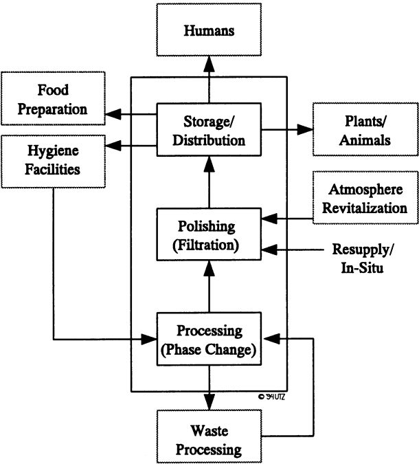
Figure IV.5: Water Management Interfaces [7]
