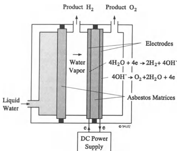
Figure V.9: SFWE Cell [30]
