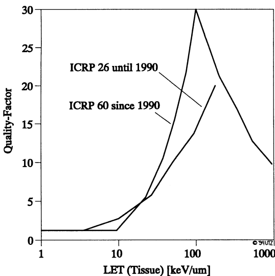
Figure III.9: Quality Factor vs. LET [29]
