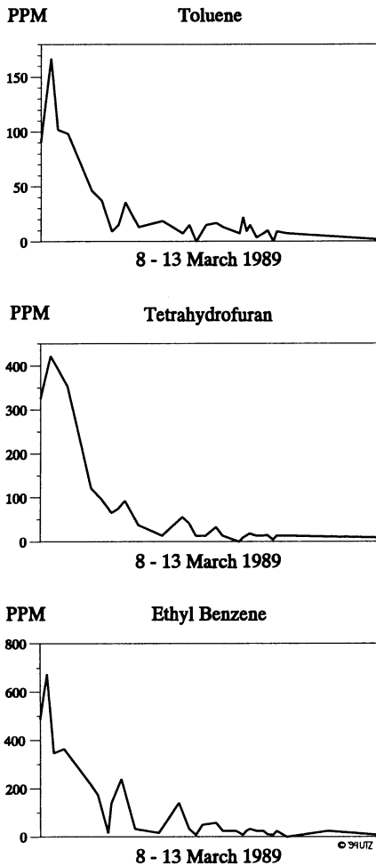
Figure VII.7: Technogenic Gases in the Test Module Air in February / March 1989 [3]
