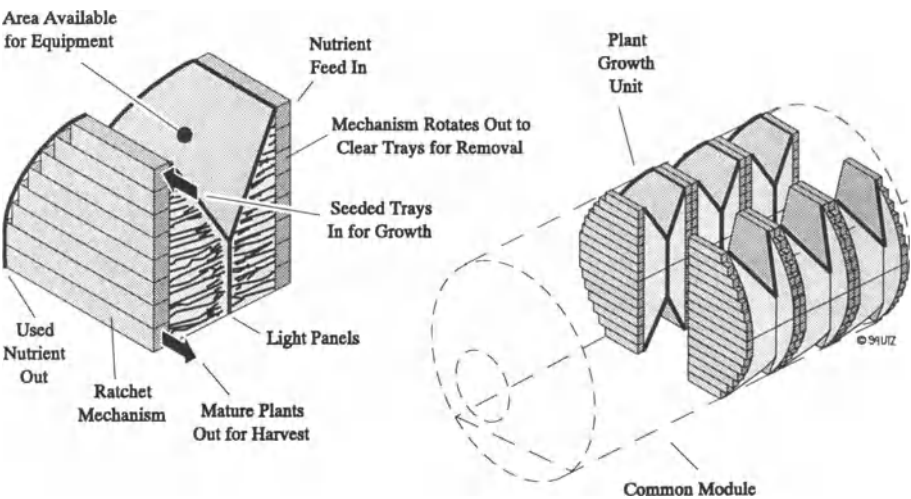
Figure VI.28: The Accordion Tray Stack Concept [48]
