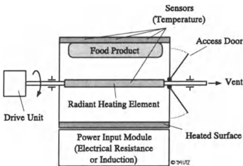
Figure VI.35: Direct Contact and/or Radiant Heating Surface Cooking Processor [18]
