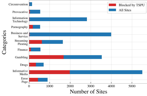
Figure 7: Domain Categories. Excluding (1398+2680) domains that failed TCP, or empty/unparseable HTML responses. Error page includes geoblocked or parking pages.
