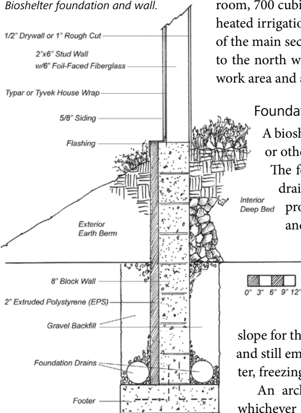
Bioshelter foundation and wall.
