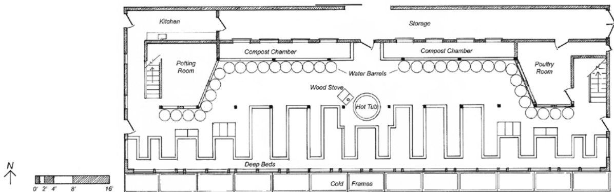
Bioshelter floor plan.
