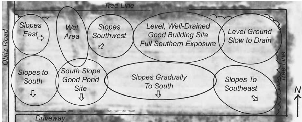
Bubble map of topography and main features.
