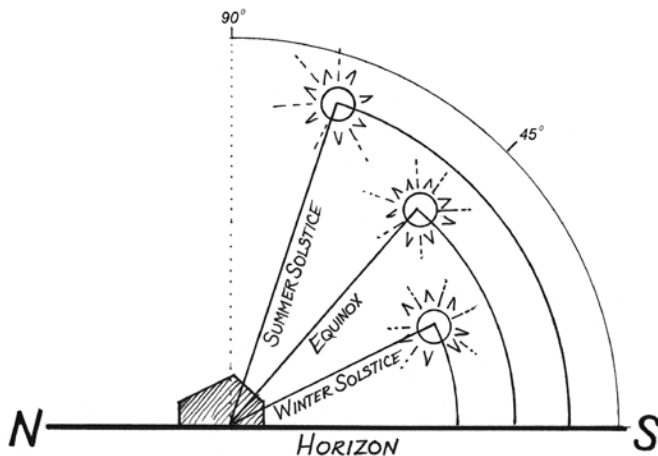
Solar angle (at solar noon) above the horizon at Solstices and Equinoxes for 45 degrees north latitude as example.
