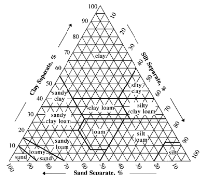
Soil triangle.
