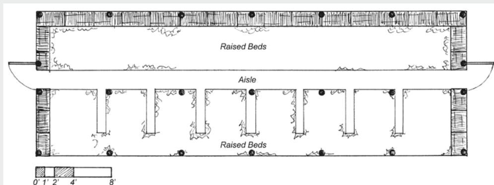
Bale shelter section and bale plan.
