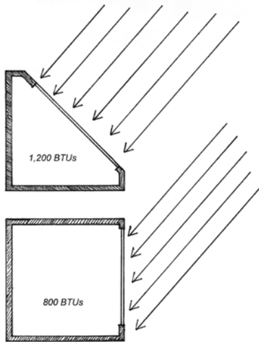
Expected average Btu per square foot at 90 degrees and 45 degrees.
