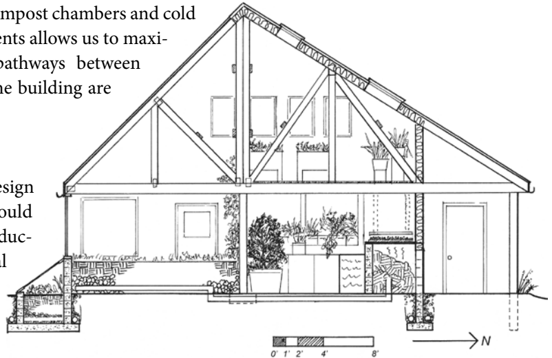
Bioshelter cross section.
