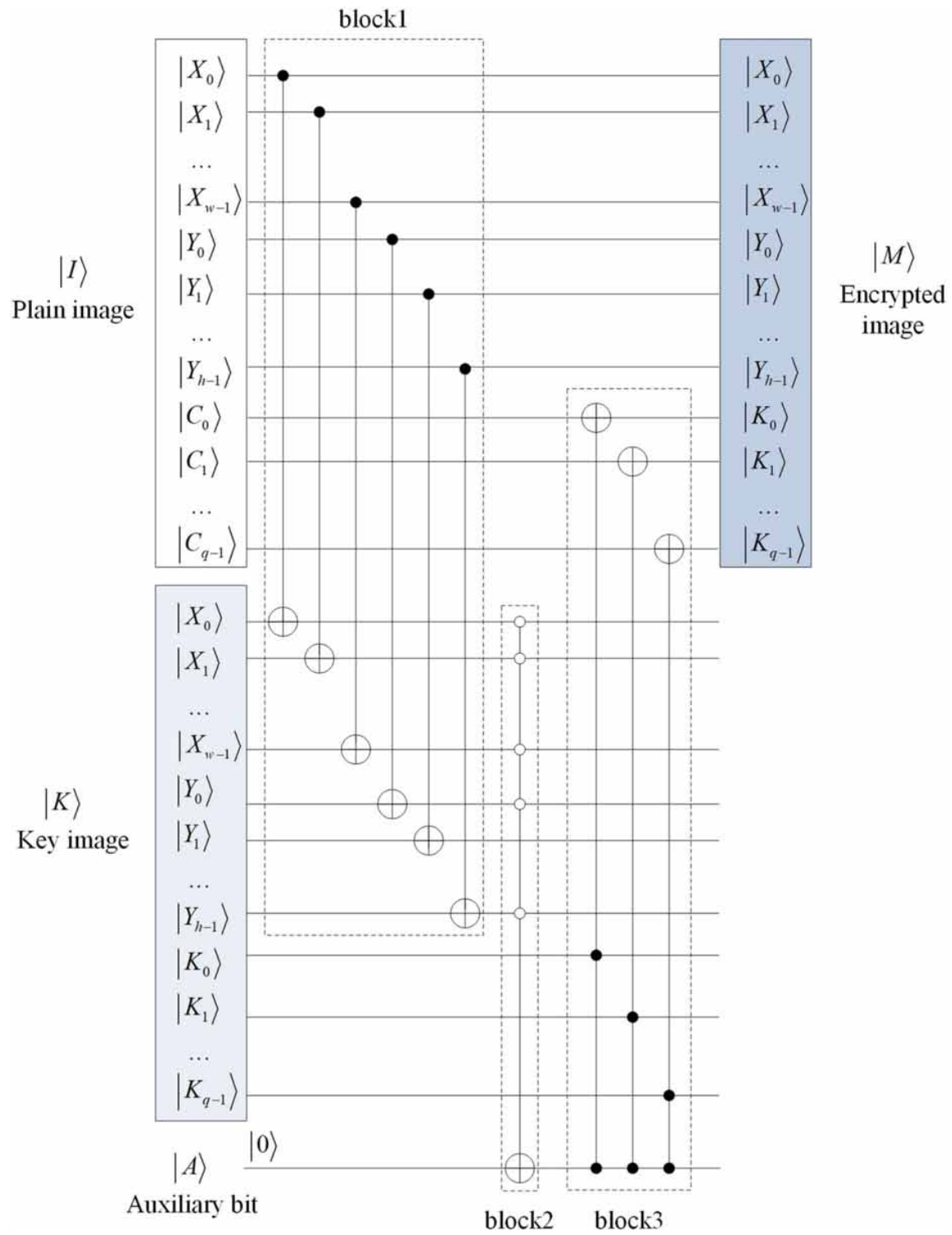
Figure 17. XOR Representation of Quantum Key Image
