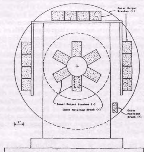
Figure 2 - Sunburst Homopolar Generator - Output (Brush) End View
