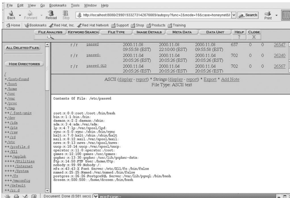
FIGURE 18.6 Viewing a Linux system using the Sleuth Kit and Autopsy Forensic Browser.
