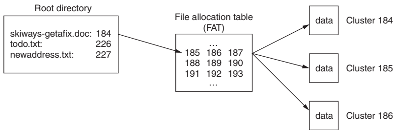
FIGURE 17.1 Root directory (skyways-getafix.doc, starts in cluster 184) → FAT → data in clusters 184-225 (42 clusters × 512 bytes/clusters = 21,504 bytes).
