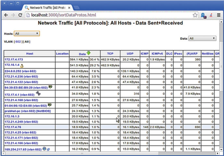
Fig. 4.19 Ntop: network traffic statistics
