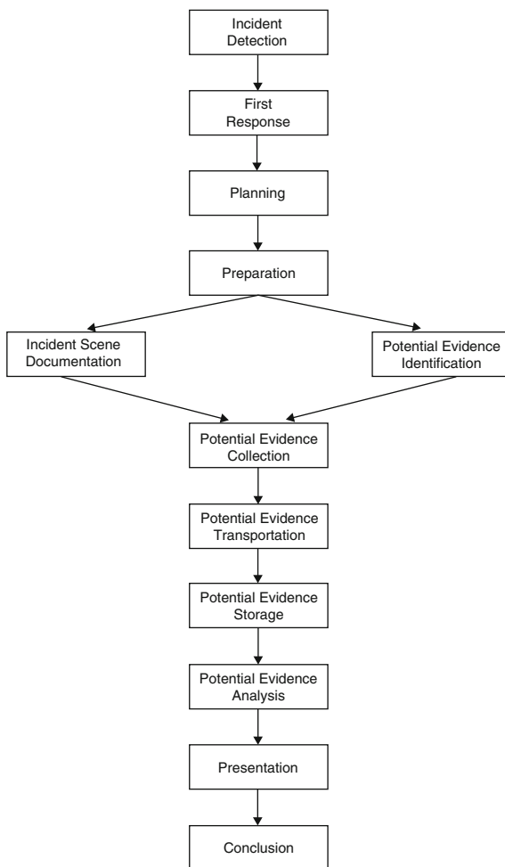
Fig. 9.3 Harmonized digital forensic investigation process model
