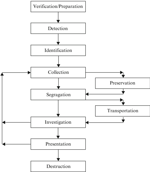
Fig. 10.2 Generic process model of cloud forensics
