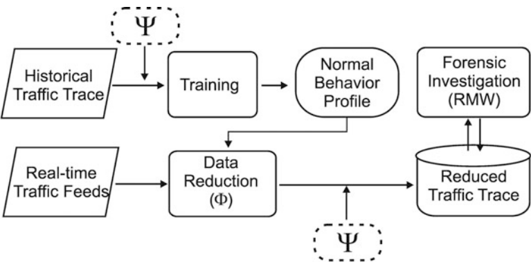
Fig. 2.19 Scalable network forensic mechanism
