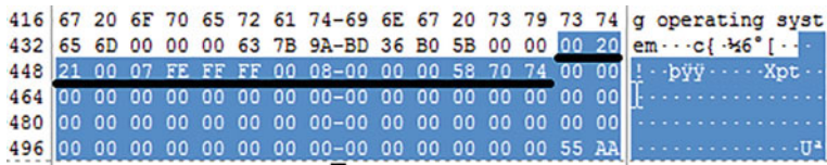
Fig. 8.5 Partition table entry viewed in FTK imager
