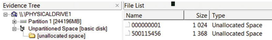
Fig. 8.4 Unallocated space shown in FTK imager
