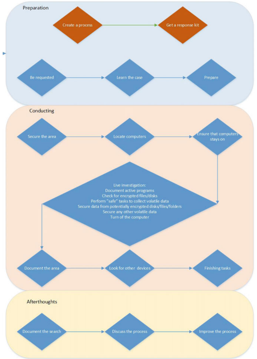
Fig. 4.1 Live investigation process
