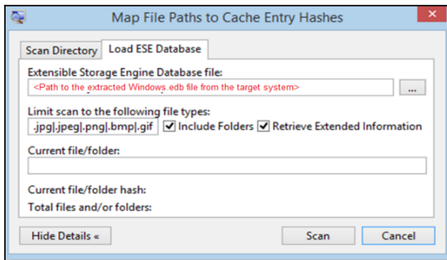
Figure 8: Mapping Thumbcache files to location
