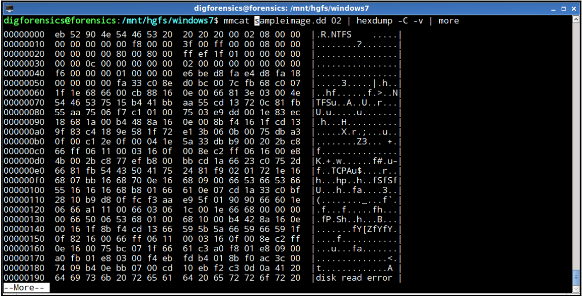
The mmcat tool
