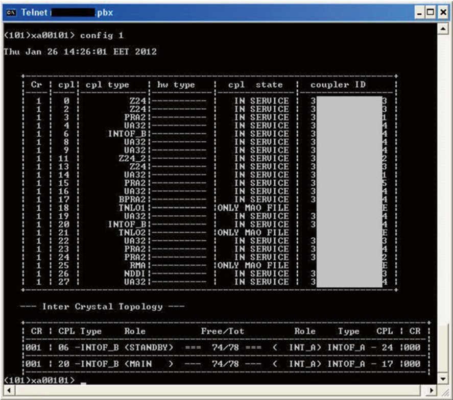
Fig. 3.10 List of boards (hardware configuration) installed in a PBX and their status
