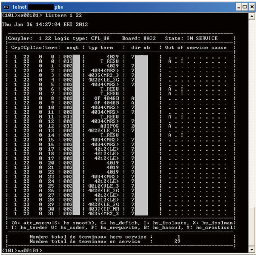
Fig. 3.12 List of sets and their numbers ( masked ) connected in a voice board
