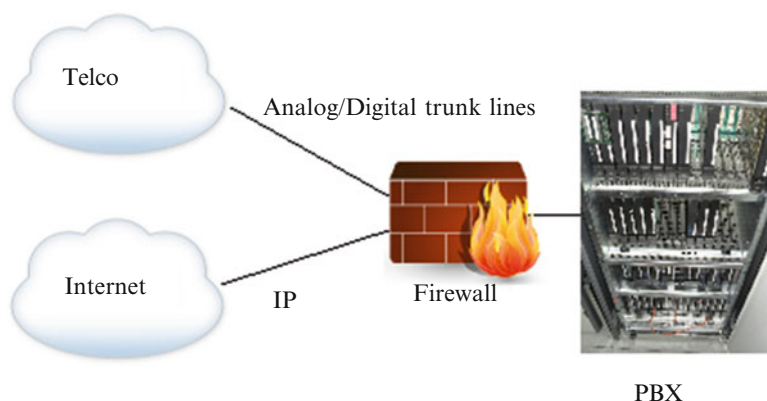
Fig. 4.4 PBX firewall
