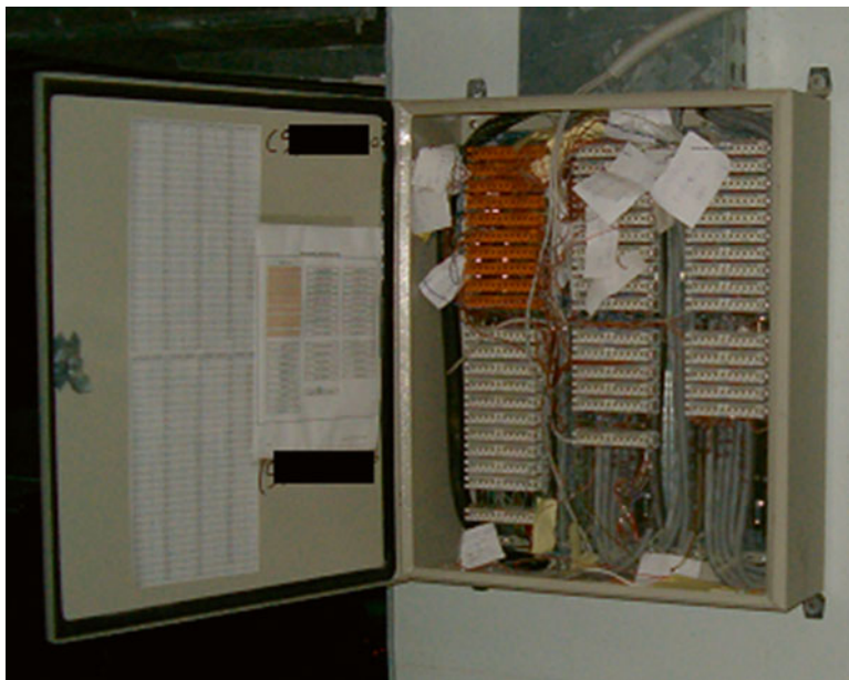
Fig. 3.5 Medium size office main distribution frame and CPE
