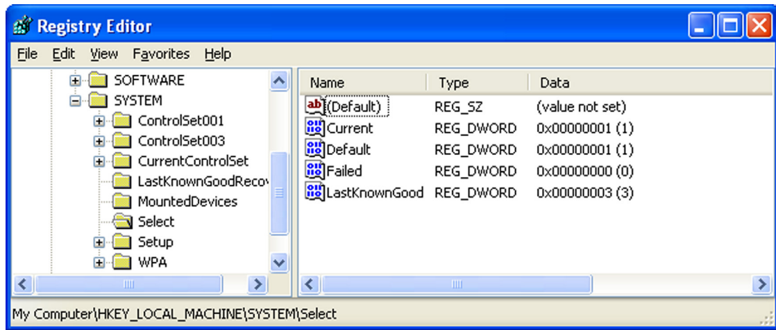
Figure 1.1 Registry Editor.
