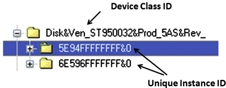
Figure 3.9 USB device in the Enum\USBStor key.
