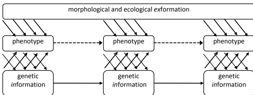
Figure 9: Flux of formation , including information and exformation, according to the points (1.) to (5.) of this section. The phenotype is not only determined by genic information , but by exformation as well. Even if one accepts the central dogma of microbiology, the resulting phenotype has itself a certain influence on the genotype, interpreting the information and influencing what is transcribed (dotted arrows). Also the transfer of cytoplasm from phenotype to phenotype is indicated (dashed arrows). Moreover, not depicted here, the phenotype constrains and directs the viable evolutionary pathways (5.).
