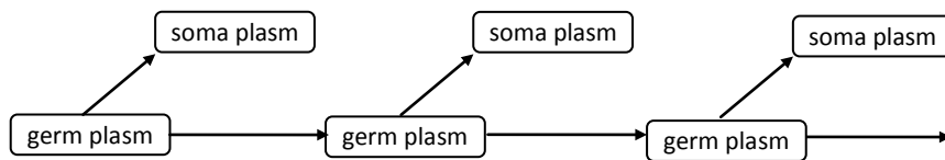
Figure 2: Flux of information in Weismann's Keimplasmatheorie .
