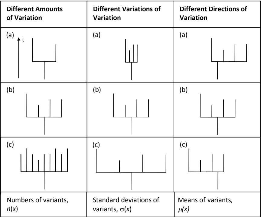
Figure 13: Simplified visualisation of types of variation of informational lines or their phenotypic expression. (Here we are only concerned with variation in the sense of evolutionary change.) In the diagram only one generation of reproductive entities (e. g. complex genes, organisms or species) is shown. The vertical dimension in each diagram is time. The horizontal dimension is something like genetic difference or, differently, distance in the morphospace. Although making some distinctions, naturally, this visualisation still makes simplifying assumptions. In regard to species it could, for example, be disputed if the genotypic variance were to emerge suddenly, which is indicated by the sharp edged corners of the trees. Also the emergence of new lines does not need to take place only when old lines have declined.
