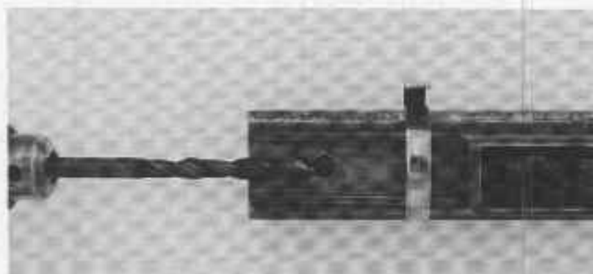
PHOTO 7: Drill through lower receiver bolt holes and into upper receiver tube.
