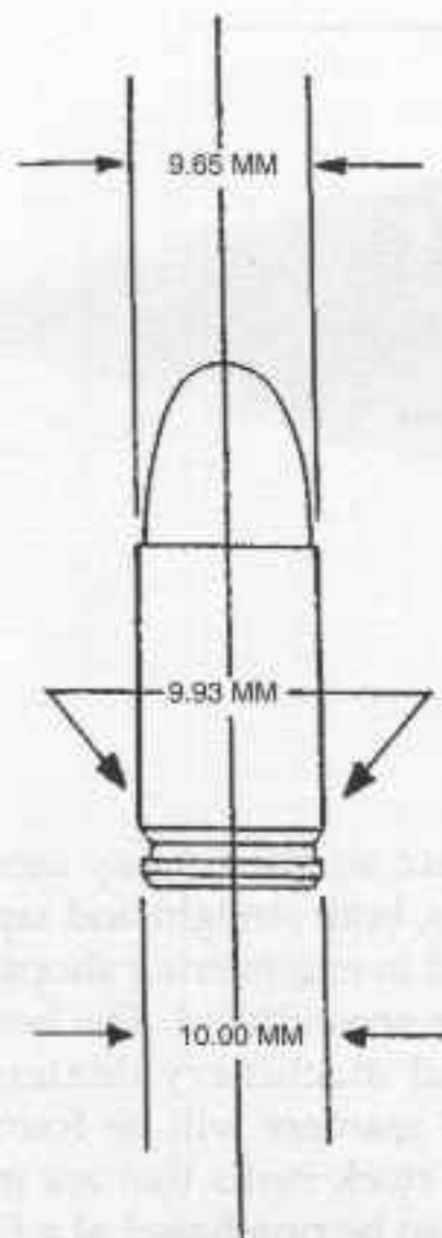
THIS CARTRIDGE CASE TAPERS FROM 9.93 MM TO 9.65 MM. THE BASE OF THE CASE IS 10 MM IN DIAMETER.
