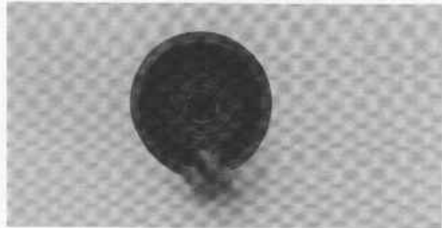
PHOTO 21: Firing pin rod fitted inside spring pin. The top of the rod should be 2.5 mm below the end of the spring pin.
