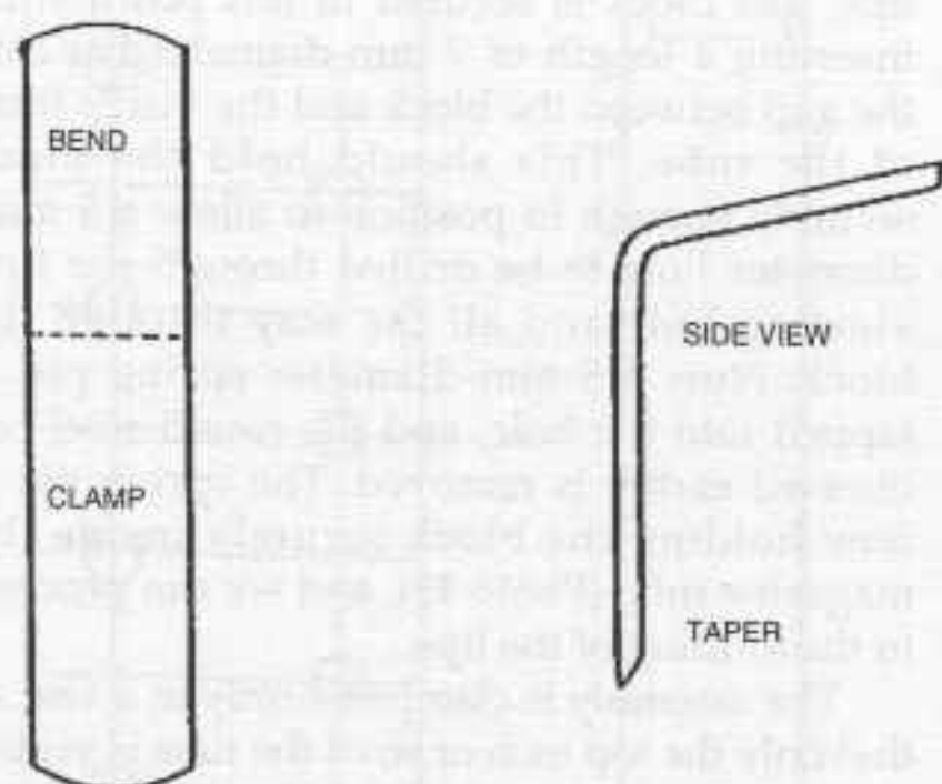
FIGURE CC FOLLOWER CONTOURS
