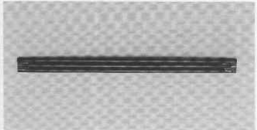
PHOTO 50: The magazine spring winding mandrel, made from three rods brazed together.
