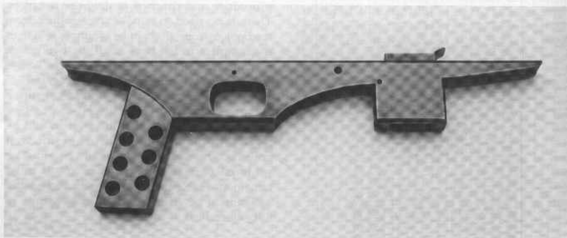
PHOTO 39: Side view of lower receiver with grip and well in position.
