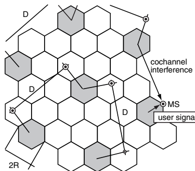
Figure 4.3: Cellular Architecture—Details
