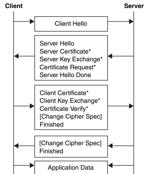
Figure 6.9: TLS in WAP
