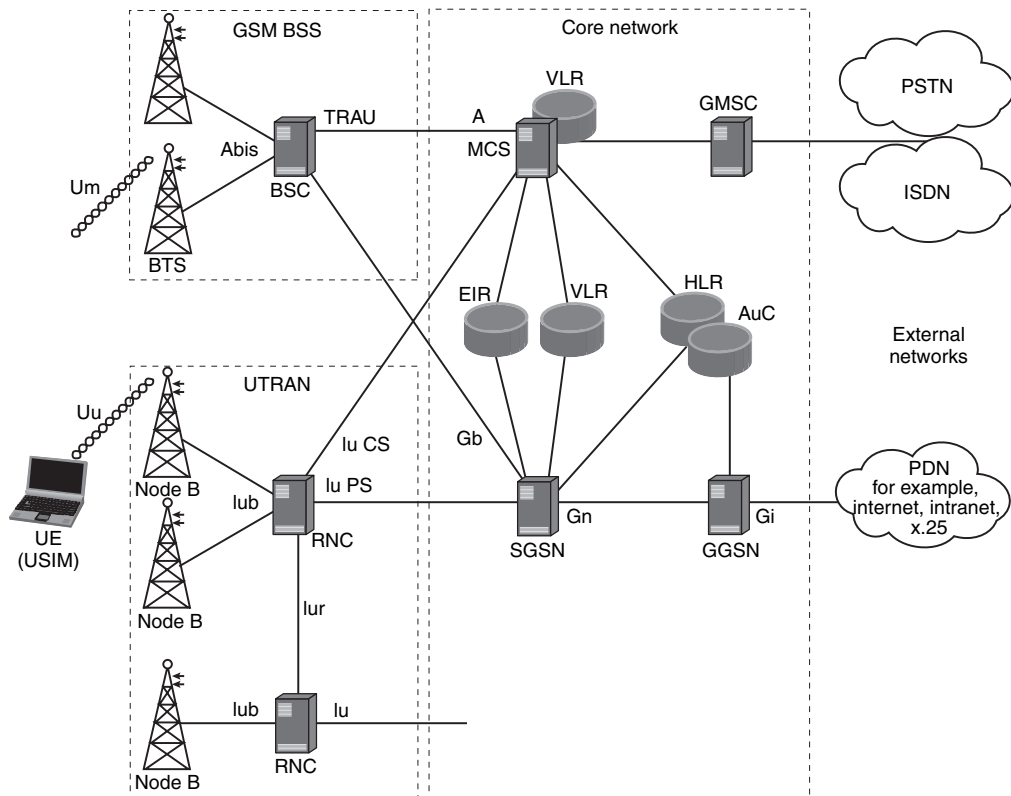
Figure 4.7: UMTS Architecture
