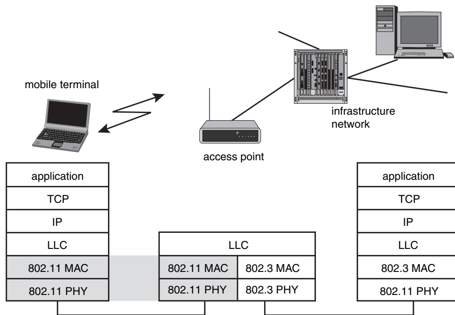
Figure 5.5a: 802.11 System Architecture
