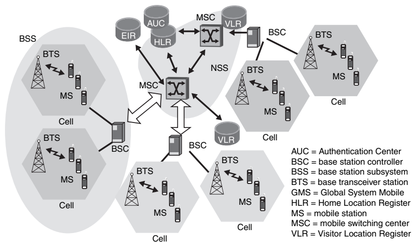
Figure 4.6b: GSM Architecture—Details
