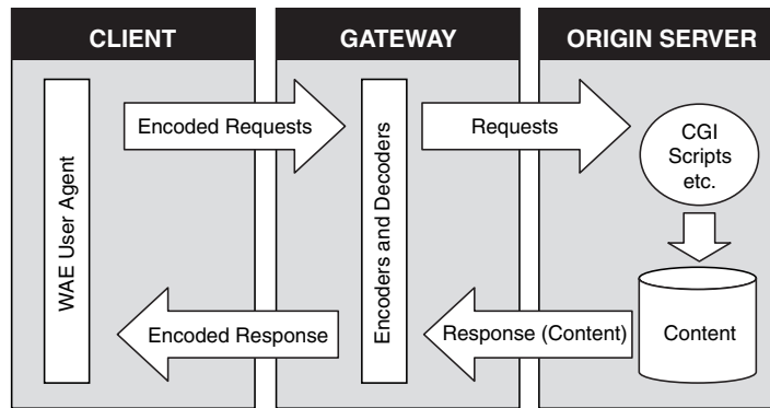
Figure 6.8: WAP—Overview
