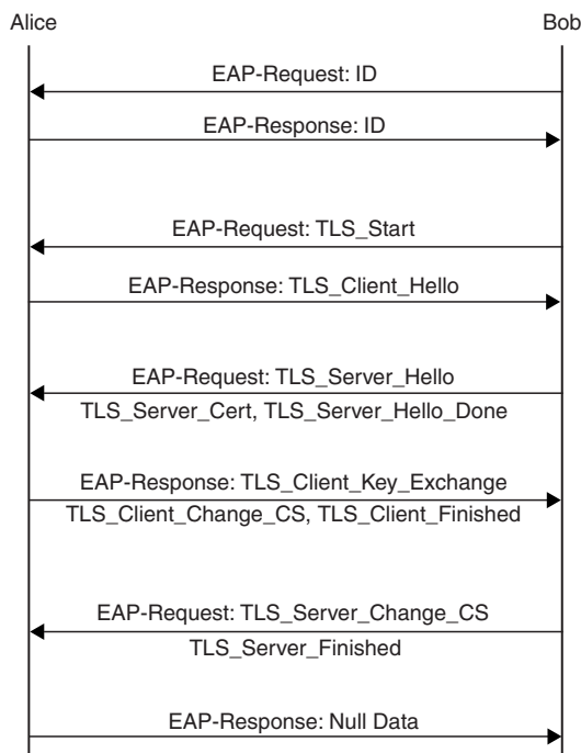
Figure 3.6: EAP-TLS
