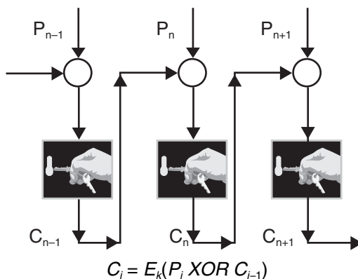
Figure 1.13: CBC Mode
