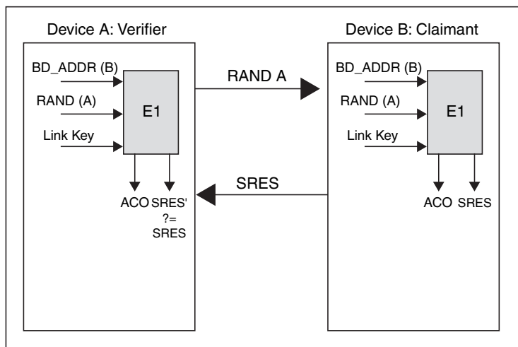
Figure 8.6: Bluetooth Authentication
