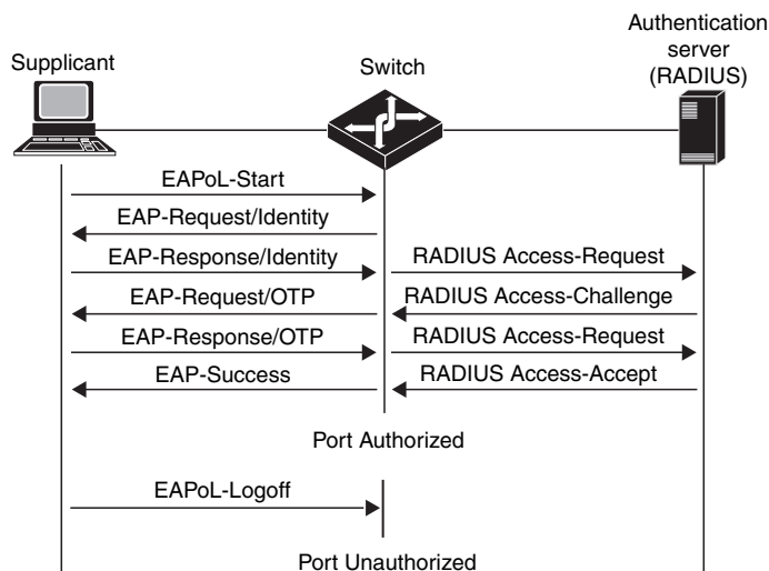
Figure 7.10b: EAPoL
