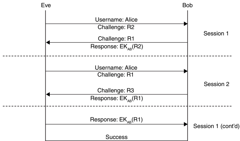
Figure 2.11: Reflection Attack
