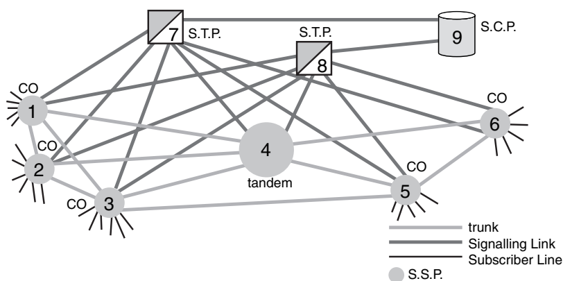
Figure 4.4b: SS7 and the PSTN
