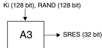
Figure 6.3: GSM SRES Generation
