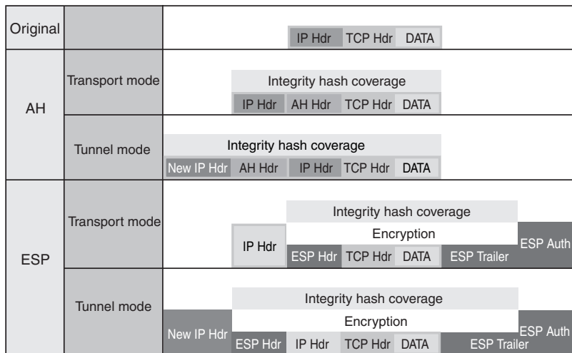
Figure 3.8b: Encapsulation in Different IPSec Modes
