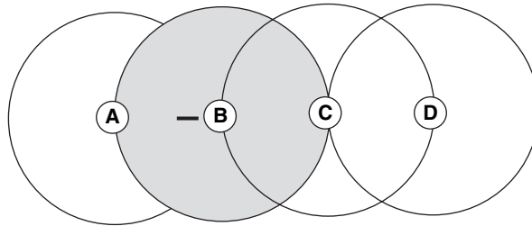
Figure 4.1c: Exposed Node Problem
