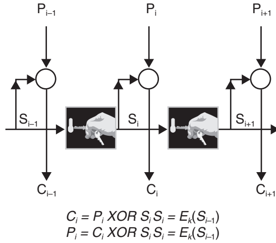
Figure 1.14: OFB Mode
