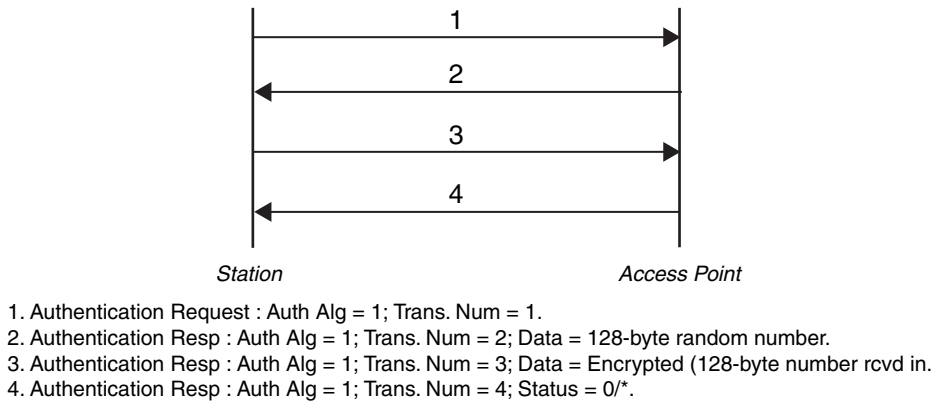
Figure 7.3: 802.11 SKA
