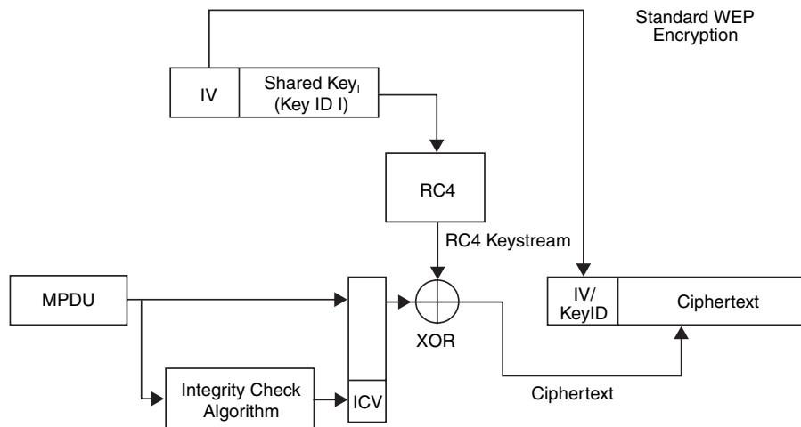
Figure 7.5: WEP
