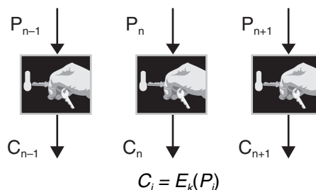
Figure 1.12: ECB Mode
