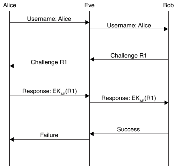
Figure 2.14: Session Hijacking
