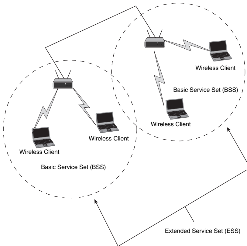
Figure 5.4: 802.11 System Overview
