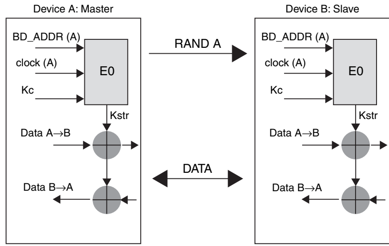
Figure 8.9: Bluetooth Encryption
