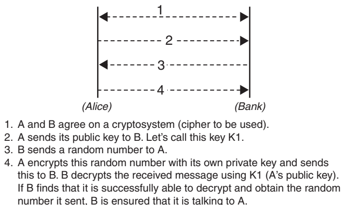
Figure 1.11: Challenge-Response
