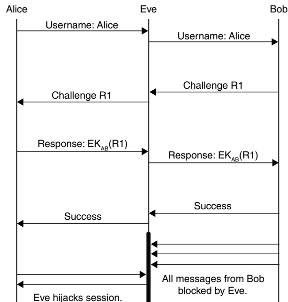
Figure 2.15: Session Hijacking—Variation
