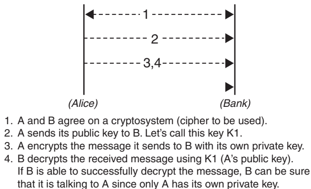
Figure 1.10: Digital Signatures
