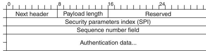
Figure 3.7a: Authentication Header for IPSec
