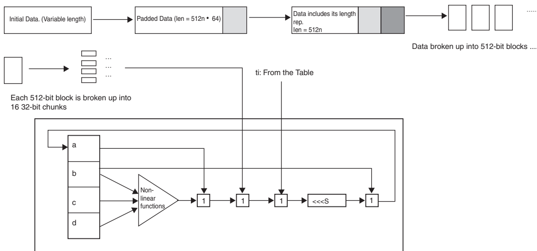
Figure 2.26: MD5
