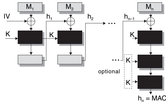
Figure 7.12: AES CBC-MAC
