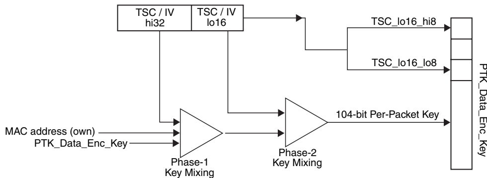
Figure 7.9: TKIP Encryption
