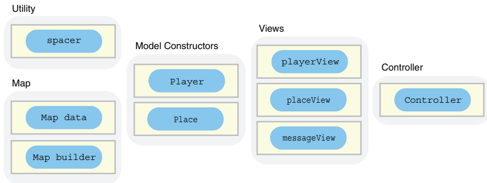
Figure 16.7 The many modules of The Crypt
