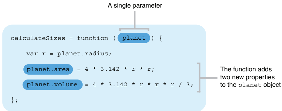
Figure 7.3 The calculateSizes function adds new properties to the planet object.
