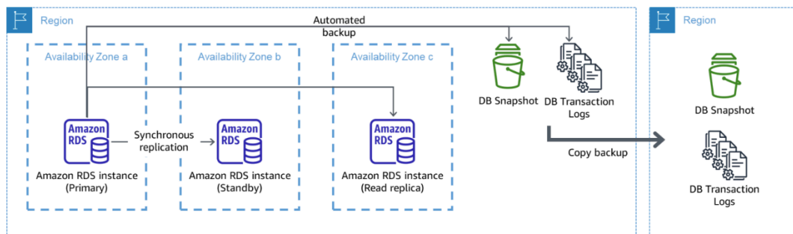
Figure 10: A resilient multi-AZ database deployment with backup to another AWS Region
