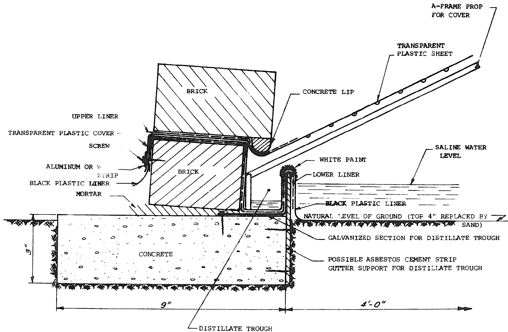
FIG No. 3 - CROSS SECTION OF SIDE WALL OF SOLAR STILL
