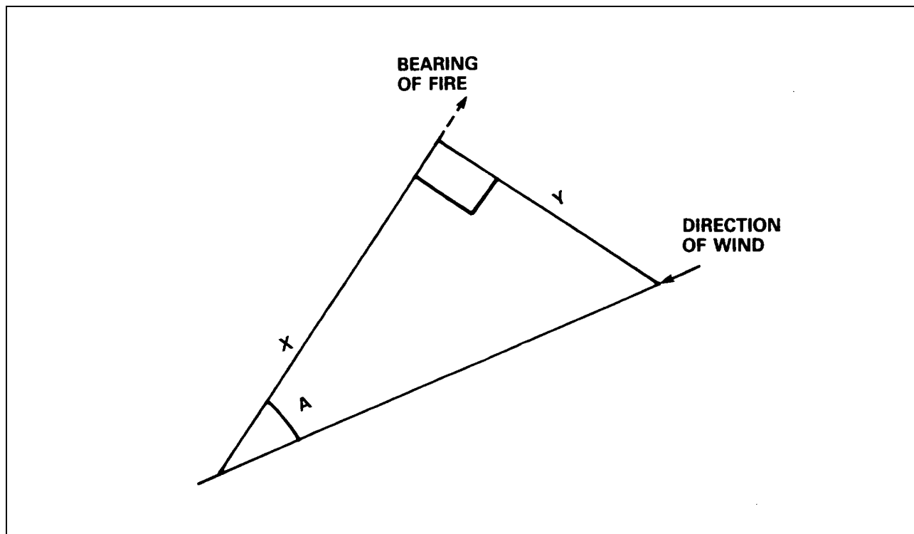
Figure 8-2-1 Determining Components of a 1 Knot Wind
