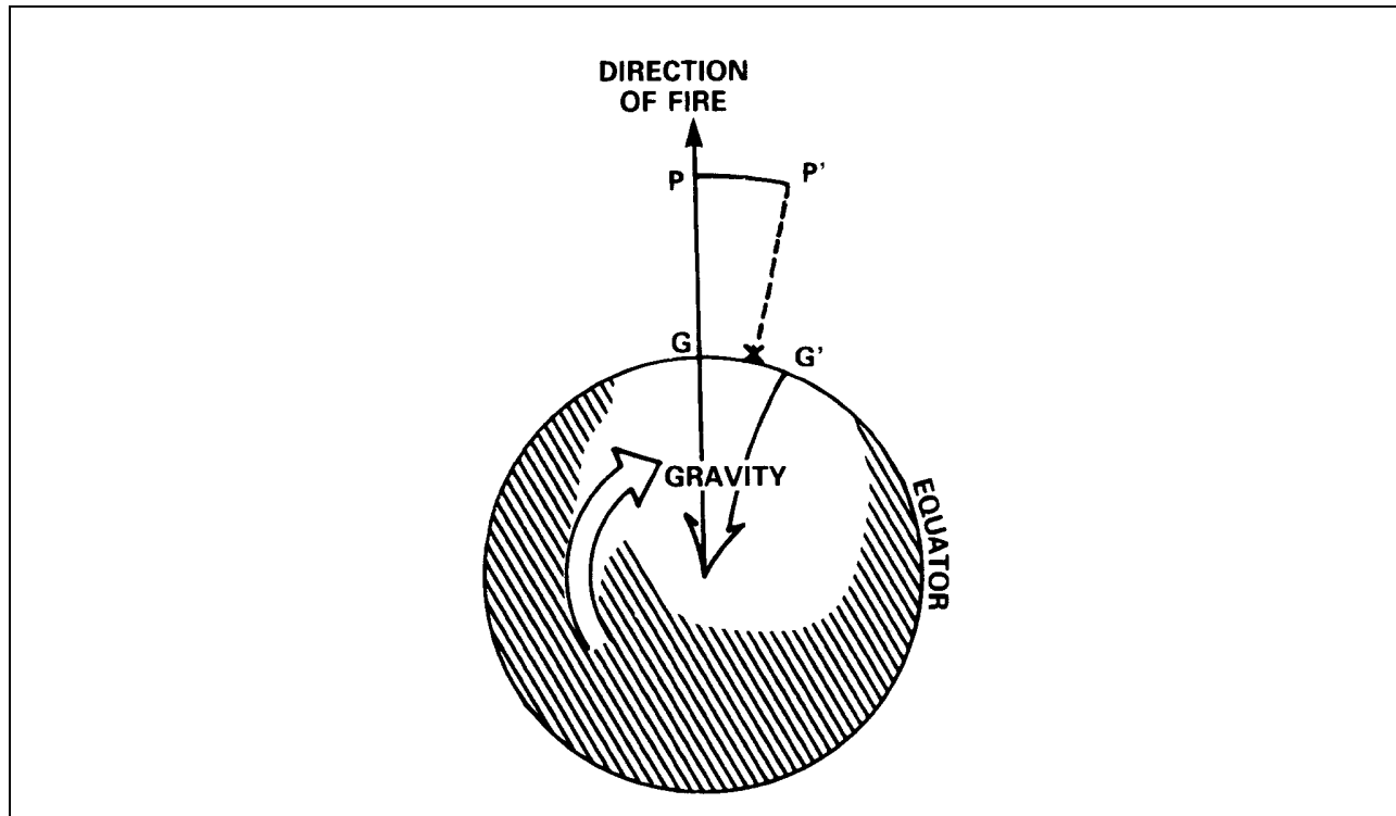
Figure 3-5-2 Projectile Lag
