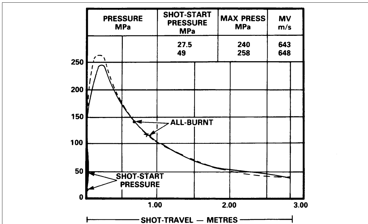
Figure 2-3-9 Variation in Shot-Start Pressure
