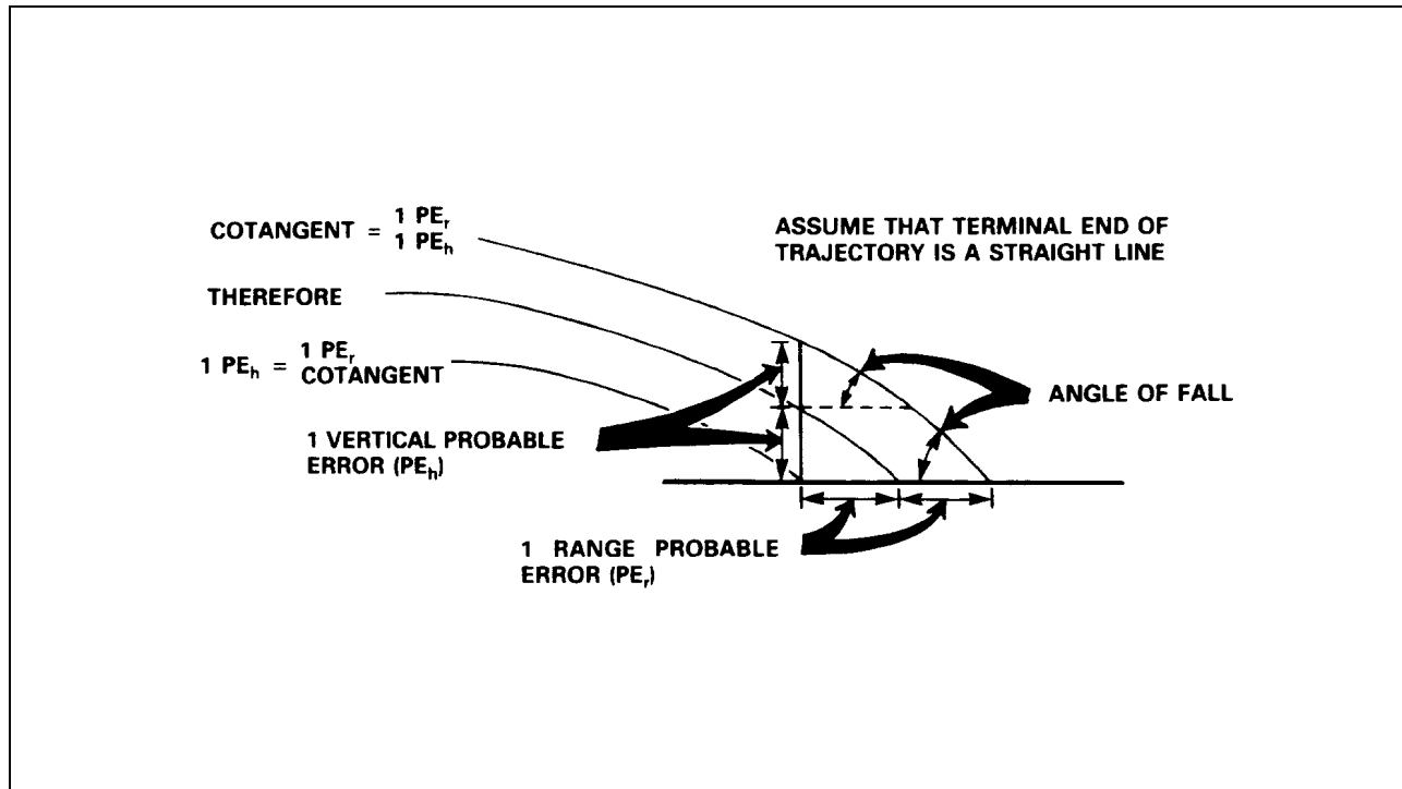
Figure 7-3-7 Vertical Dispersion
