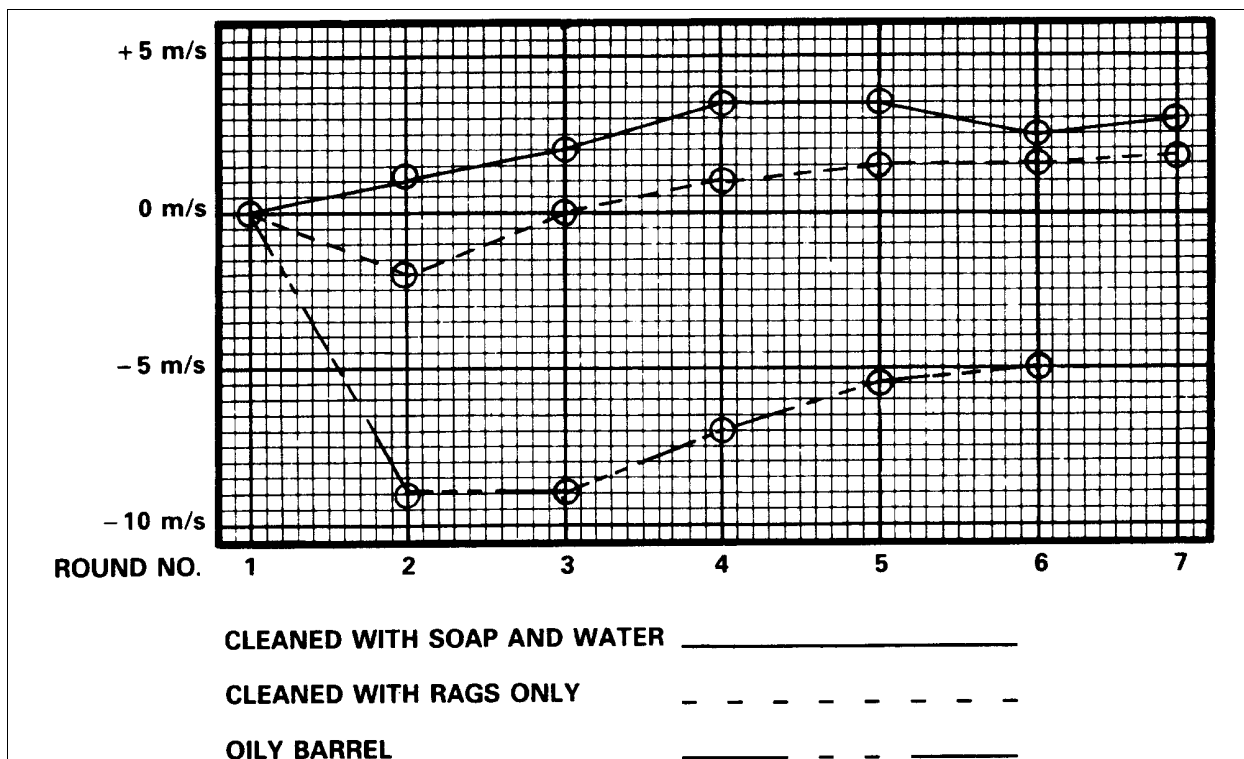
Figure 2-4-1 Velocity Trends - 105 mm Howitzer
