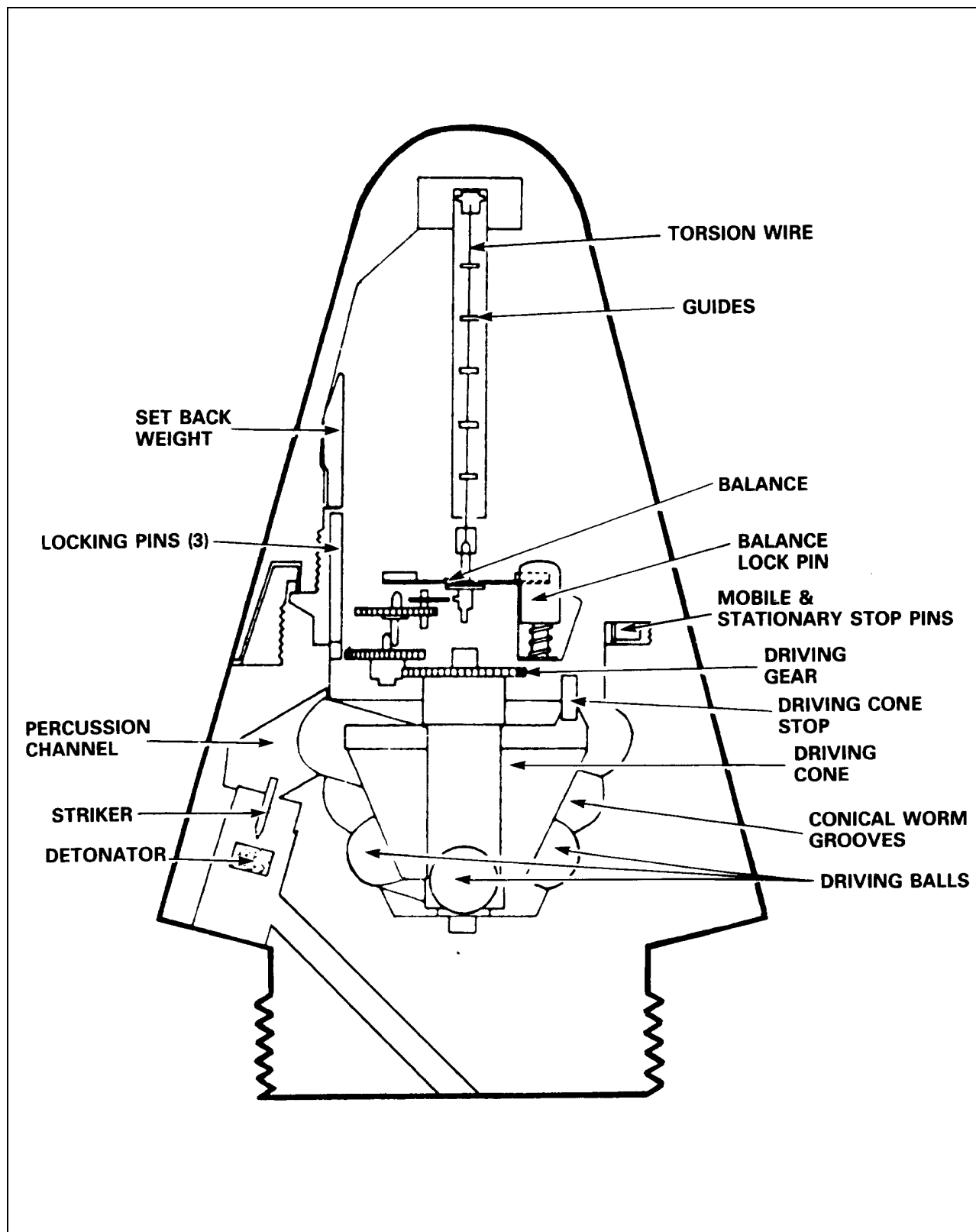
Figure 9-7-8 The Dixi Time Mechanism (Swiss)
