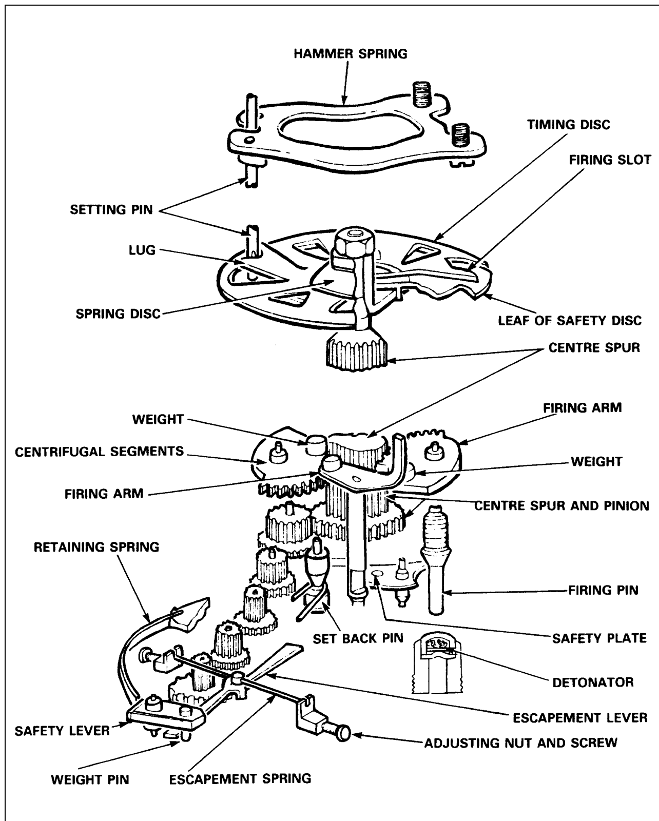
Figure 9-7-7 The Junghans Time Mechanism (US)
