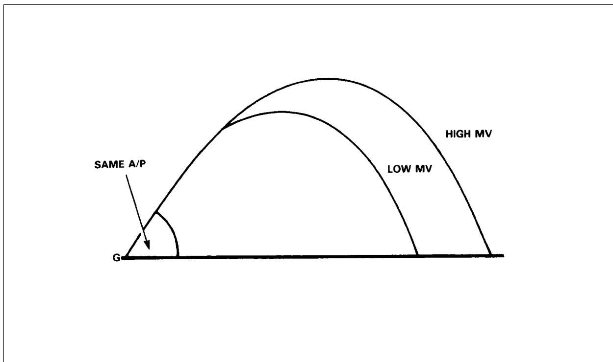
Figure 6-1-8 Variation Due to Change in Muzzle Velocity (High Angle) (Elevation View)
