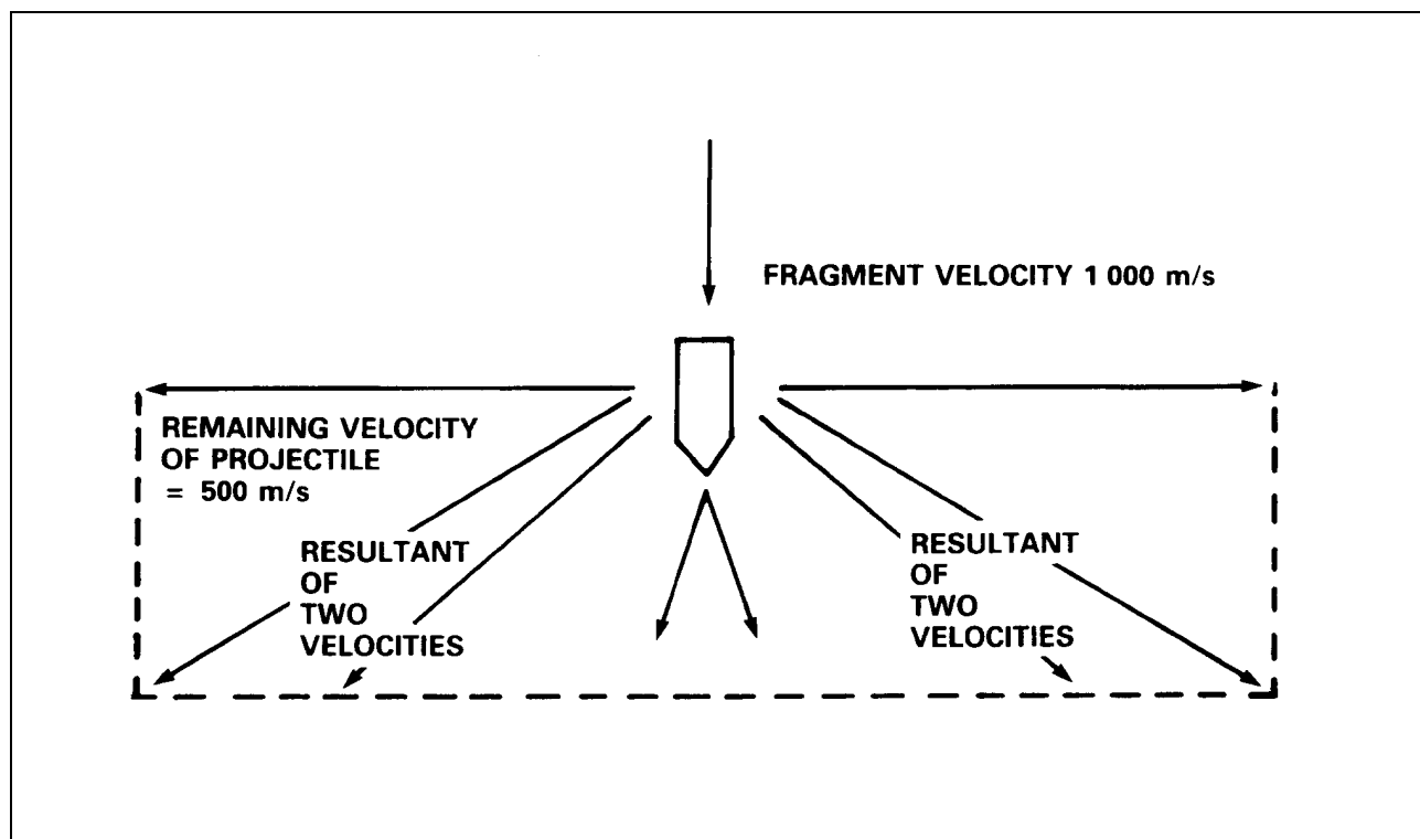
Figure 4-2-3 Detonation of a Projectile in Flight
