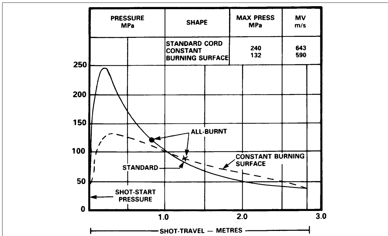
Figure 2-3-6 Variation in Propellant Shape
