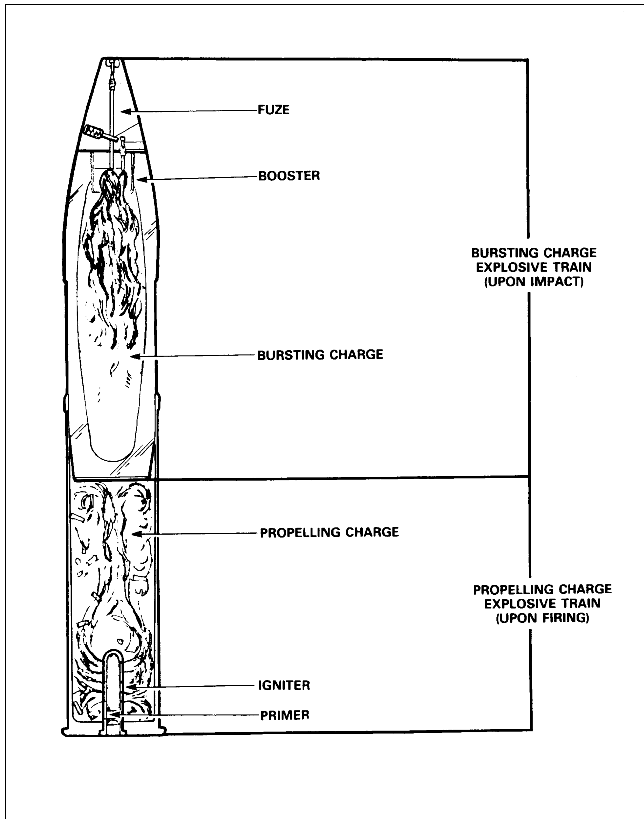
Figure 9-3-2 Propelling Charge and Bursting Charge Explosive Train
