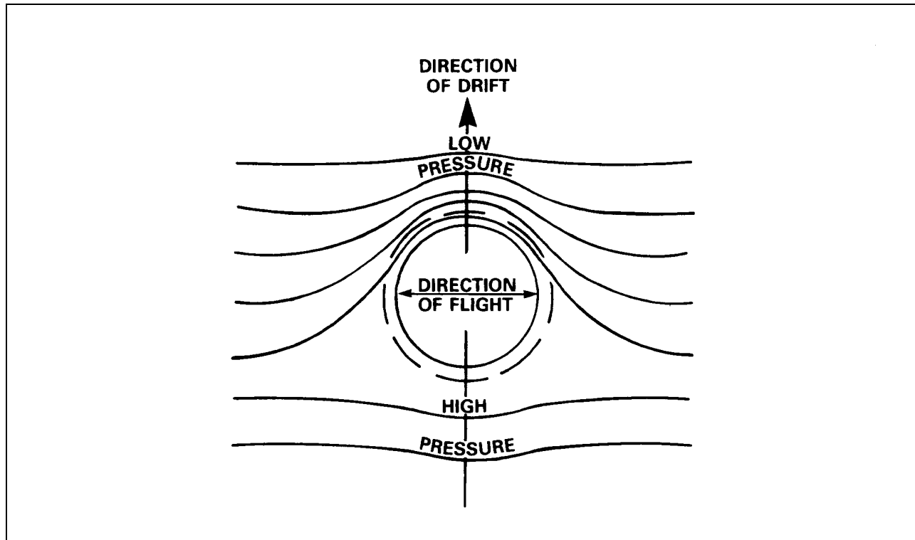
Figure 3-4-8 Magnus Effect
