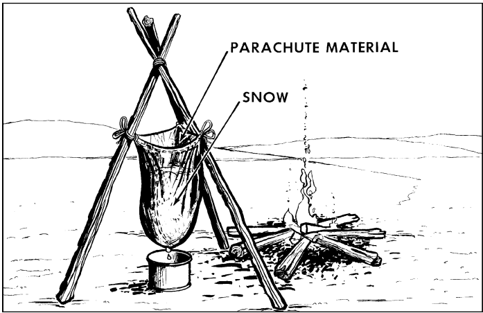
Figure VII-3. Water Generator
