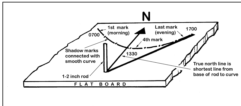
Figure II-3. Pocket Navigator
