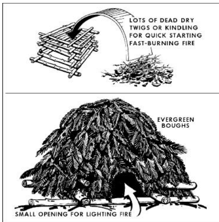
Figure III-5. Smoke Generator
