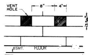
AIR VENT DETAIL
