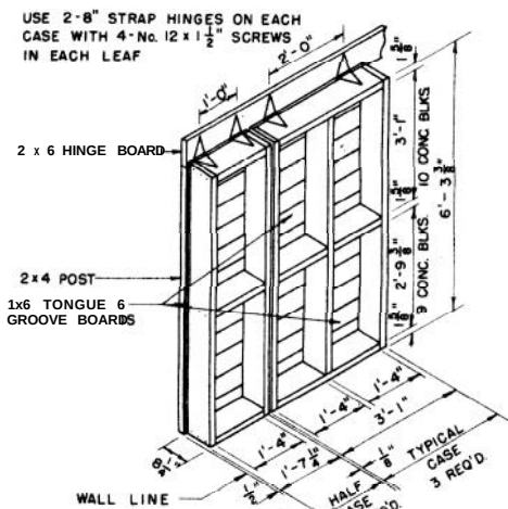
ISOMETRIC OF CASES
