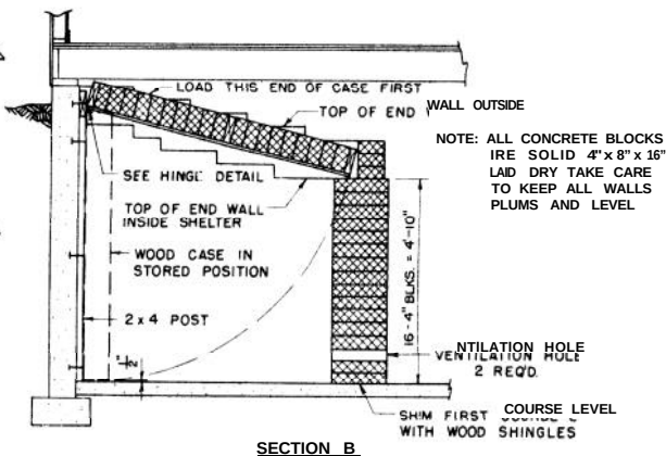
SECTION B
