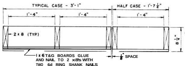
DETAIL SECTIONS
