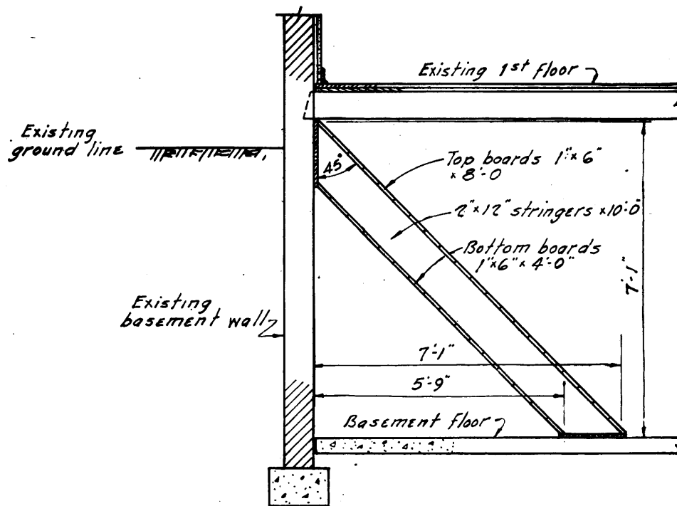
SECTION
