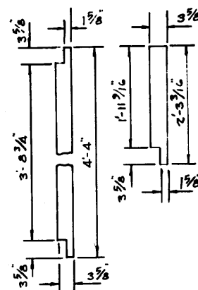
STIFFENER DETAILS
