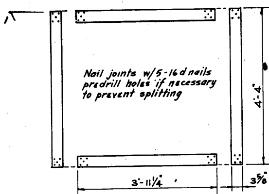
FRAME DETAIL
