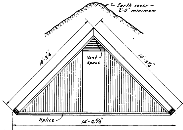
FRONT ELEVATION
