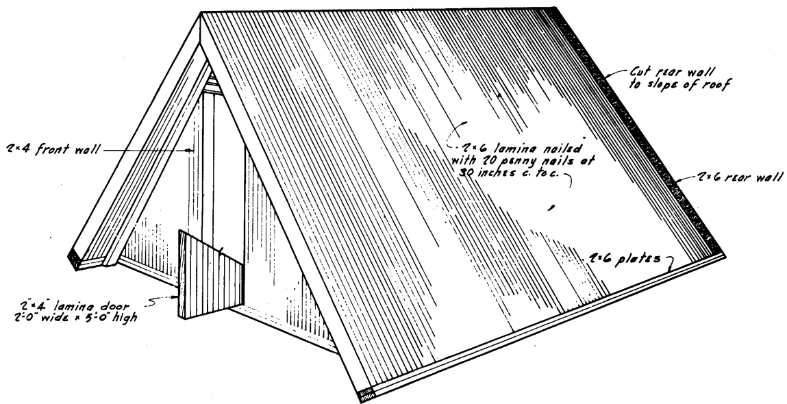
PERSPECTIVE VIEW
