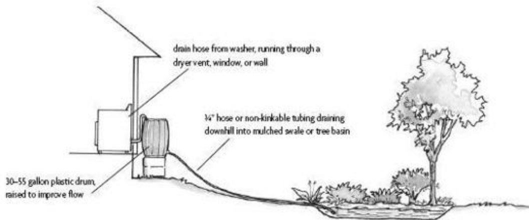
A washing machine set up to pump graywater into a drum that will then drain to a planted, mulched swale or tree. REDRAWN WITH PERMISSION FROM CREATE AN OASIS WITH GREYWATER , BY ART LUDWIG (OASIS DESIGN 2000).
