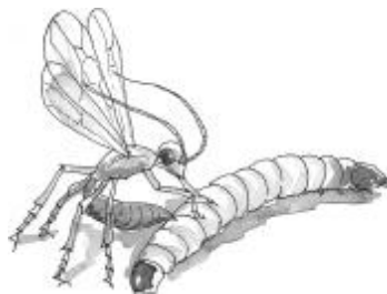
A parasitic braconid wasp injecting eggs into a cabbageworm larva.
