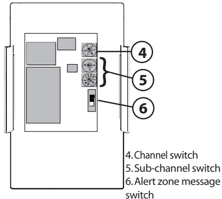
Figure 4 Radio Transmitter Module
