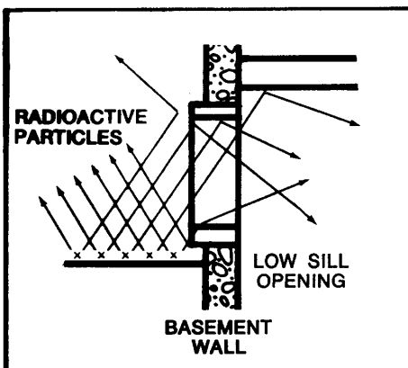
GEOMETRY SHIELDING BY LOCATION OF WINDOWS
