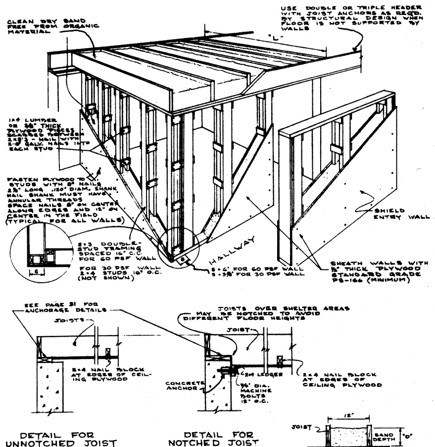
CEILING DETAILS
