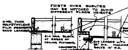
DETAIL FOR UNNOTCHED JOIST
